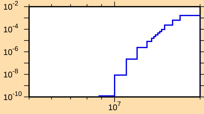
\sigma vs. E for ^{234}\text{Pa}(n,np)
