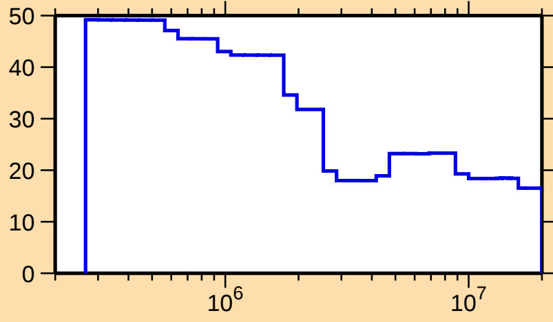
\Delta\sigma/\sigma vs. E for ^{234}\text{Pa}(n,n\text{onel.})
