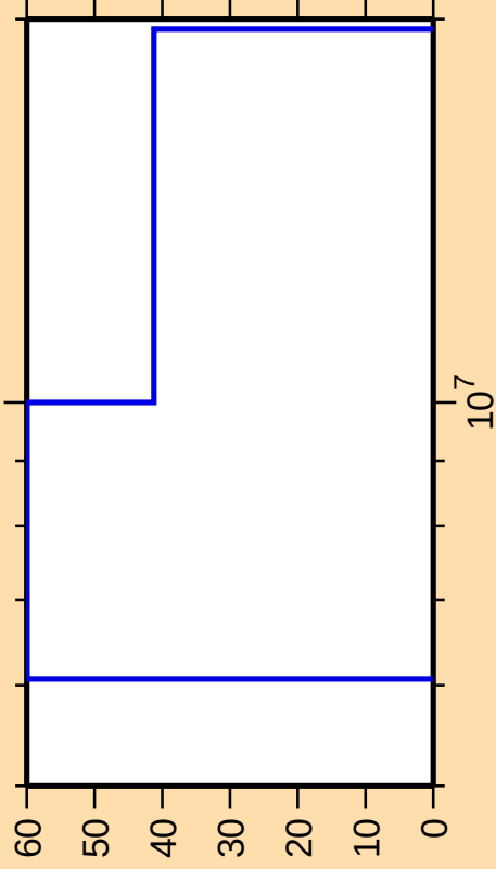
\Delta\sigma/\sigma vs. E for ^{234}\text{Pa}(n,d)
