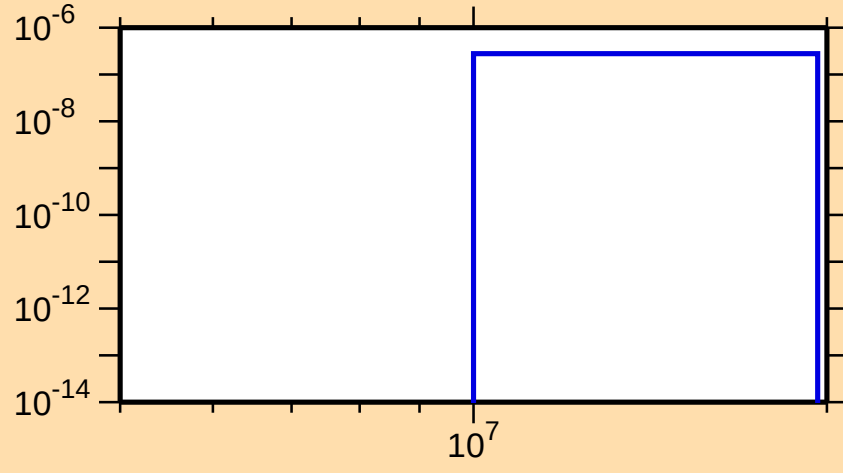
\sigma vs. E for ^{234}\text{Pa}(n,\text{nd})
