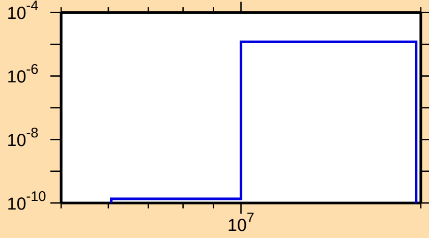
\sigma vs. E for ^{234}\text{Pa}(n,n\alpha)
