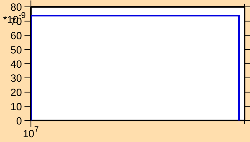
\sigma vs. E for ^{234}\text{Pa}(n,nt)
