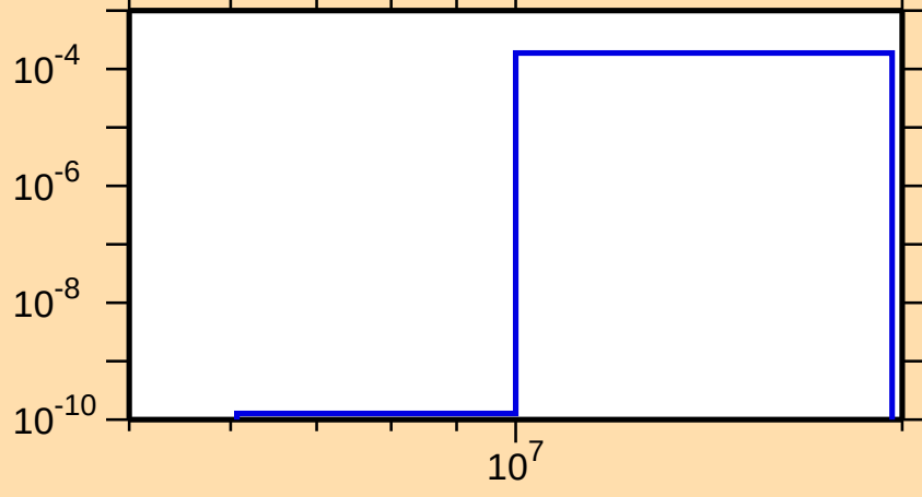
\sigma vs. E for ^{234}\text{Pa}(n,d)
