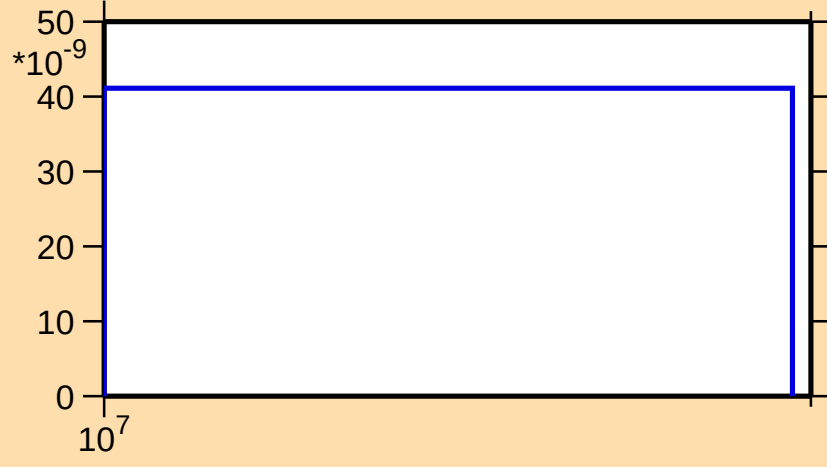
\sigma vs. E for ^{234}\text{Pa}(n,2np)
