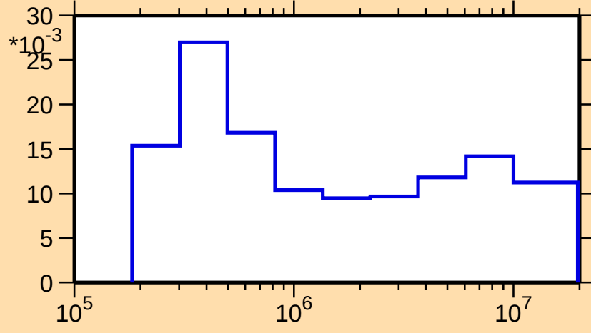
\sigma vs. E for ^{234}\text{Pa}(n,n_3)
