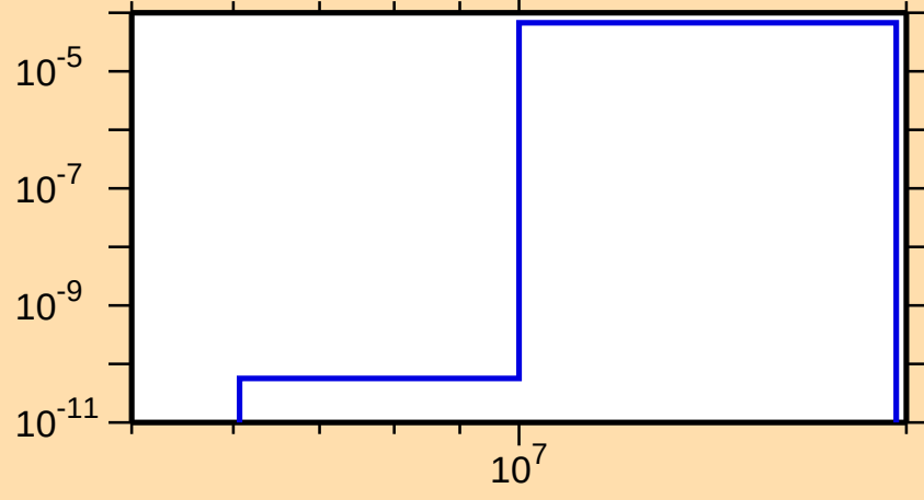
\sigma vs. E for ^{234}\text{Pa}(n,t)
