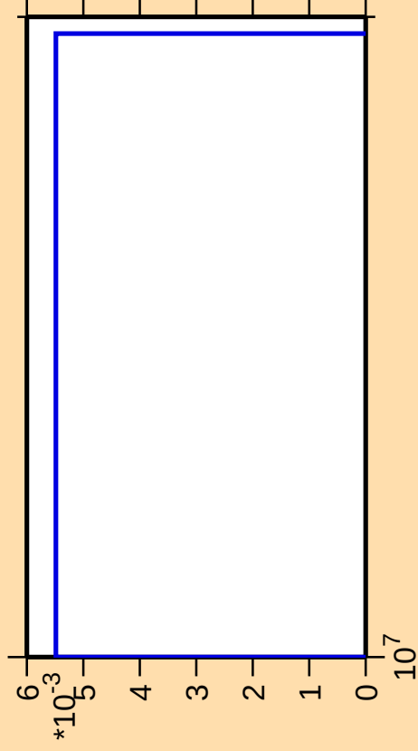
\Delta\sigma/\sigma vs. E for ^{234}\text{Pa} (mt 11)
