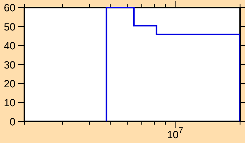
\Delta\sigma/\sigma vs. E for ^{234}\text{Pa}(n,2n)
