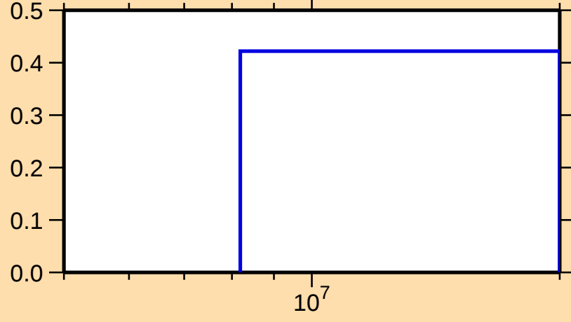
\sigma vs. E for ^{234}\text{Pa}(n,3n)
