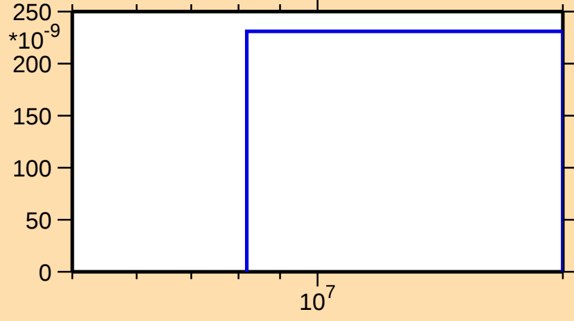
\sigma vs. E for ^{234}\text{Pa}(n,\text{nd})
