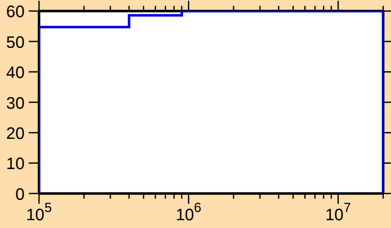
\Delta\sigma/\sigma vs. E for ^{234}\text{Pa}(n,f)
