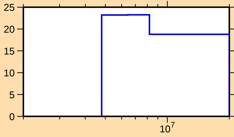
\Delta\sigma/\sigma vs. E for ^{234}\text{Pa}(n,\text{nonel.})
