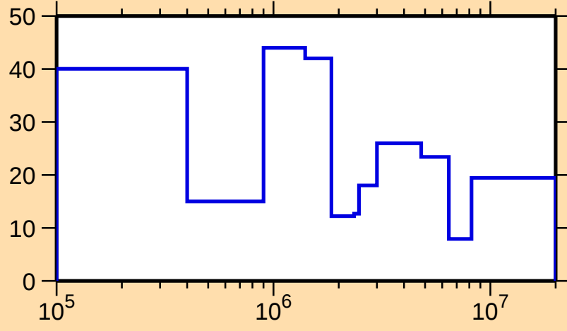
\Delta\sigma/\sigma vs. E for ^{234}\text{Pa}(n,\text{el.})
