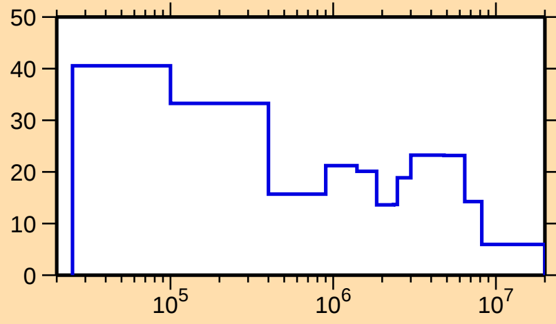
\Delta\sigma/\sigma vs. E for ^{234}\text{Pa}(n,\text{tot.})
