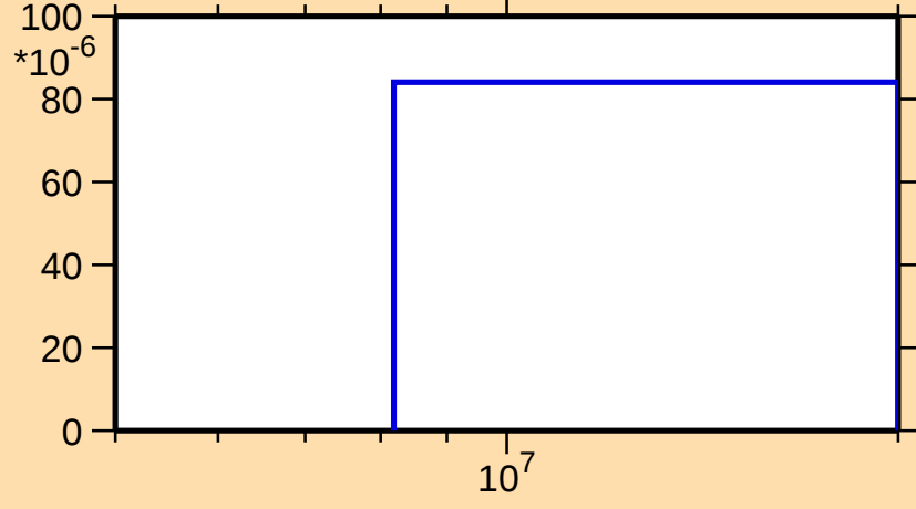
\sigma vs. E for ^{234}\text{Pa}(n,np)
