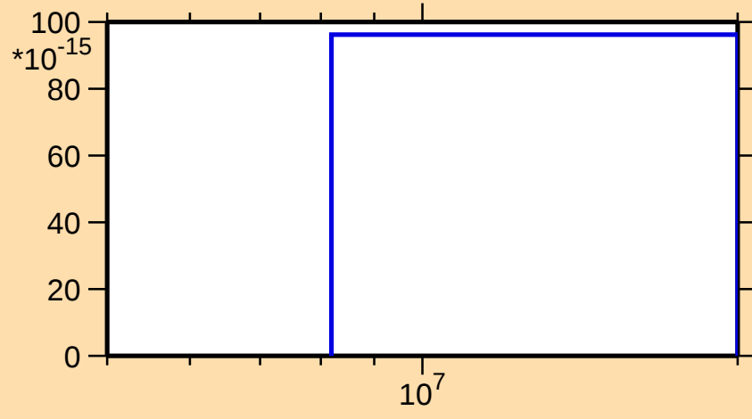
\sigma vs. E for ^{234}\text{Pa}(n,\text{He}3)
