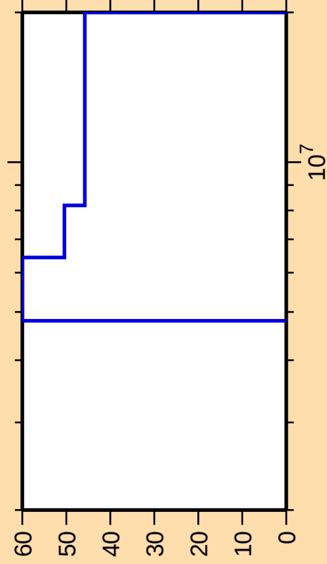
\Delta\sigma/\sigma vs. E for ^{234}\text{Pa}(n,2n)
