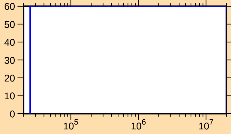
\Delta\sigma/\sigma vs. E for ^{234}\text{Pa}(n,n_1)
