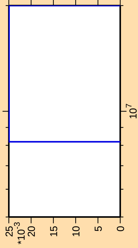
\Delta\sigma/\sigma vs. E for ^{234}\text{Pa}(n,3n\alpha)
