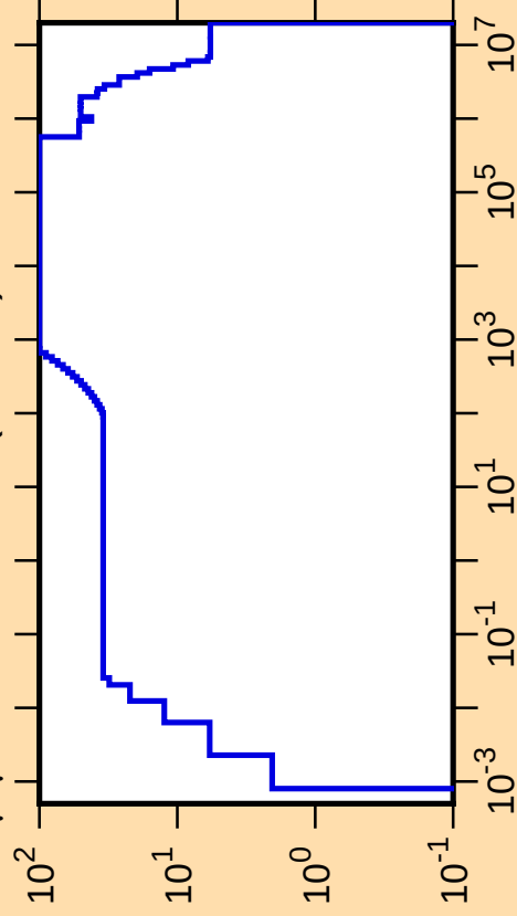
\Delta\mu/\mu vs. E for ^{236}\text{Pa}(\text{mt251})
