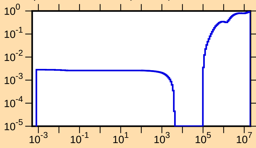
\mu vs. E for ^{236}\text{Pa}(\text{mt251})
