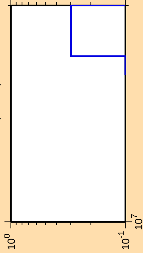
\Delta\sigma/\sigma vs. E for ^{236}\text{Pa}(\text{mt } 42)
