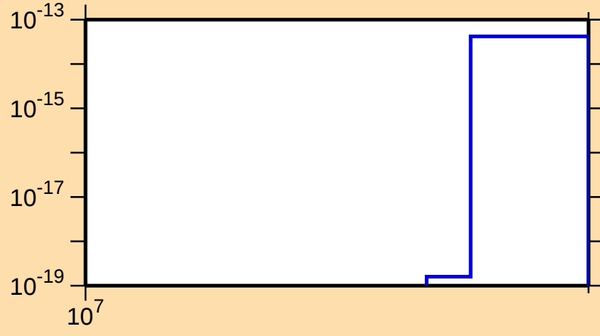
\sigma vs. E for ^{236}\text{Pa}(\text{mt } 42)
