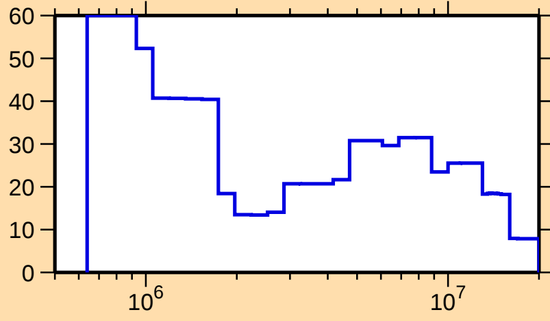
\Delta\sigma/\sigma vs. E for ^{236}\text{Pa}(n,\text{el.})
