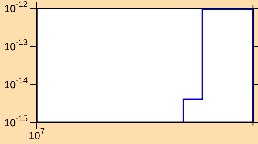
\sigma vs. E for ^{236}\text{Pa}(n,3n\alpha)
