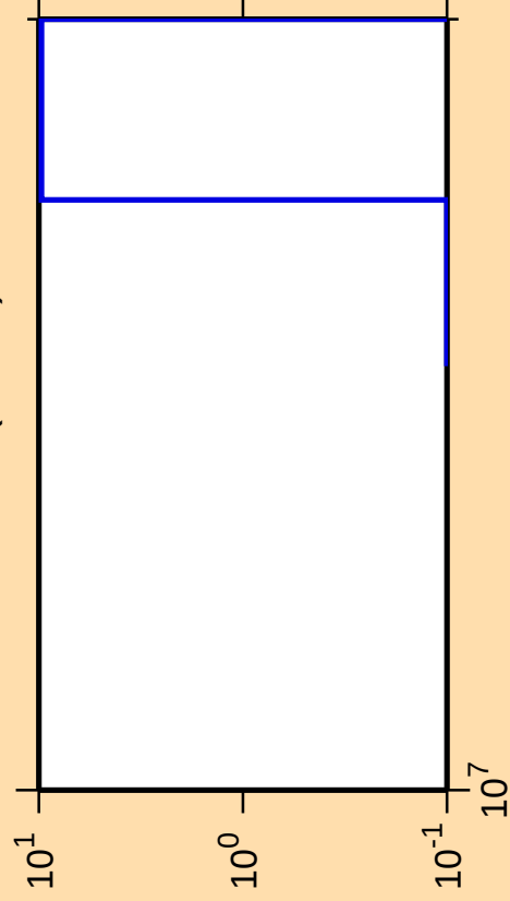
\Delta\sigma/\sigma vs. E for ^{236}\text{Pa}(\text{mt 11})
