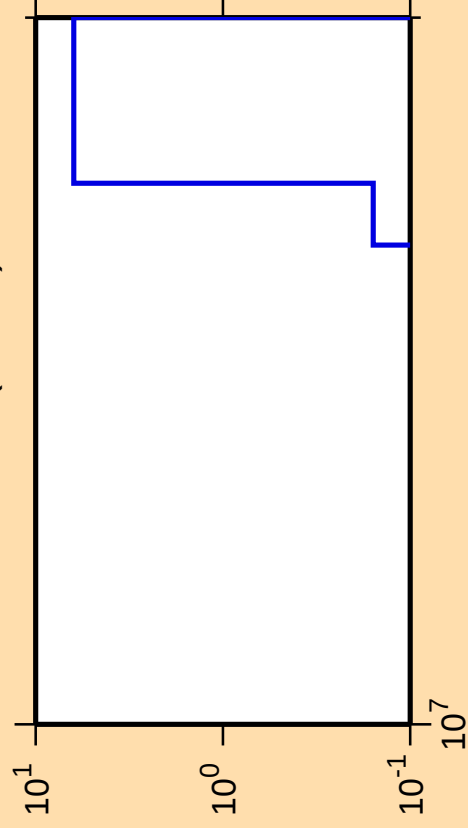
\Delta\sigma/\sigma vs. E for ^{236}\text{Pa}(n,\text{He3})
