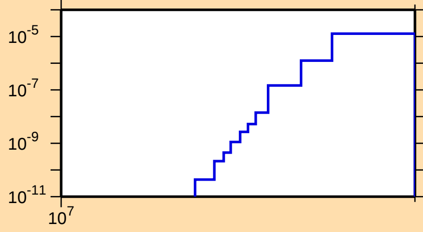
\sigma vs. E for ^{236}\text{Pa}(n,\text{nd})
