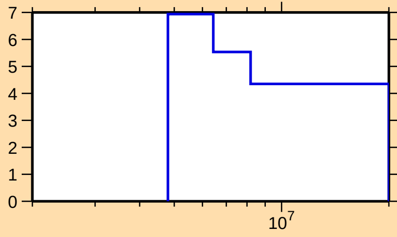
\Delta\sigma/\sigma vs. E for ^{236}\text{Pa}(n,\text{nonel.})
