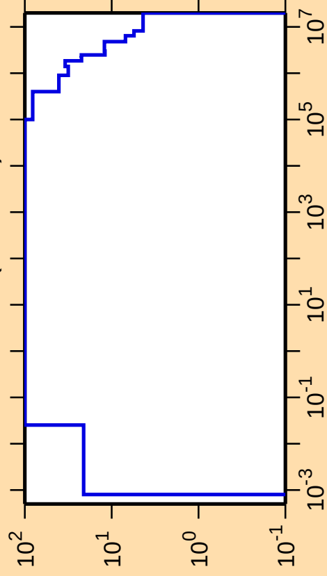
\Delta\sigma/\sigma vs. E for ^{236}\text{Pa}(n,\text{nonel.})
