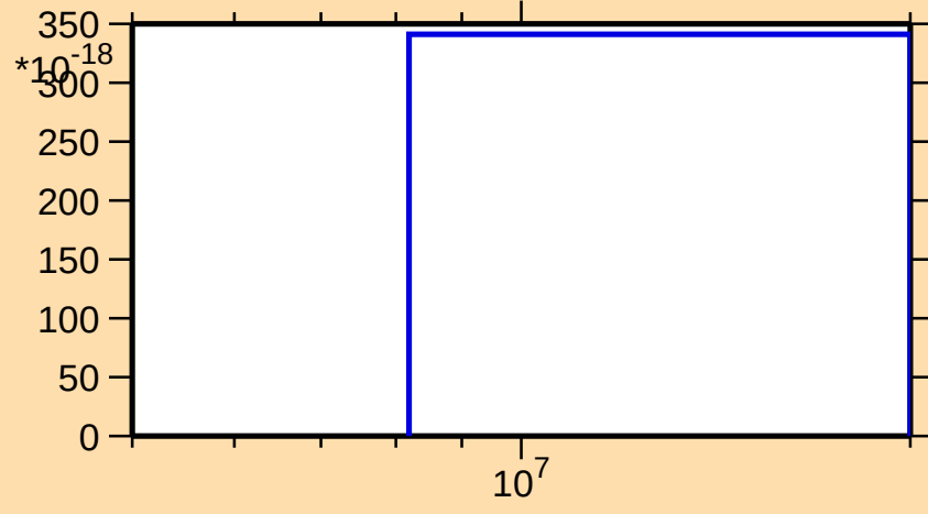
\sigma vs. E for ^{236}\text{Pa}(\text{mt } 42)
