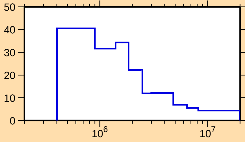
\Delta\sigma/\sigma vs. E for ^{236}\text{Pa}(n,n\text{onel.})
