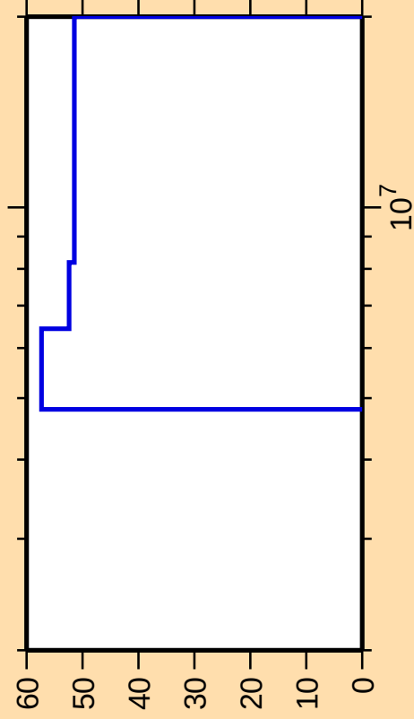
\Delta\sigma/\sigma vs. E for ^{236}\text{Pa}(n,2n)
