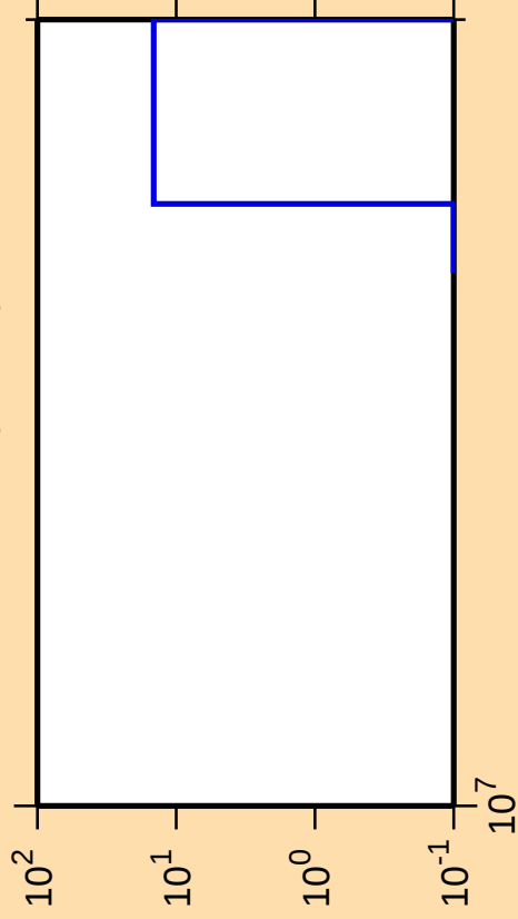
\Delta\sigma/\sigma vs. E for ^{237}\text{Pa} (mt 11)
