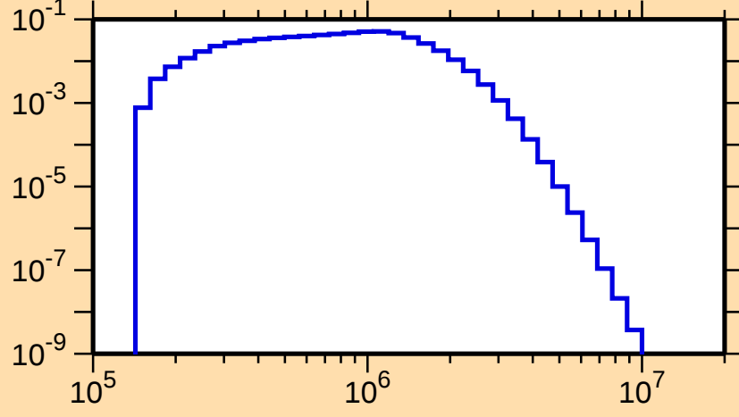
\sigma vs. E for ^{237}\text{Pa}(n,n_4)
