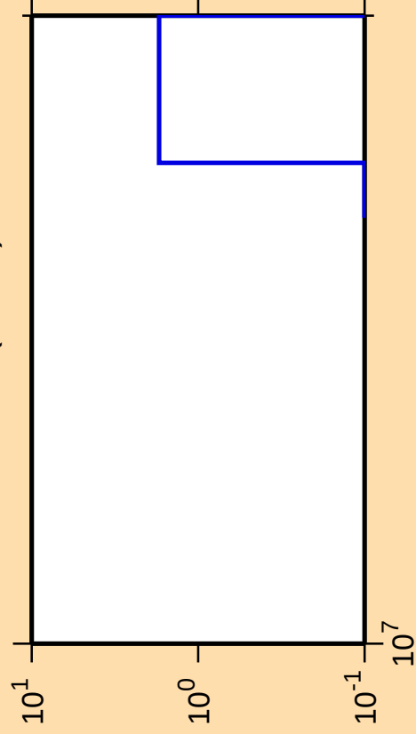
\Delta\sigma/\sigma vs. E for ^{237}\text{Pa} (mt 42)
