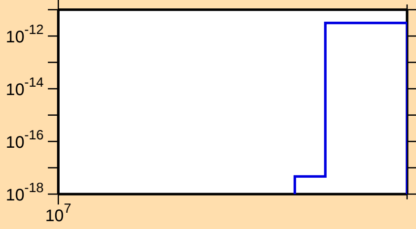
\sigma vs. E for ^{237}\text{Pa} (mt 11)
