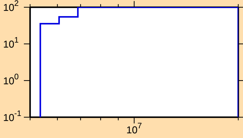
\Delta\sigma/\sigma vs. E for ^{237}\text{Pa}(n,\text{inel.})
