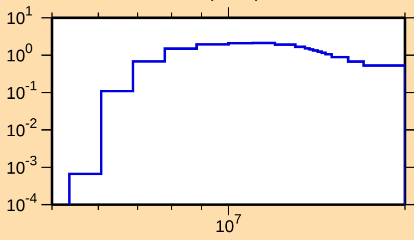
\sigma vs. E for ^{237}\text{Pa}(n,2n)
