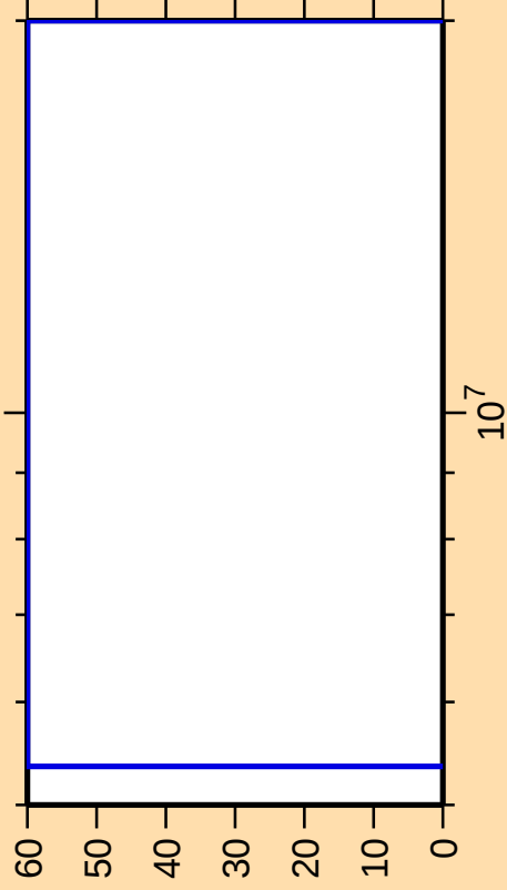
\Delta\sigma/\sigma vs. E for ^{237}\text{Pa}(n,\gamma)
