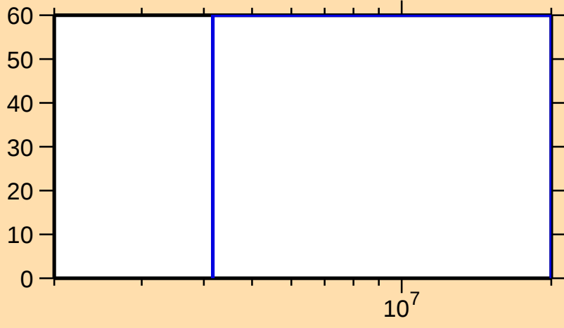
\Delta\sigma/\sigma vs. E for ^{237}\text{Pa}(n,\gamma)
