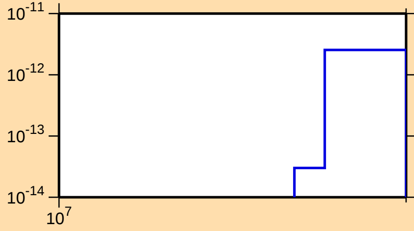
\sigma vs. E for ^{237}\text{Pa}(n,3n\alpha)
