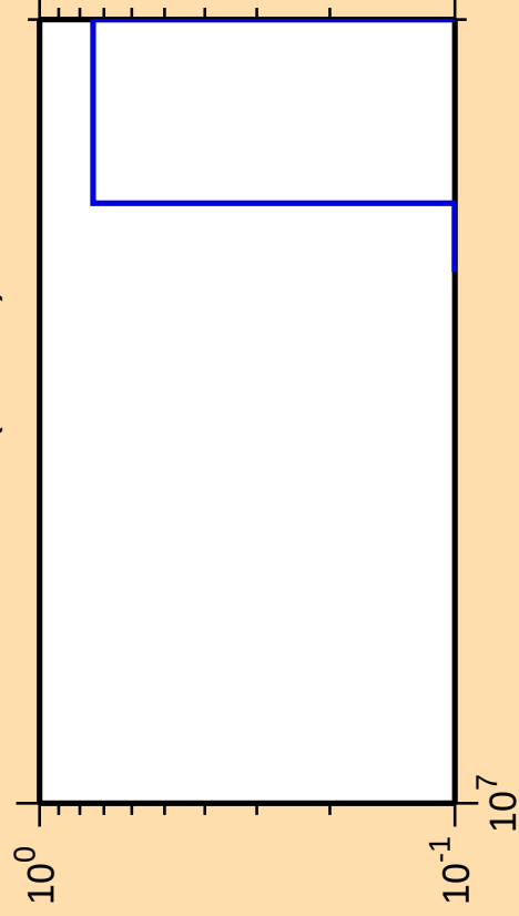
\Delta\sigma/\sigma vs. E for ^{237}\text{Pa}(n,\text{He3})
