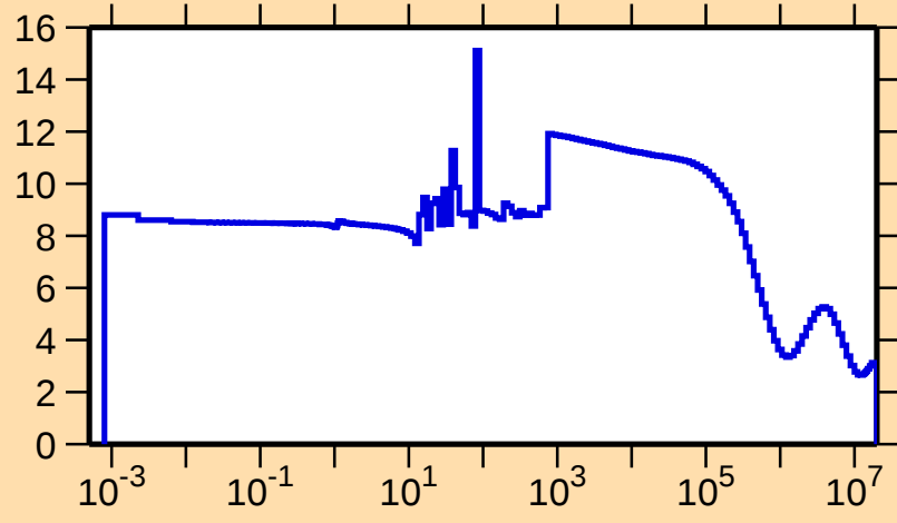
\sigma vs. E for ^{237}\text{Pa}(n,\text{el.})
