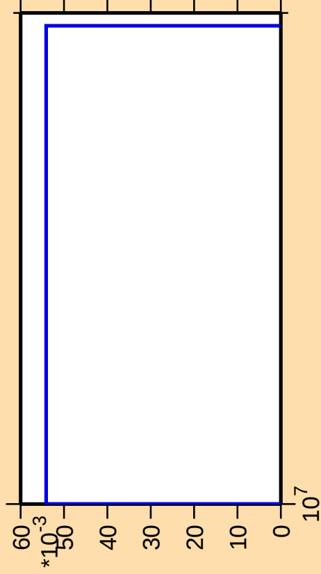
\Delta\sigma/\sigma vs. E for ^{237}\text{Pa}(n,3n\alpha)
