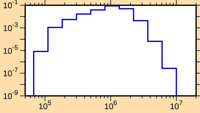
\sigma vs. E for ^{237}\text{Pa}(n,n_3)
