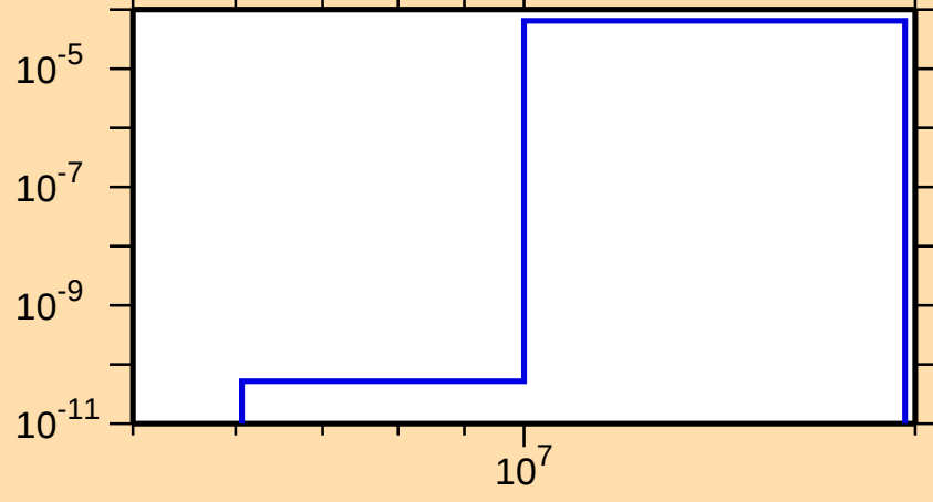
\sigma vs. E for ^{237}\text{Pa}(n,d)
