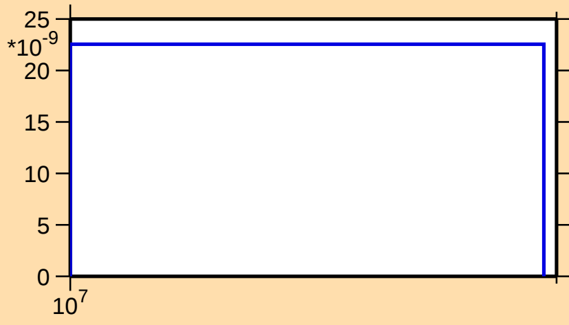
\sigma vs. E for ^{237}\text{Pa}(n,\text{nd})
