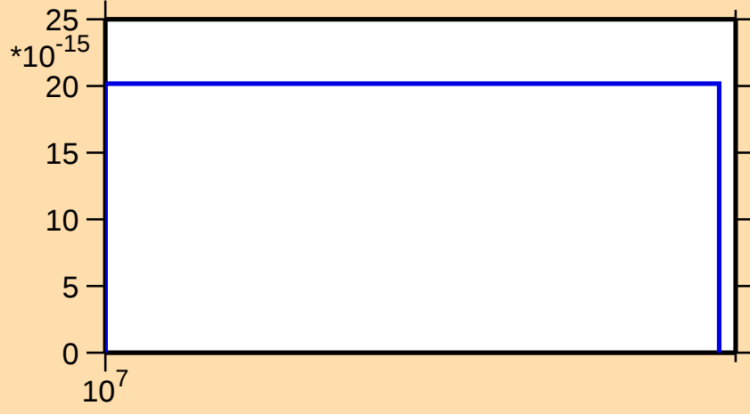
\sigma vs. E for ^{237}\text{Pa}(\text{mt } 11)
