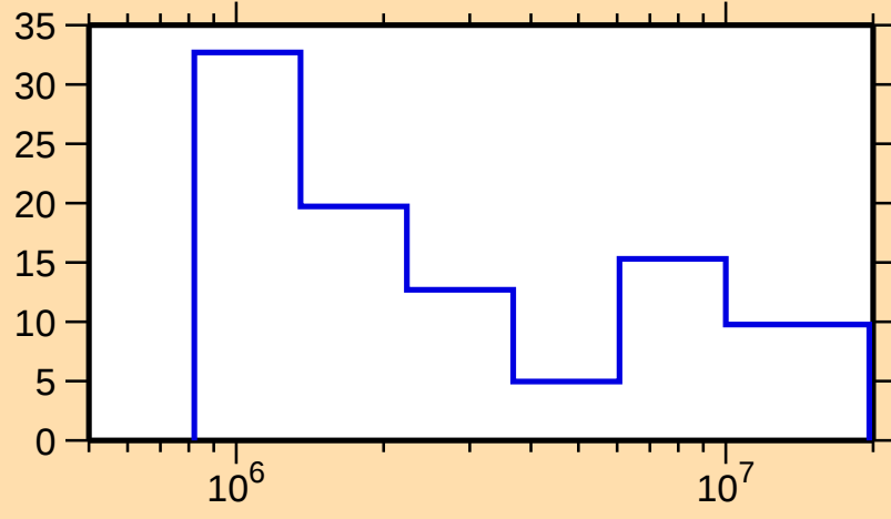
\Delta\sigma/\sigma vs. E for ^{237}\text{Pa}(n,\text{tot.})
