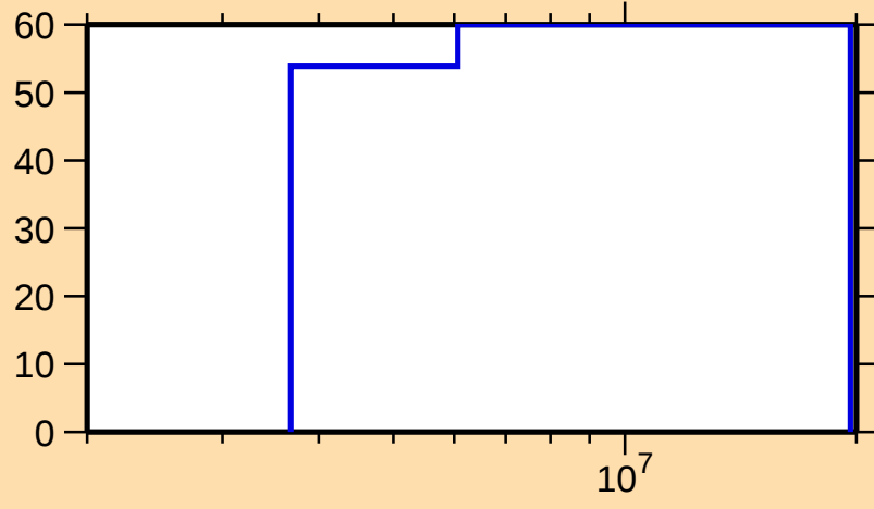
\Delta\sigma/\sigma vs. E for ^{237}\text{Pa}(n,p)
