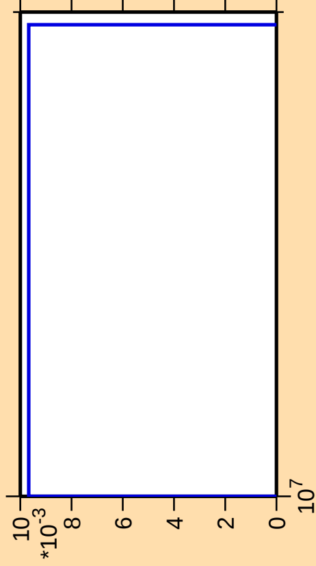
\Delta\sigma/\sigma vs. E for ^{237}\text{Pa} (mt 42)
