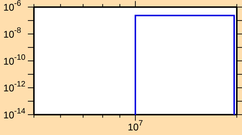
\sigma vs. E for ^{237}\text{Pa}(n,nt)
