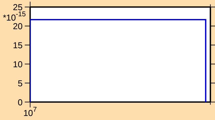
\sigma vs. E for ^{237}\text{Pa}(n,3n\alpha)
