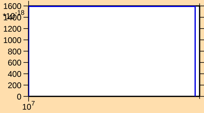
\sigma vs. E for ^{237}\text{Pa} (mt 42)
