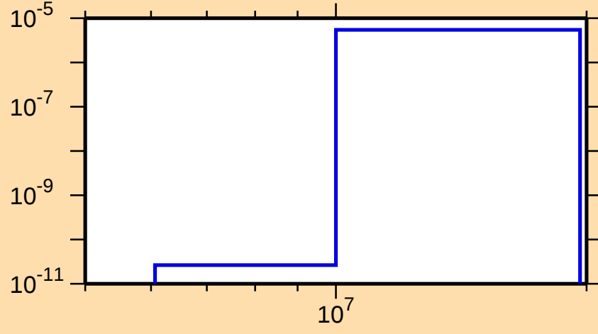
\sigma vs. E for ^{237}\text{Pa}(n,n\alpha)
