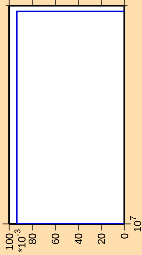
\Delta\sigma/\sigma vs. E for ^{237}\text{Pa}(\text{mt } 11)
