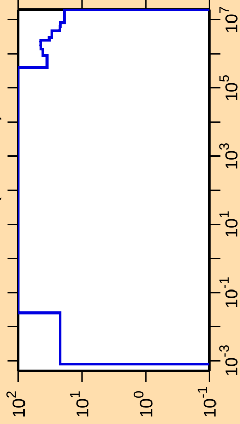
\Delta\sigma/\sigma vs. E for ^{237}\text{Pa}(n,\text{nonel.})
