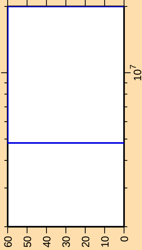
\Delta\sigma/\sigma vs. E for ^{237}\text{Pa}(n,n\text{cont.})
