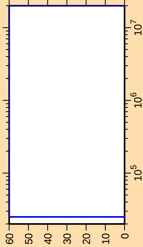
\Delta\sigma/\sigma vs. E for ^{237}\text{Pa}(n,n_1)
