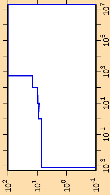
\Delta\sigma/\sigma vs. E for ^{237}\text{Pa}(n,f)
