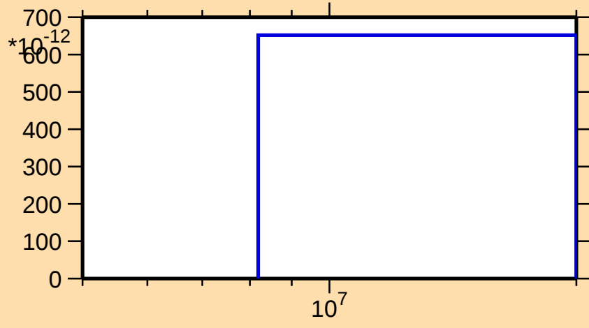
\sigma vs. E for ^{237}\text{Pa}(n,2n\alpha)
