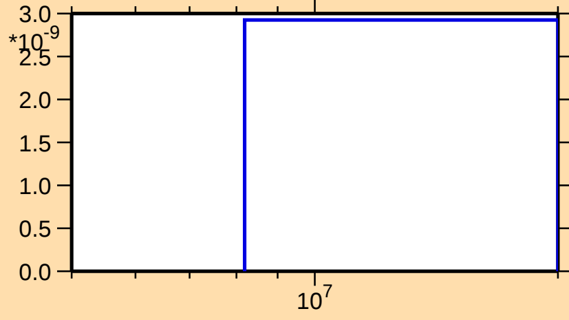
\sigma vs. E for ^{237}\text{Pa}(n,2np)
