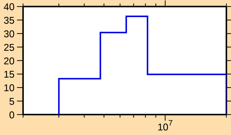
\Delta\sigma/\sigma vs. E for ^{237}\text{Pa}(n,\text{el.})
