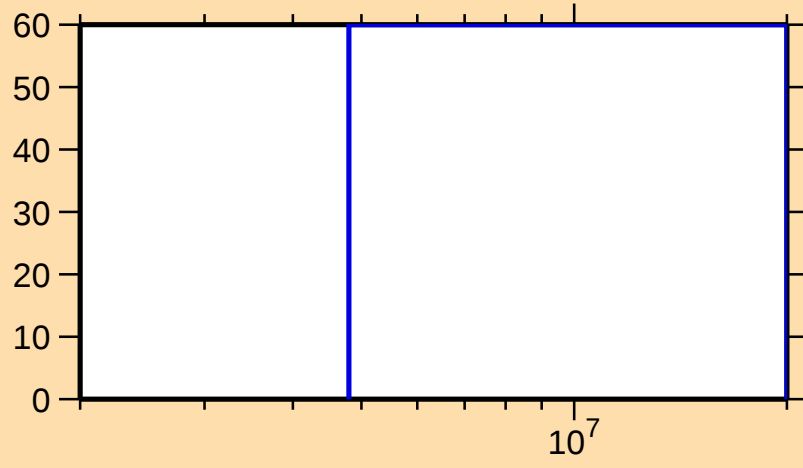
\Delta\sigma/\sigma vs. E for ^{237}\text{Pa}(n,2n)
