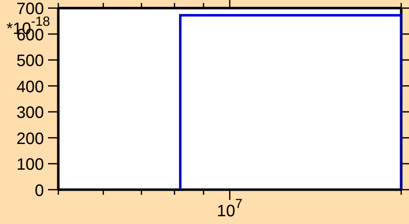
\sigma vs. E for ^{237}\text{Pa}(n,\text{He}3)
