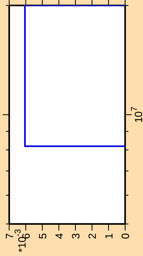
\Delta\sigma/\sigma vs. E for ^{237}\text{Pa}(n,\text{He}3)
