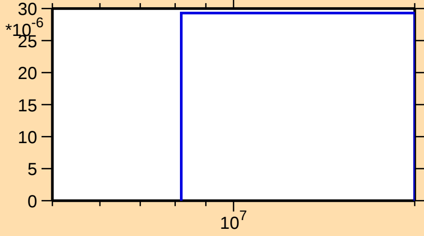
\sigma vs. E for ^{237}\text{Pa}(n,t)
