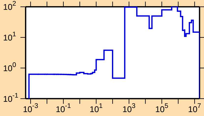
\Delta\sigma/\sigma vs. E for ^{237}\text{Pa}(n,\text{el.})
