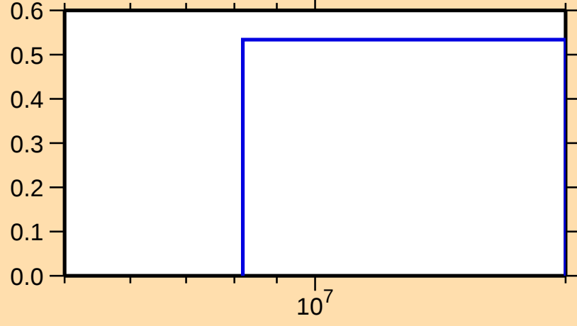
\sigma vs. E for ^{237}\text{Pa}(n,3n)
