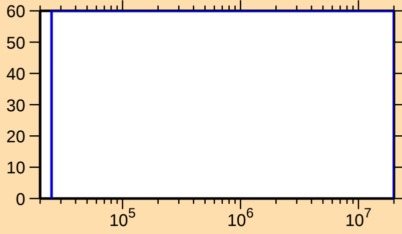
\Delta\sigma/\sigma vs. E for ^{237}\text{Pa}(n,n_1)
