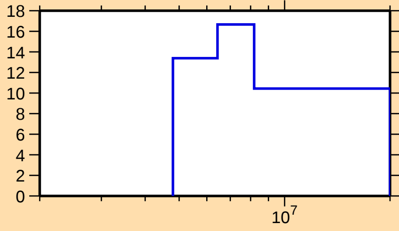
\Delta\sigma/\sigma vs. E for ^{237}\text{Pa}(n,\text{tot.})
