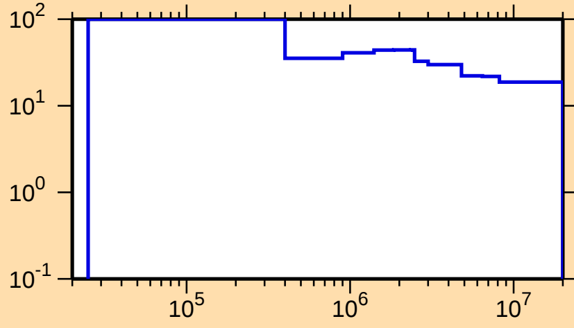
\Delta\sigma/\sigma vs. E for ^{237}\text{Pa}(n,\text{nonel.})
