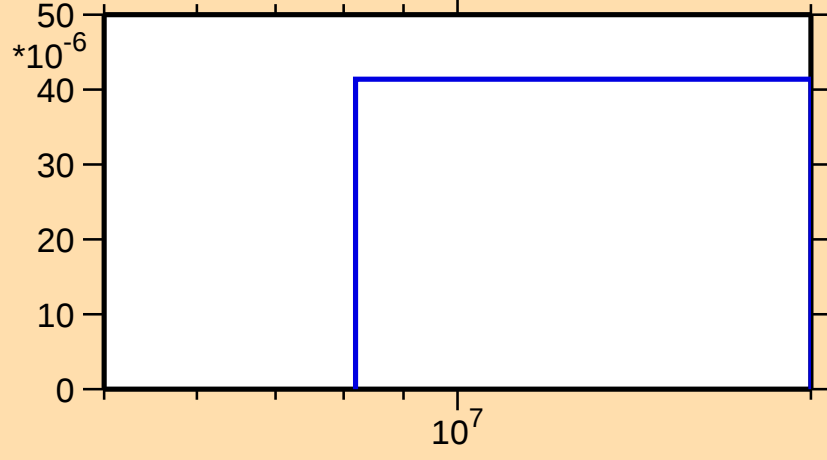
\sigma vs. E for ^{237}\text{Pa}(n,np)
