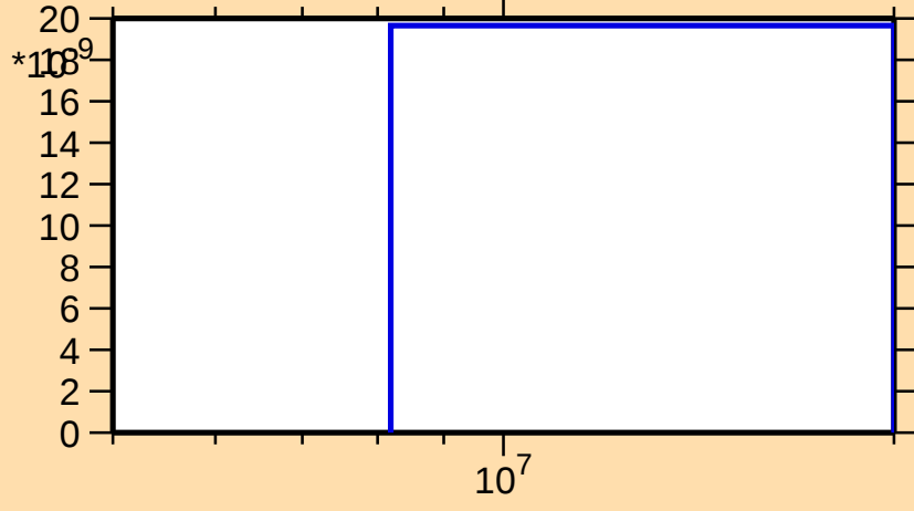
\sigma vs. E for ^{237}\text{Pa}(n,\text{nd})
