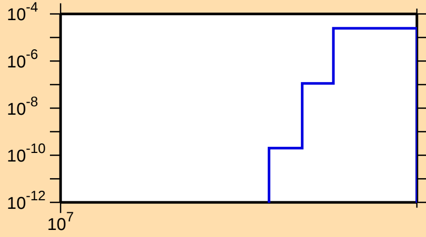
\sigma vs. E for ^{186}\text{Pb}(n,2np)
