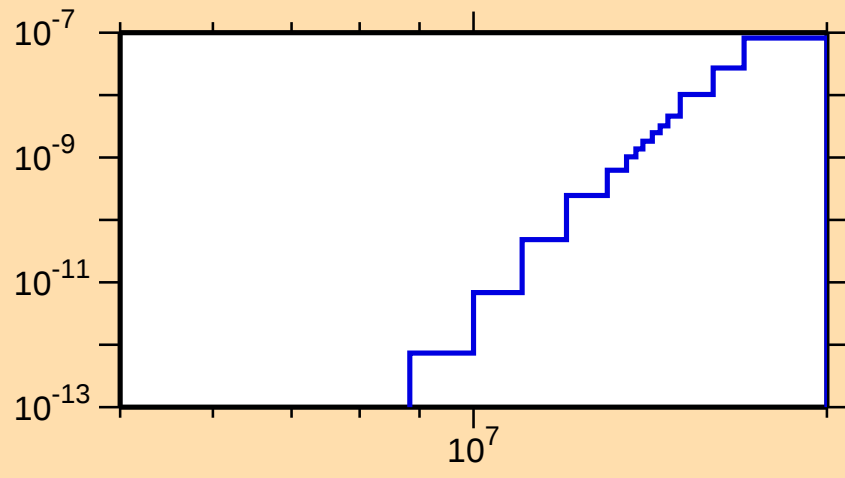
\sigma vs. E for ^{186}\text{Pb}(\text{mt117})
