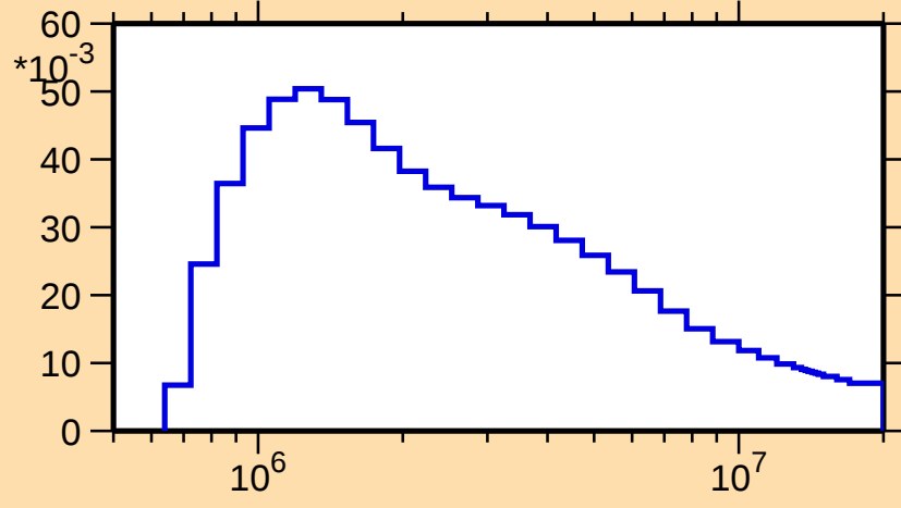
\sigma vs. E for ^{186}\text{Pb}(n,n_3)
