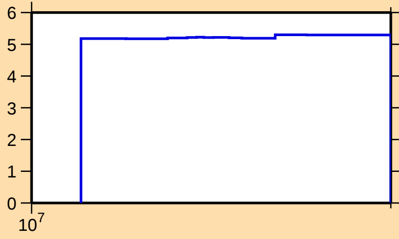
\Delta\sigma/\sigma vs. E for ^{186}\text{Pb}(n,\text{tot.})
