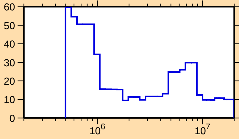
\Delta\sigma/\sigma vs. E for ^{186}\text{Pb}(n,\text{el.})
