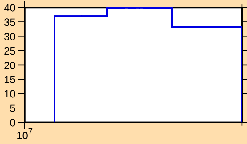
\Delta\sigma/\sigma vs. E for ^{186}\text{Pb}(n,\text{inel.})
