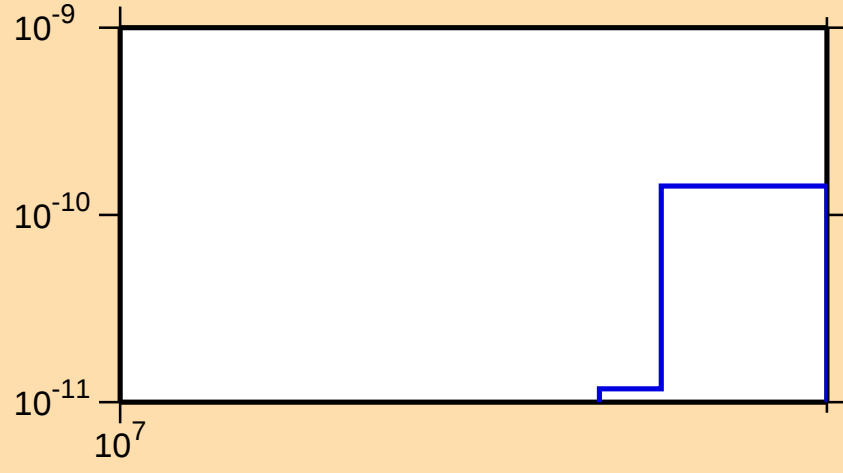
\sigma vs. E for ^{186}\text{Pb}(\text{mt } 34)
