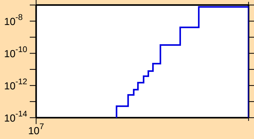
\sigma vs. E for ^{186}\text{Pb}(n,\text{pt})
