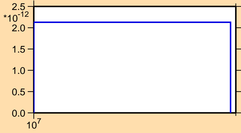
\sigma vs. E for ^{186}\text{Pb} (mt 34)
