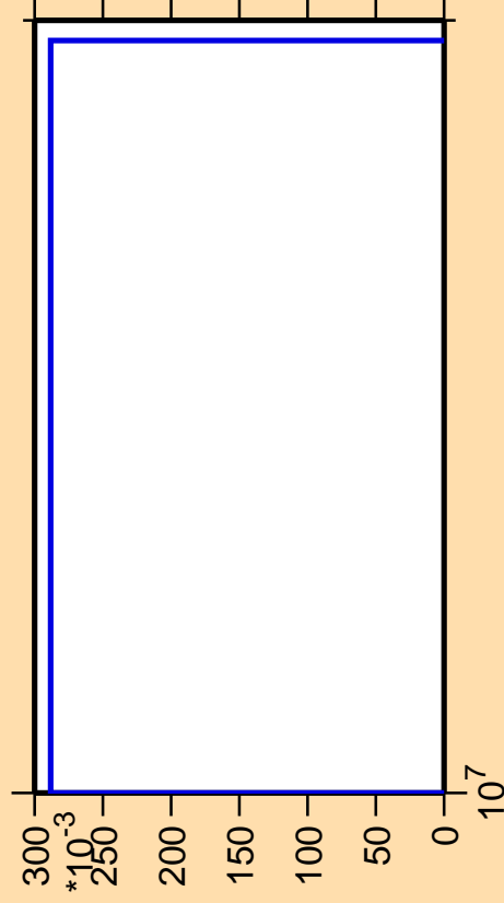
\Delta\sigma/\sigma vs. E for ^{186}\text{Pb}(n,nt)
