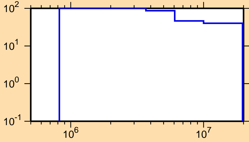
\Delta\sigma/\sigma vs. E for ^{186}\text{Pb}(n,n\text{cont.})
