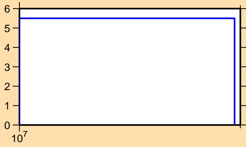
\Delta\sigma/\sigma vs. E for ^{186}\text{Pb}(n,\text{nonel.})
