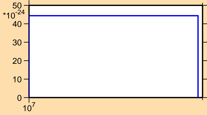
\sigma vs. E for ^{186}\text{Pb} (mt 11)
