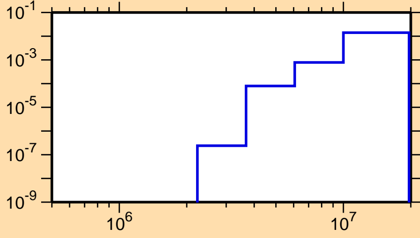
\sigma vs. E for ^{186}\text{Pb}(n,n\alpha)
