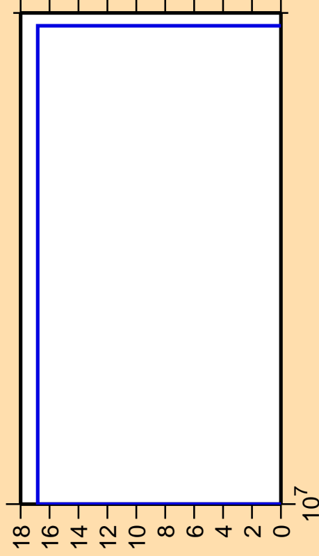
\Delta\sigma/\sigma vs. E for ^{186}\text{Pb} (mt 34)
