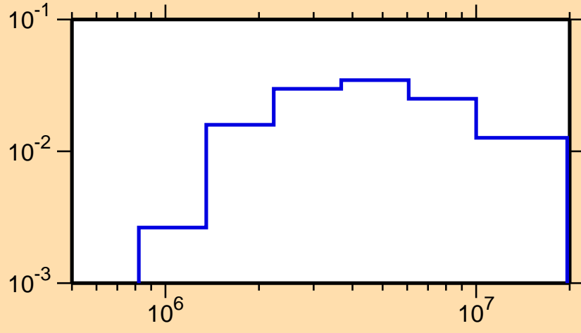
\sigma vs. E for ^{186}\text{Pb}(n,n_4)
