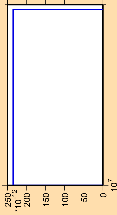
\Delta\sigma/\sigma vs. E for ^{186}\text{Pb} (mt 11)
