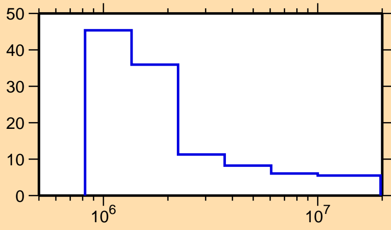
\Delta\sigma/\sigma vs. E for ^{186}\text{Pb}(n,\text{nonel.})
