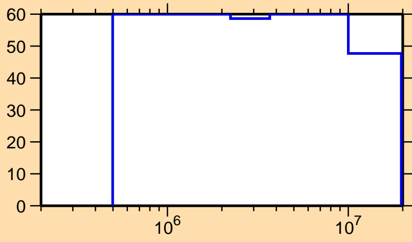
\Delta\sigma/\sigma vs. E for ^{186}\text{Pb}(n,n_1)
