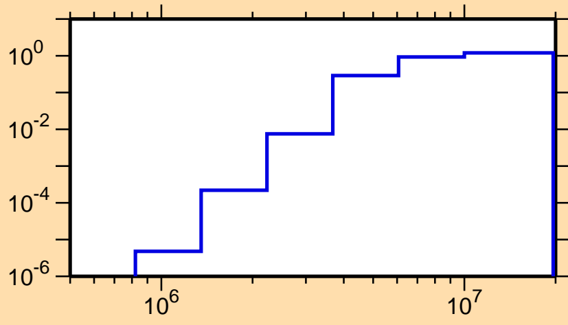
\sigma vs. E for ^{186}\text{Pb}(n,n\text{cont.})
