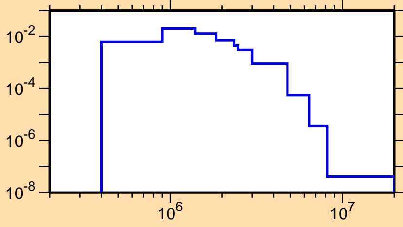
\sigma vs. E for ^{186}\text{Pb}(n,n_2)
