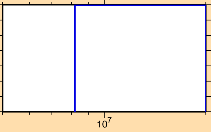
\sigma vs. E for ^{186}\text{Pb}(n,2n\alpha)
