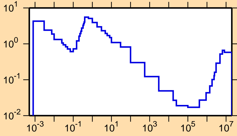
\sigma vs. E for ^{186}\text{Pb}(n,p)
