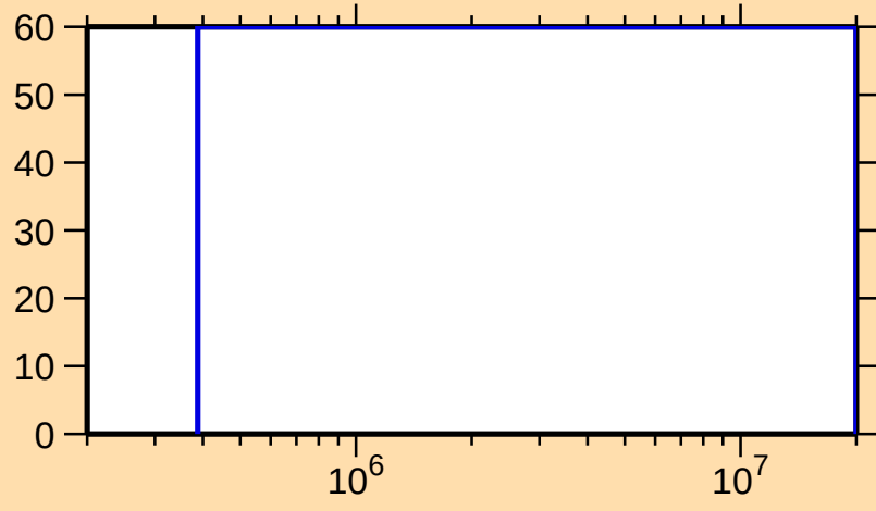
\Delta\sigma/\sigma vs. E for ^{189}\text{Pb}(n,\text{ncont.})
