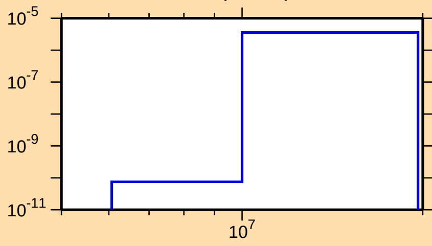
\sigma vs. E for ^{189}\text{Pb}(n,\text{He}3)
