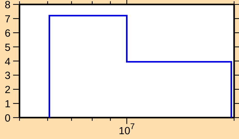
\Delta\sigma/\sigma vs. E for ^{189}\text{Pb}(n,\text{tot.})
