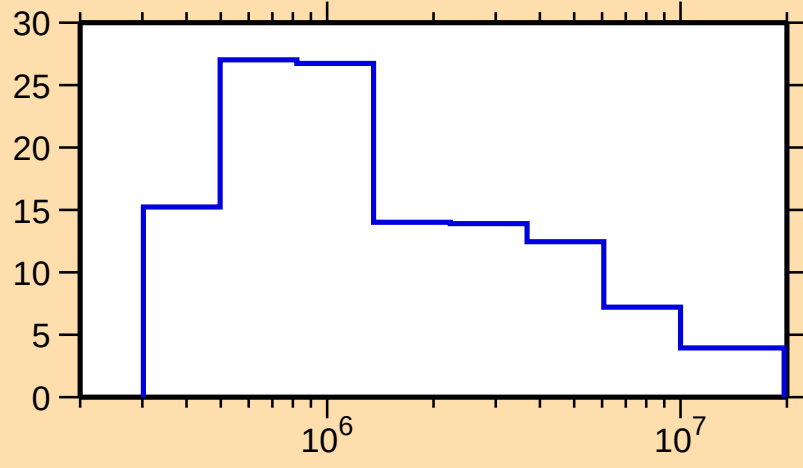
\Delta\sigma/\sigma vs. E for ^{189}\text{Pb}(n,\text{tot.})
