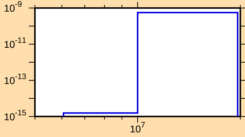
\sigma vs. E for ^{189}\text{Pb}(\text{mt117})
