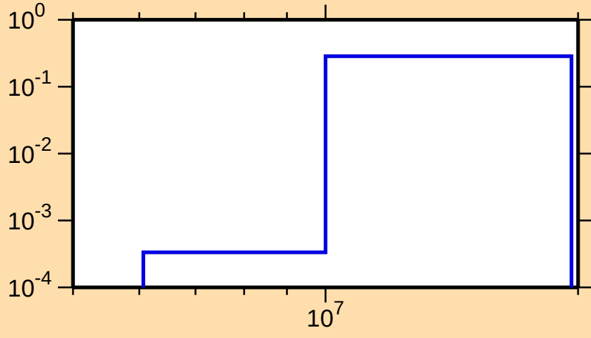
\sigma vs. E for ^{189}\text{Pb}(n,2n)
