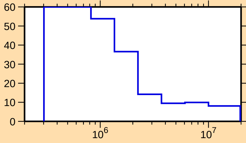
\Delta\sigma/\sigma vs. E for ^{189}\text{Pb}(n,\text{nonel.})
