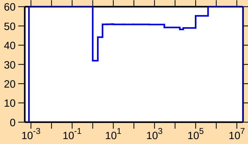
\Delta\sigma/\sigma vs. E for ^{189}\text{Pb}(n,\gamma)
