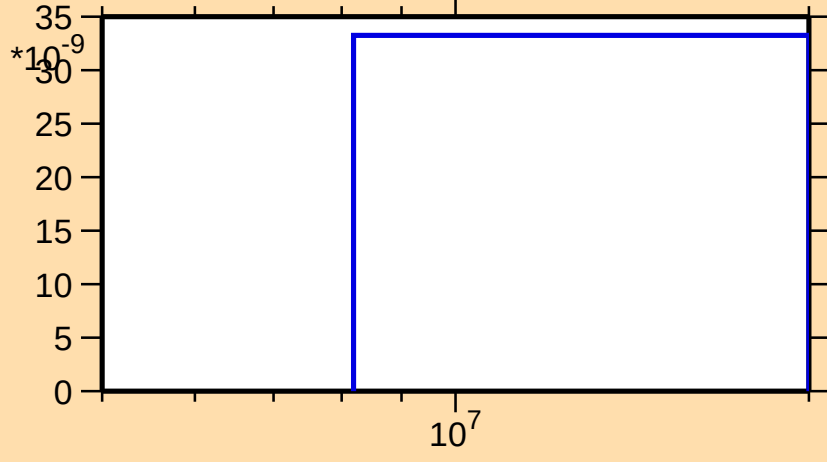
\sigma vs. E for ^{189}\text{Pb}(n,\text{nd})
