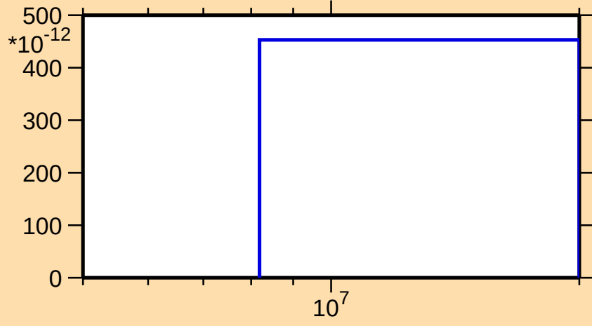
\sigma vs. E for ^{189}\text{Pb}(\text{mt117})
