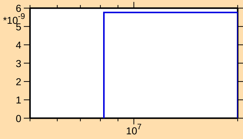
\sigma vs. E for ^{189}\text{Pb}(n,3n)
