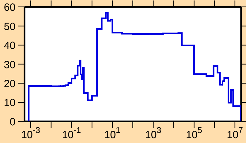
\Delta\sigma/\sigma vs. E for ^{189}\text{Pb}(n,\text{el.})
