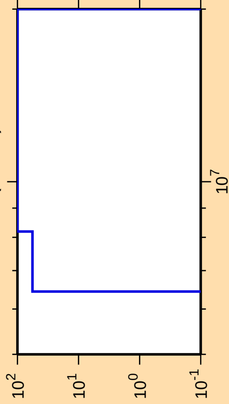
\Delta\sigma/\sigma vs. E for ^{189}\text{Pb}(n,\text{He}3)
