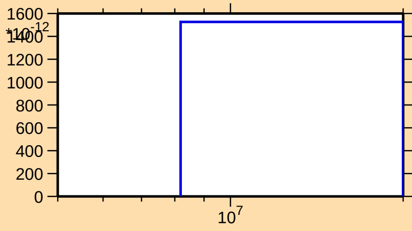
\sigma vs. E for ^{189}\text{Pb}(n,\text{pt})
