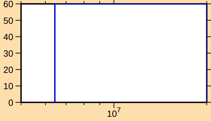
\Delta\sigma/\sigma vs. E for ^{189}\text{Pb}(n,2n)
