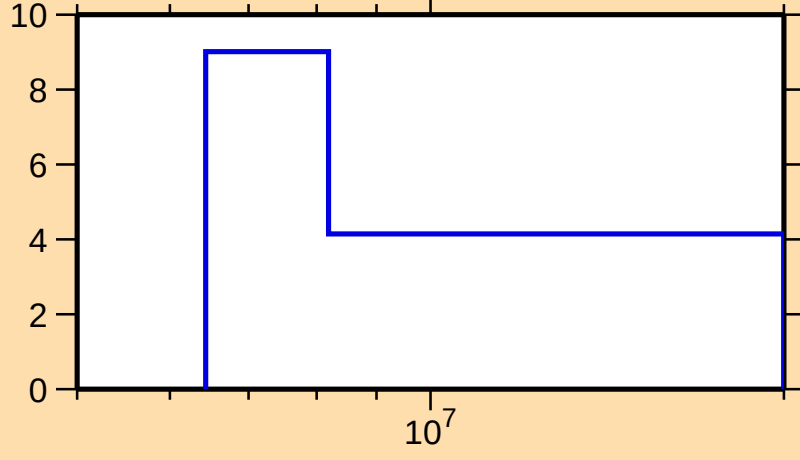
\Delta\sigma/\sigma vs. E for ^{189}\text{Pb}(n,\text{tot.})
