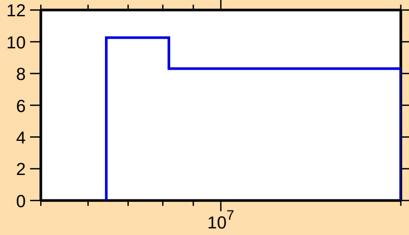
\Delta\sigma/\sigma vs. E for ^{189}\text{Pb}(n,\text{nonel.})
