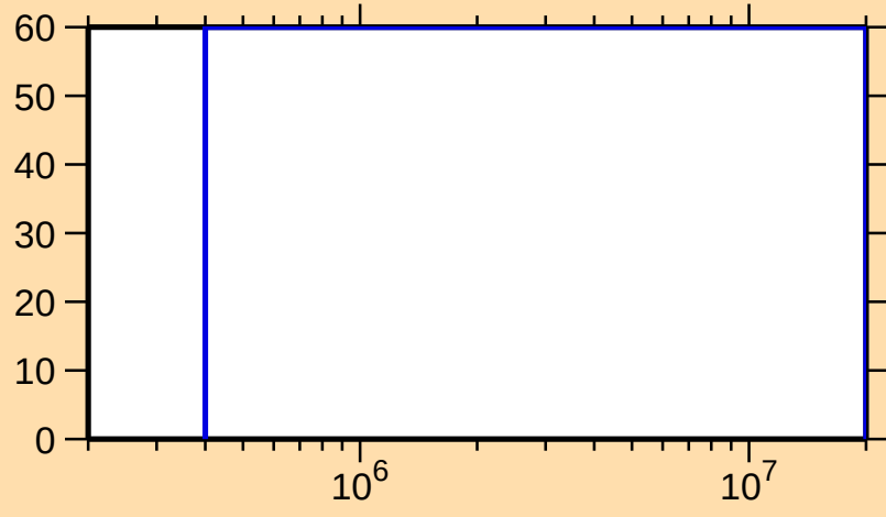
\Delta\sigma/\sigma vs. E for ^{189}\text{Pb}(n,n\text{cont.})
