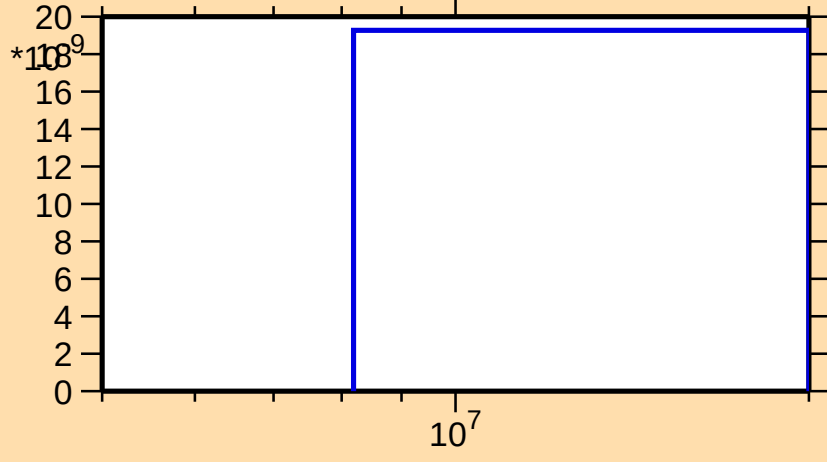
\sigma vs. E for ^{189}\text{Pb}(n,\text{pd})
