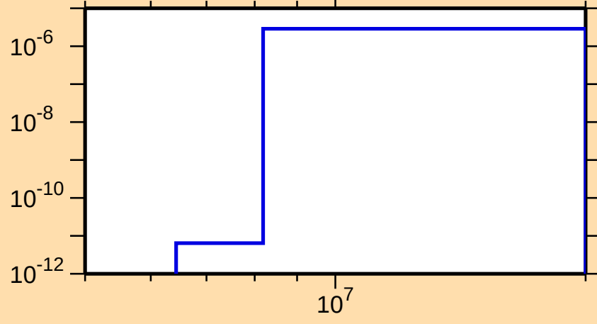
\sigma vs. E for ^{189}\text{Pb}(n,\text{He}3)
