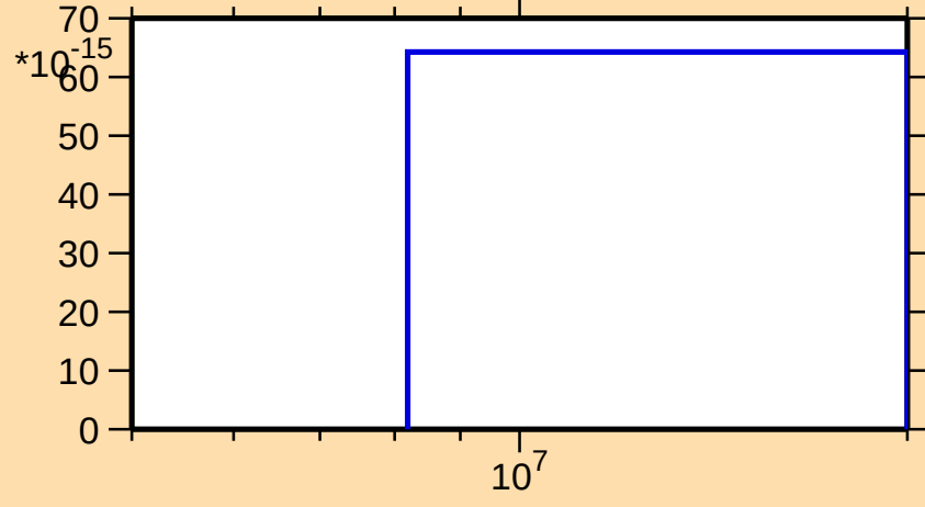
\sigma vs. E for ^{189}\text{Pb}(n,nt)
