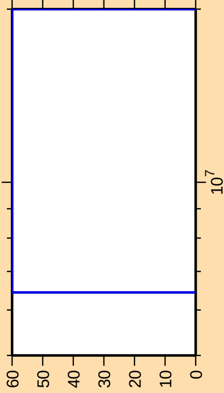
\Delta\sigma/\sigma vs. E for ^{189}\text{Pb}(n,\gamma)
