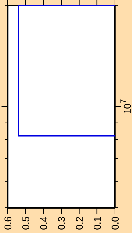
\Delta\sigma/\sigma vs. E for ^{189}\text{Pb}(n,nt)
