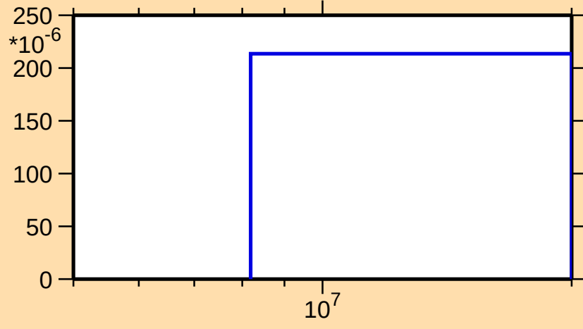
\sigma vs. E for ^{189}\text{Pb}(n,2n\alpha)
