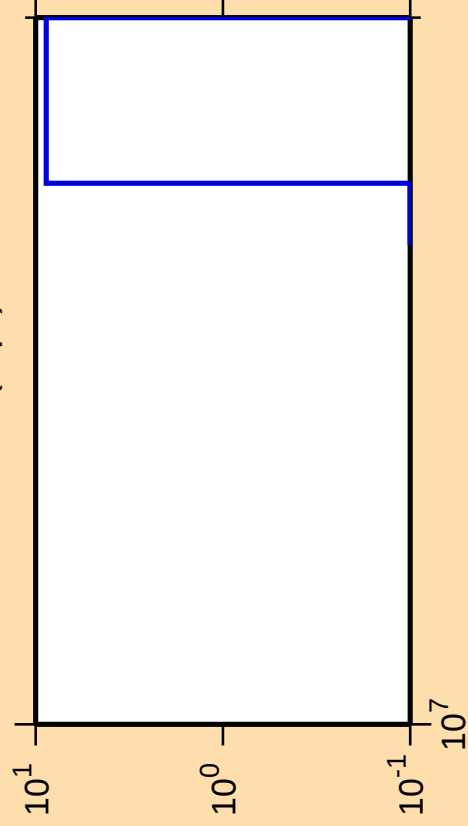
\Delta\sigma/\sigma vs. E for ^{194}\text{Pb}(n,\text{pt})
