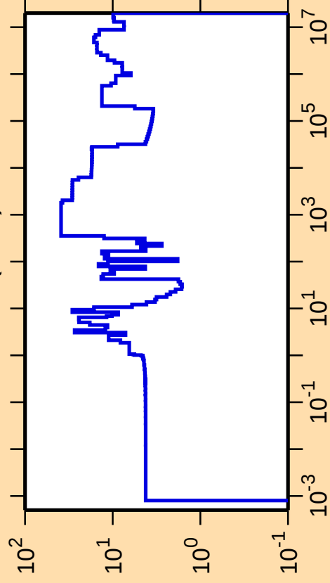
\Delta\sigma/\sigma vs. E for ^{194}\text{Pb}(n,\text{el.})
