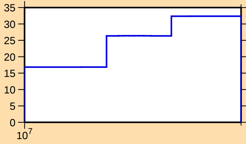
\Delta\sigma/\sigma vs. E for ^{194}\text{Pb}(n,\text{inel.})
