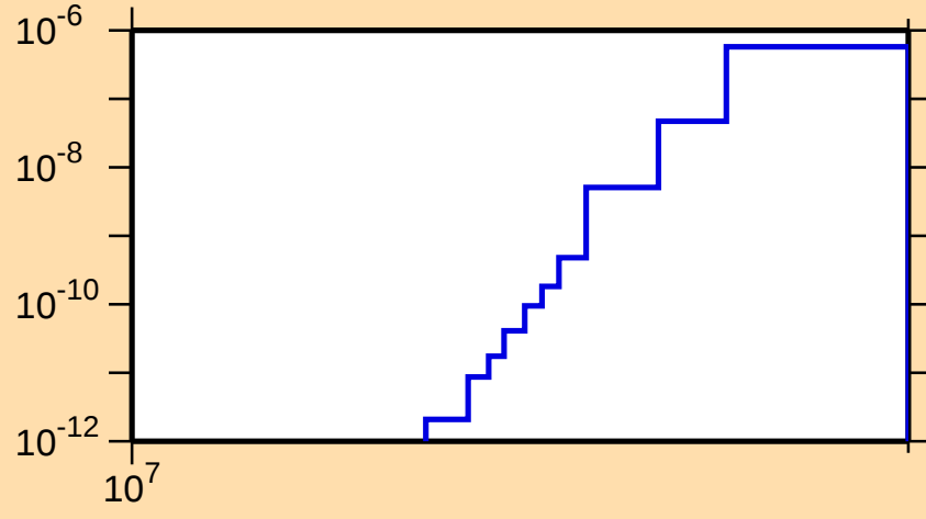
\sigma vs. E for ^{194}\text{Pb}(n,2n\alpha)
