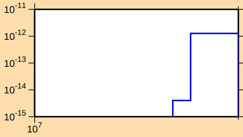
\sigma vs. E for ^{194}\text{Pb}(n,\text{pt})
