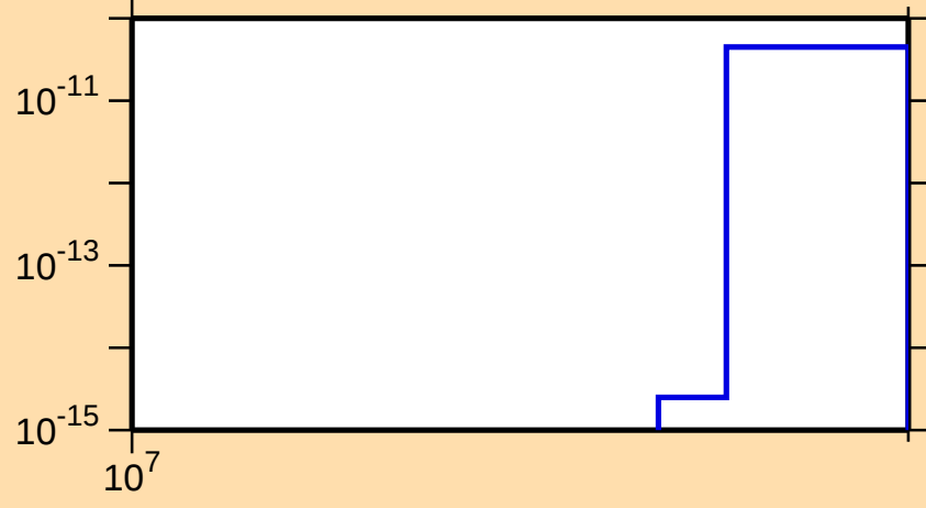
\sigma vs. E for ^{194}\text{Pb}(n,nt)
