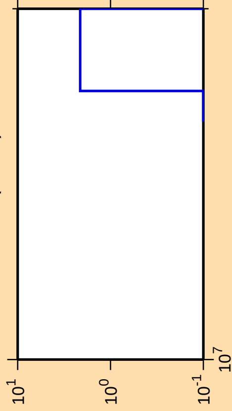
\Delta\sigma/\sigma vs. E for ^{194}\text{Pb}(\text{mt } 34)
