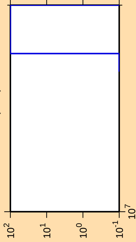
\Delta\sigma/\sigma vs. E for ^{194}\text{Pb}(n,nt)
