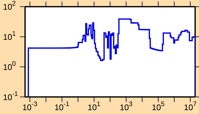
\Delta\sigma/\sigma vs. E for ^{194}\text{Pb}(n,\text{el.})
