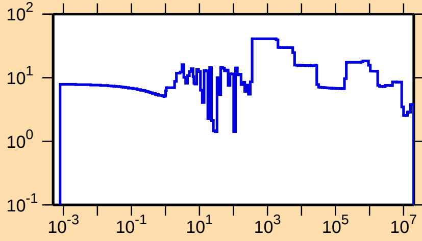
\Delta\sigma/\sigma vs. E for ^{194}\text{Pb}(n,\text{tot.})
