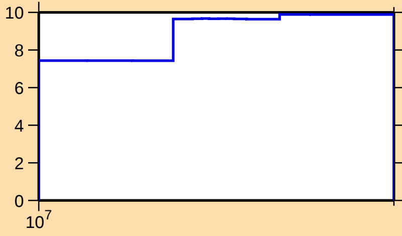
\Delta\sigma/\sigma vs. E for ^{194}\text{Pb}(n,\text{el.})
