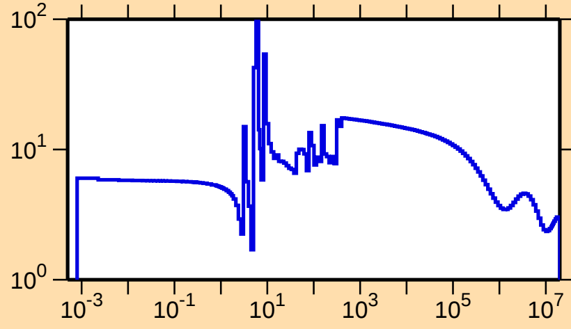
\sigma vs. E for ^{194}\text{Pb}(n,\text{el.})
