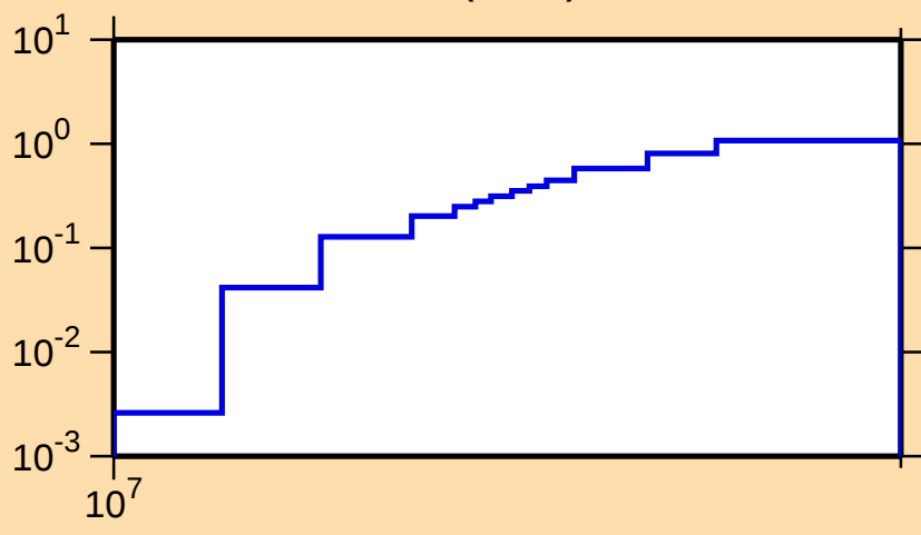
\sigma vs. E for ^{194}\text{Pb}(n,2n)
