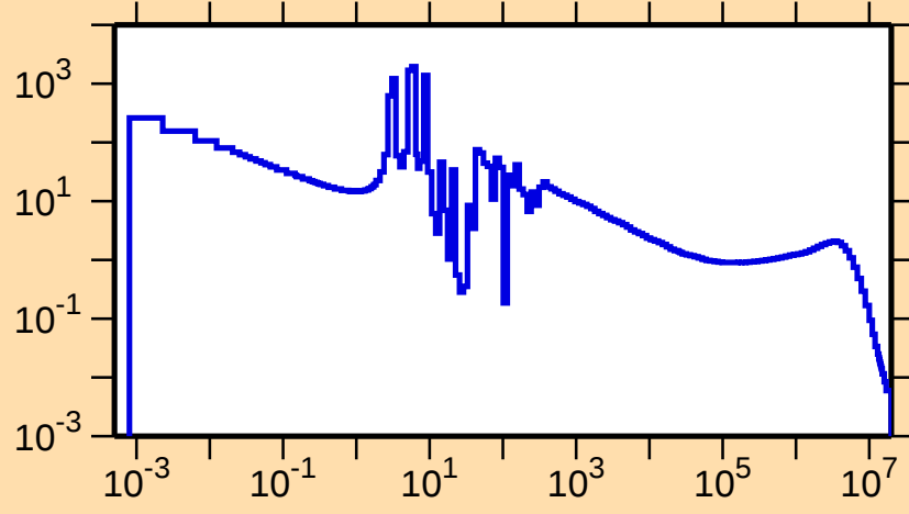
\sigma vs. E for ^{194}\text{Pb}(n,\gamma)
