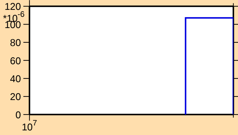
\sigma vs. E for ^{194}\text{Pb}(n,3n)
