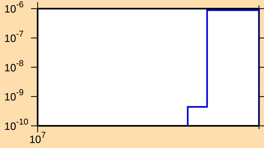
\sigma vs. E for ^{194}\text{Pb}(n,2np)
