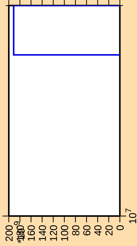
\Delta\sigma/\sigma vs. E for ^{194}\text{Pb}(\text{mt } 11)
