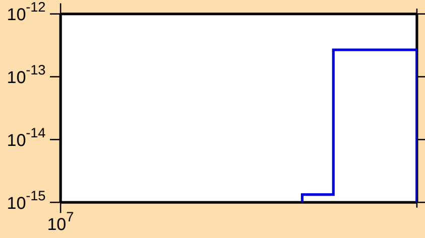
\sigma vs. E for ^{194}\text{Pb}(\text{mt } 34)
