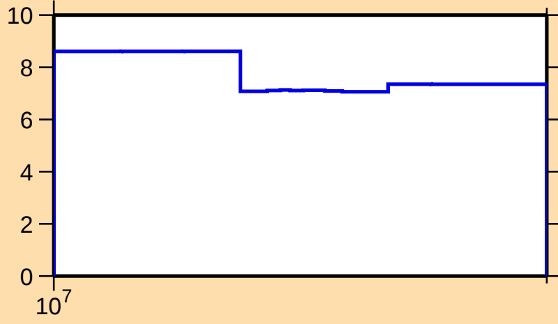
\Delta\sigma/\sigma vs. E for ^{194}\text{Pb}(n,\text{nonel.})
