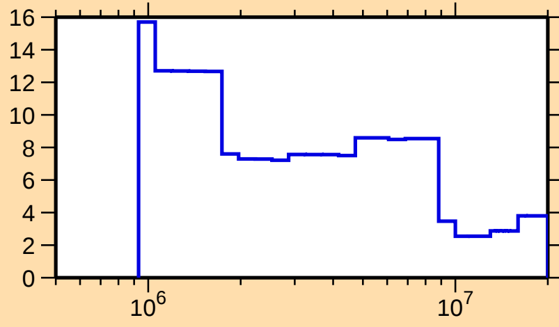
\Delta\sigma/\sigma vs. E for ^{194}\text{Pb}(n,\text{tot.})
