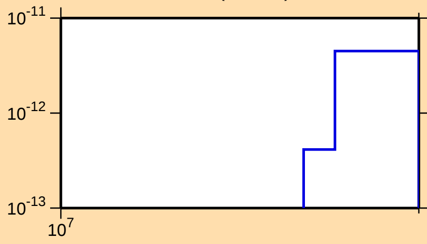
\sigma vs. E for ^{194}\text{Pb}(\text{mt117})
