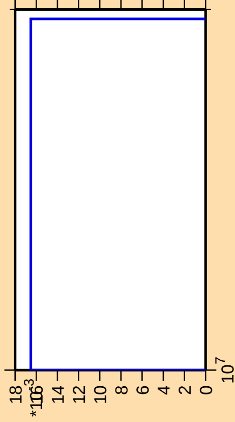
\Delta\sigma/\sigma vs. E for ^{194}\text{Pb}(\text{mt } 34)
