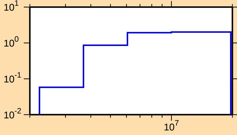
\sigma vs. E for ^{194}\text{Pb}(n,n\text{cont.})
