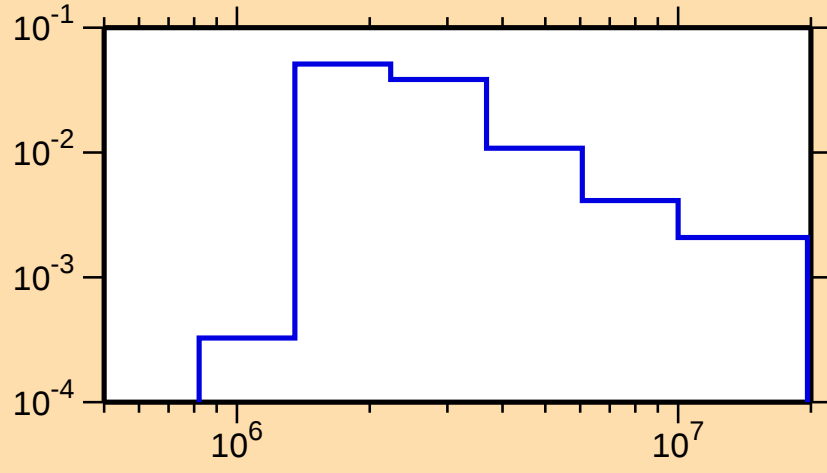
\sigma vs. E for ^{194}\text{Pb}(n,n_3)
