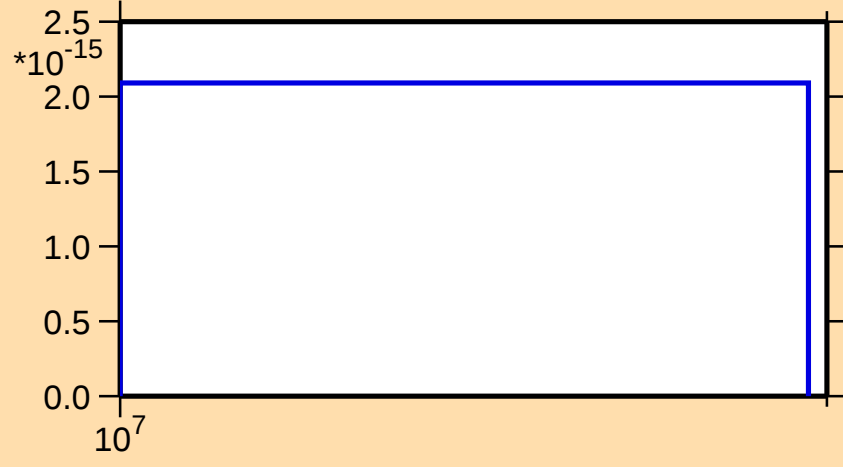
\sigma vs. E for ^{194}\text{Pb}(\text{mt } 34)
