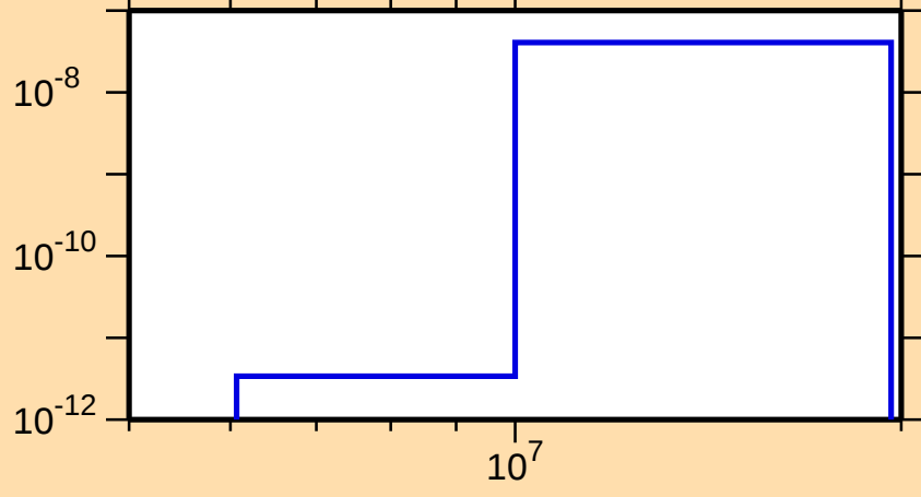
\sigma vs. E for ^{194}\text{Pb}(n,p\alpha)
