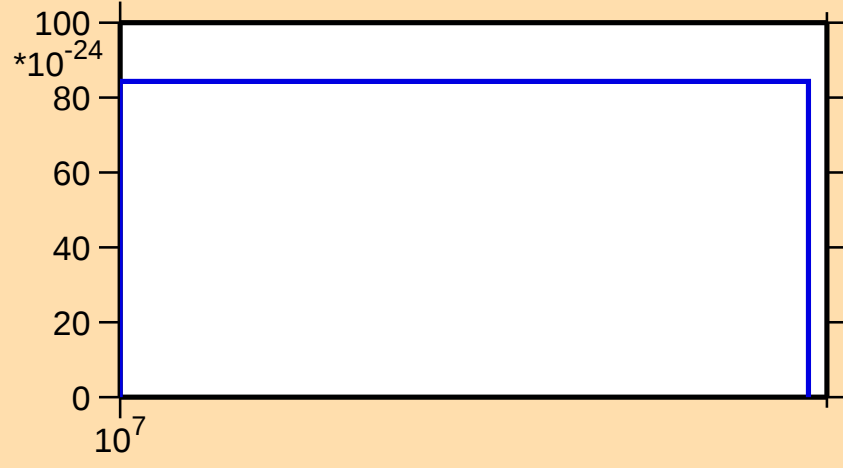
\sigma vs. E for ^{194}\text{Pb}(\text{mt } 11)
