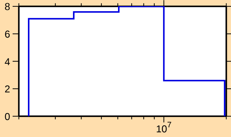
\Delta\sigma/\sigma vs. E for ^{194}\text{Pb}(n,\text{tot.})
