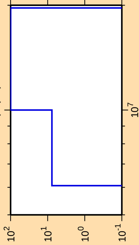
\Delta\sigma/\sigma vs. E for ^{194}\text{Pb}(n,p\alpha)
