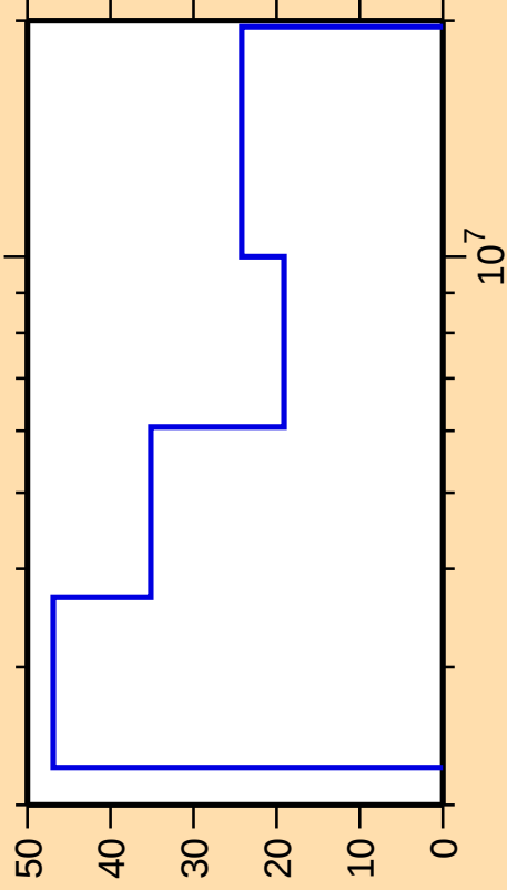
\Delta\sigma/\sigma vs. E for ^{194}\text{Pb}(n,n\text{cont.})
