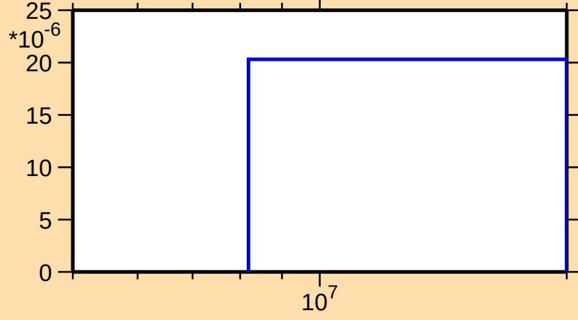
\sigma vs. E for ^{194}\text{Pb}(n,t)
