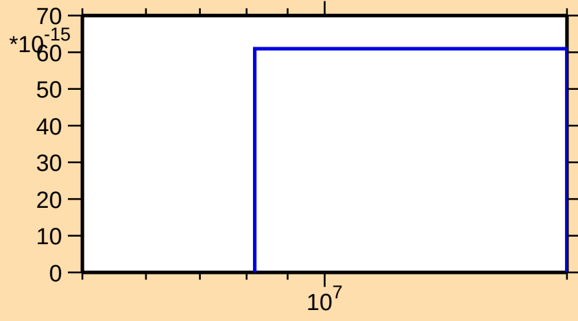
\sigma vs. E for ^{194}\text{Pb}(\text{mt117})
