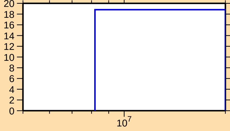
\Delta\sigma/\sigma vs. E for ^{194}\text{Pb}(n,\text{inel.})
