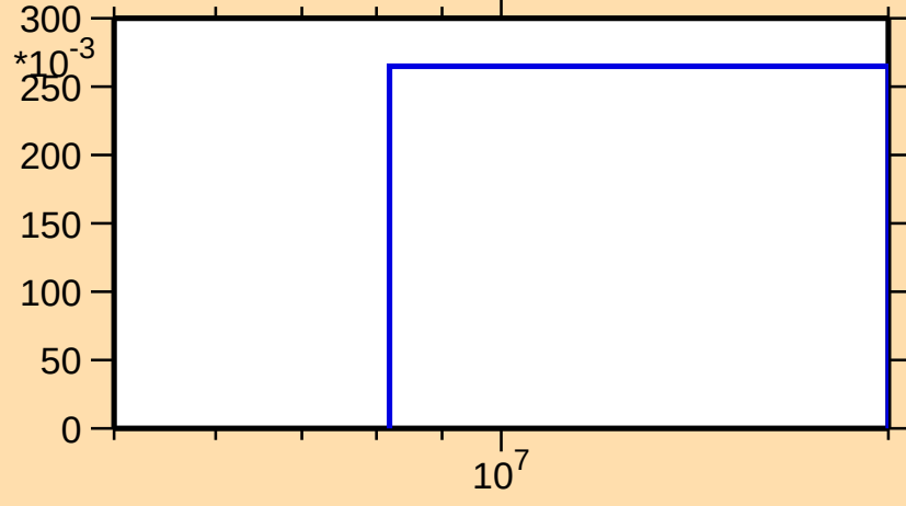
\sigma vs. E for ^{194}\text{Pb}(n,2n)
