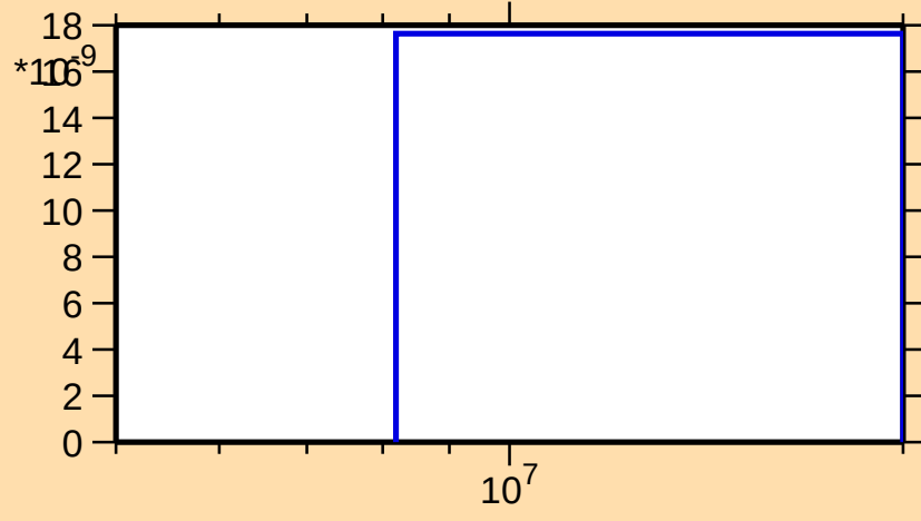
\sigma vs. E for ^{194}\text{Pb}(n,\text{He}3)
