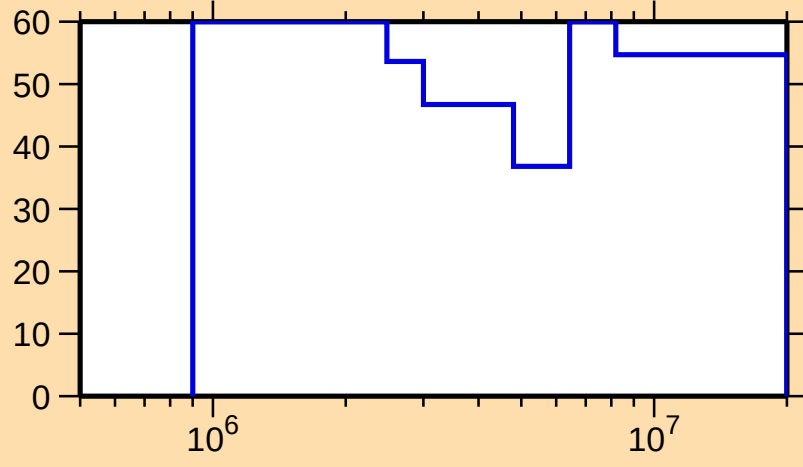
\Delta\sigma/\sigma vs. E for ^{194}\text{Pb}(n,n_1)
