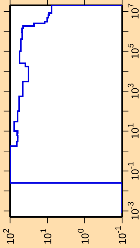
\Delta\sigma/\sigma vs. E for ^{194}\text{Pb}(n,\text{nonel.})
