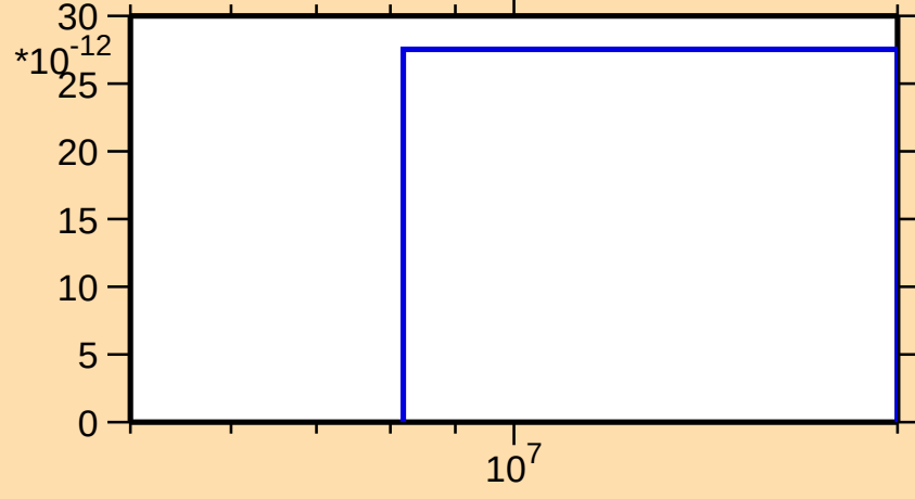
\sigma vs. E for ^{194}\text{Pb}(n,\text{pd})
