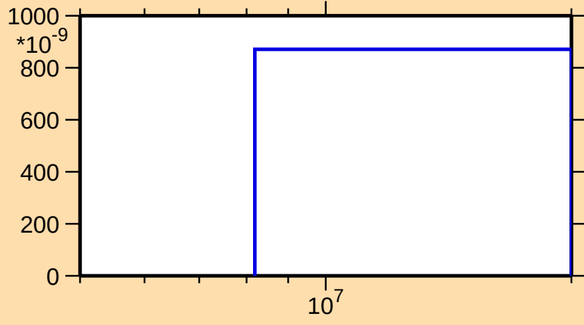
\sigma vs. E for ^{194}\text{Pb}(n,3n)
