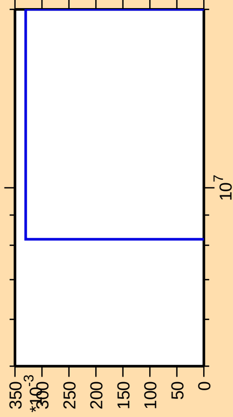
\Delta\sigma/\sigma vs. E for ^{194}\text{Pb}(\text{mt117})
