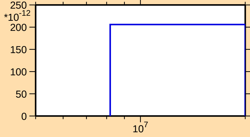
\sigma vs. E for ^{194}\text{Pb}(n,\text{nd})
