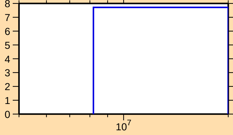
\Delta\sigma/\sigma vs. E for ^{194}\text{Pb}(n,\text{nonel.})
