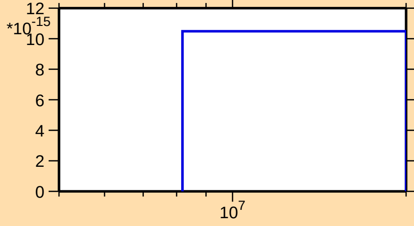
\sigma vs. E for ^{194}\text{Pb}(n,\text{pt})
