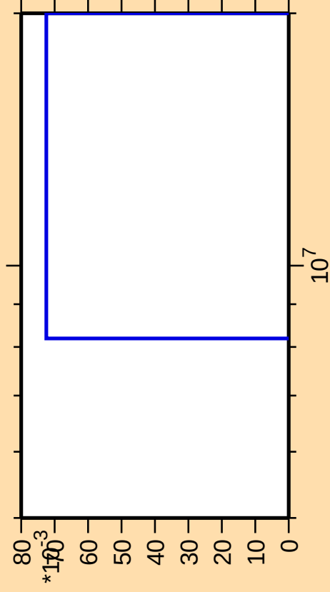
\Delta\sigma/\sigma vs. E for ^{194}\text{Pb}(n,\text{pt})
