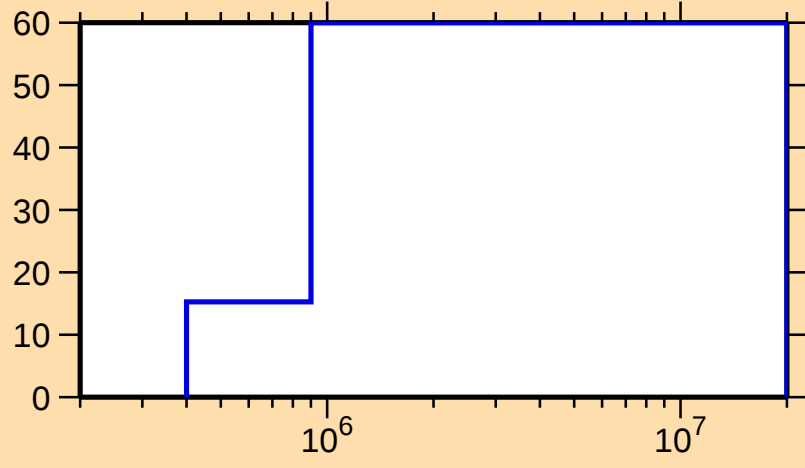
\Delta\sigma/\sigma vs. E for ^{203}\text{Pb}(n,p)
