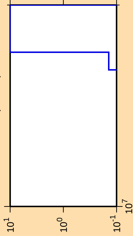
\Delta\sigma/\sigma vs. E for ^{206}\text{Pb}(n,\text{He3})
