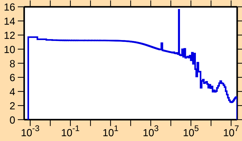
\sigma vs. E for ^{206}\text{Pb}(n,\text{el.})
