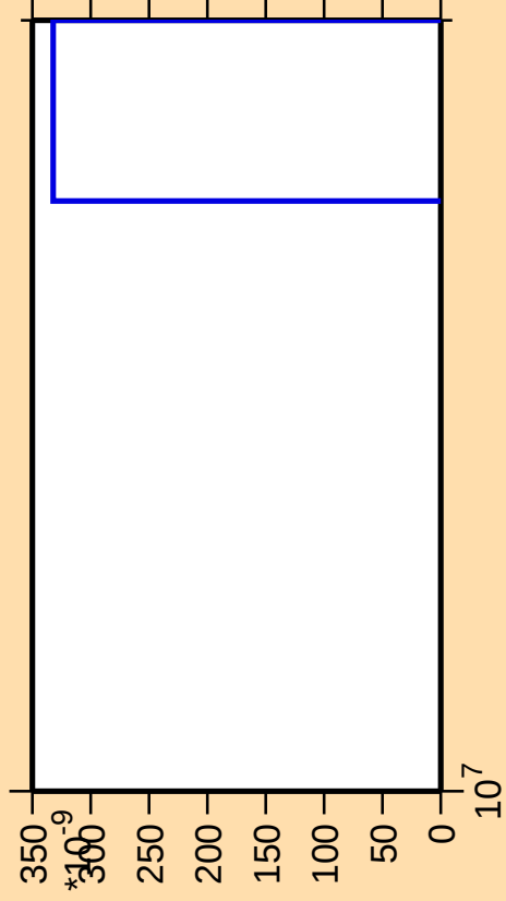
\Delta\sigma/\sigma vs. E for ^{206}\text{Pb}(\text{mt 11})
