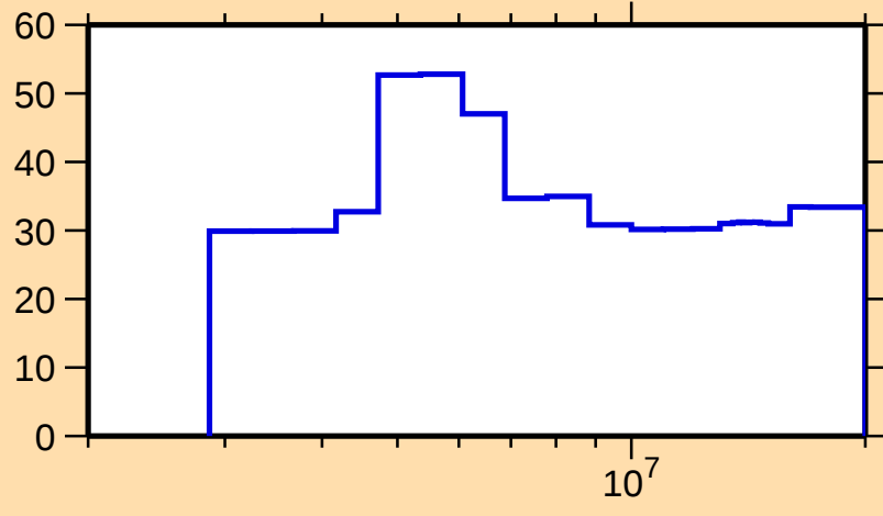
\Delta\sigma/\sigma vs. E for ^{206}\text{Pb}(n,n_1)
