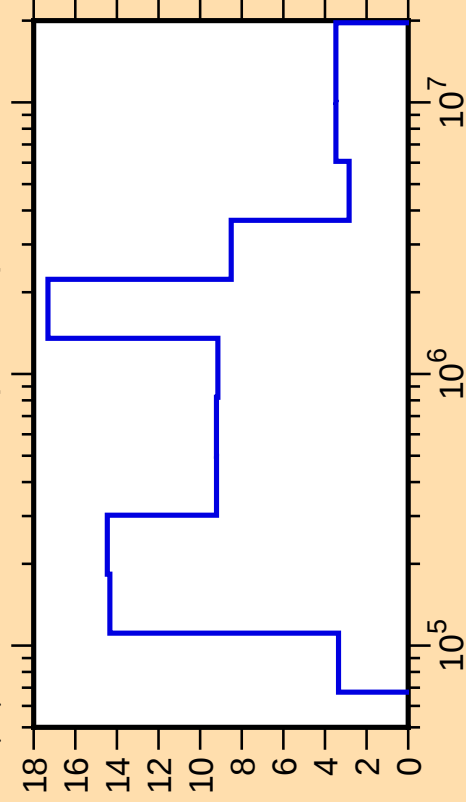
\Delta\mu/\mu vs. E for ^{206}\text{Pb}(\text{mt251})
