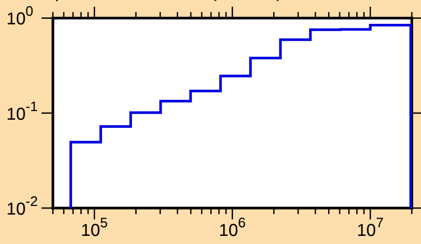
\mu vs. E for ^{206}\text{Pb}(\text{mt251})
