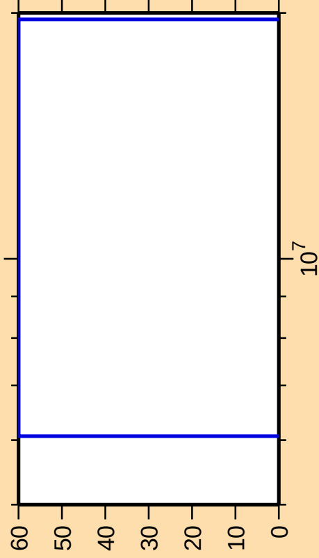
\Delta\sigma/\sigma vs. E for ^{206}\text{Pb}(n,\gamma)
