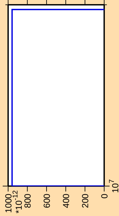
\Delta\sigma/\sigma vs. E for ^{206}\text{Pb}(\text{mt } 11)
