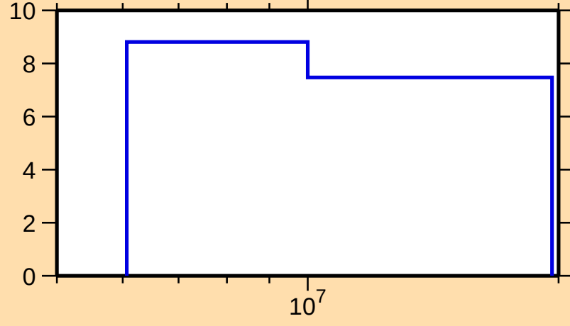
\Delta\sigma/\sigma vs. E for ^{206}\text{Pb}(n,\text{el.})
