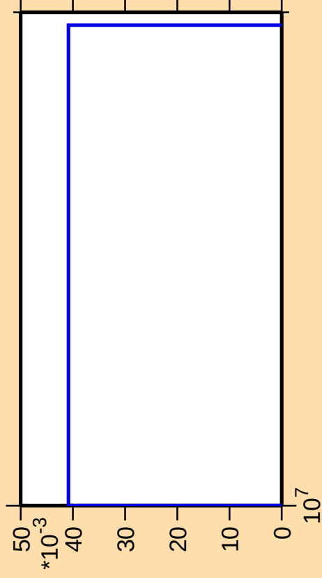
\Delta\sigma/\sigma vs. E for ^{206}\text{Pb}(n,p\alpha)
