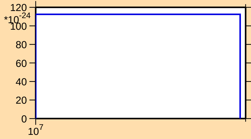
\sigma vs. E for ^{206}\text{Pb}(\text{mt } 11)
