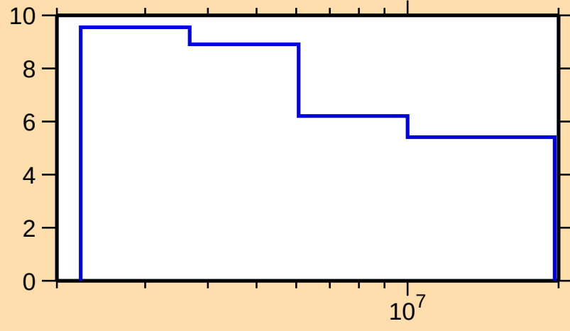
\Delta\sigma/\sigma vs. E for ^{206}\text{Pb}(n,n\text{onel.})
