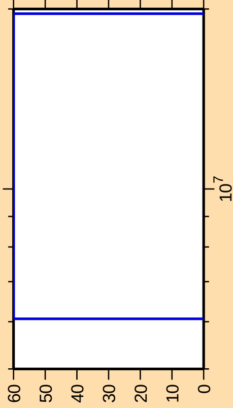
\Delta\sigma/\sigma vs. E for ^{206}\text{Pb}(n,p)
