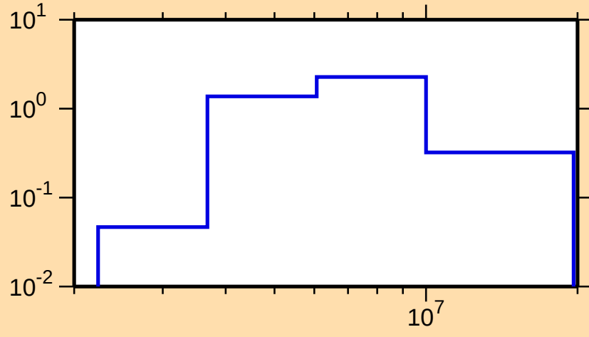
\sigma vs. E for ^{206}\text{Pb}(n,n\text{cont.})
