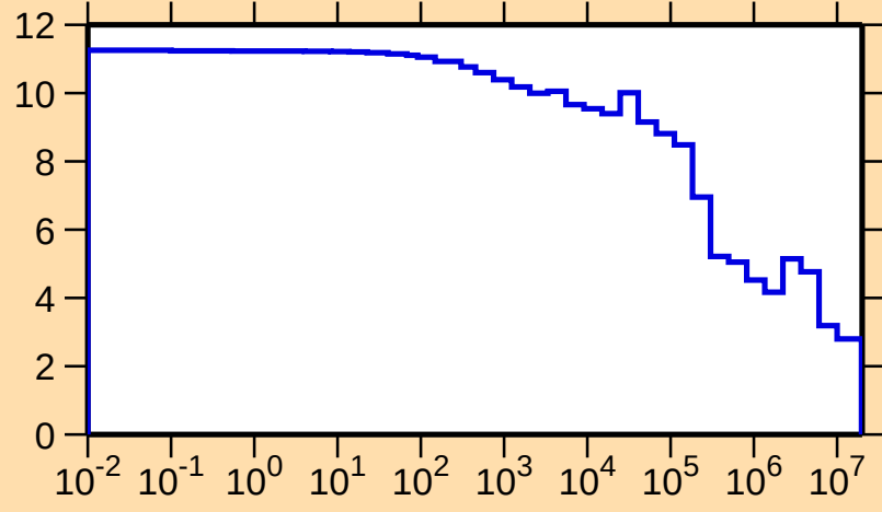
\sigma vs. E for ^{206}\text{Pb}(n,\text{el.})
