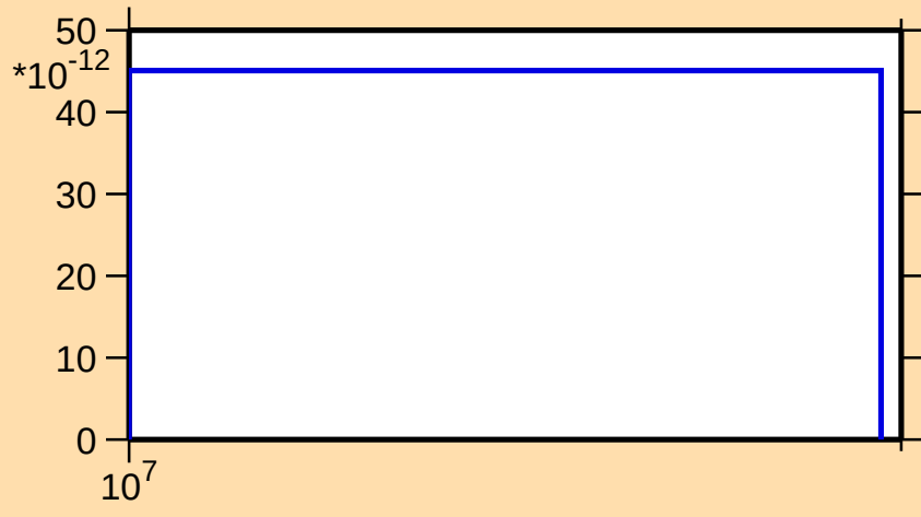
\sigma vs. E for ^{206}\text{Pb}(n,\text{nd})
