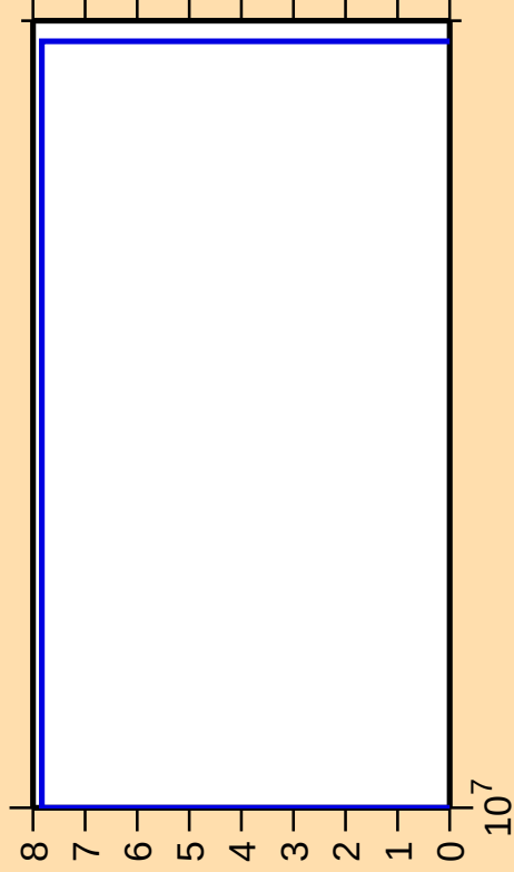
\Delta\sigma/\sigma vs. E for ^{206}\text{Pb}(n,nt)
