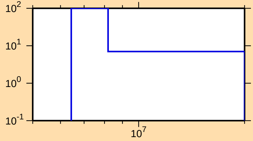
\Delta\sigma/\sigma vs. E for ^{206}\text{Pb}(n,2n)
