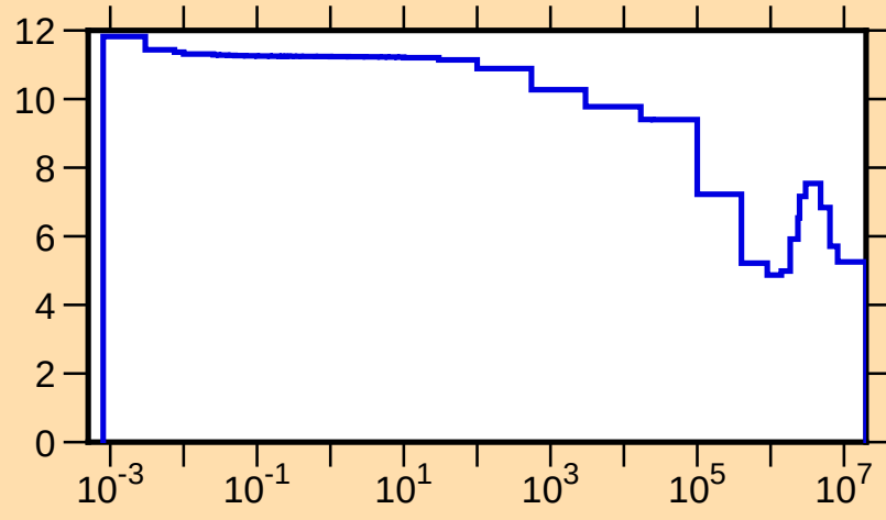
\sigma vs. E for ^{206}\text{Pb}(n,\text{tot.})
