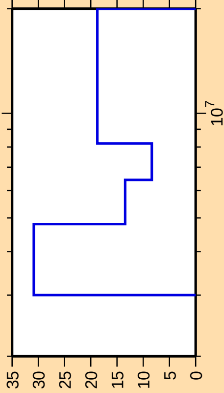
\Delta\sigma/\sigma vs. E for ^{206}\text{Pb}(n,\text{ncont.})
