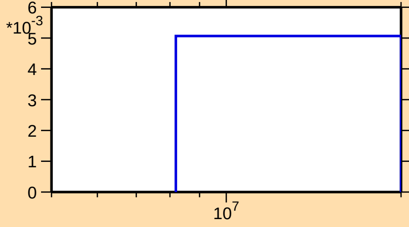
\sigma vs. E for ^{206}\text{Pb}(n,3n)
