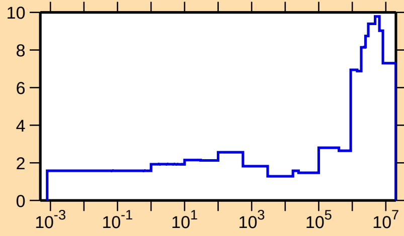
\Delta\sigma/\sigma vs. E for ^{206}\text{Pb}(n,\text{el.})
