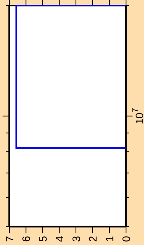
\Delta\sigma/\sigma vs. E for ^{206}\text{Pb}(n,2np)
