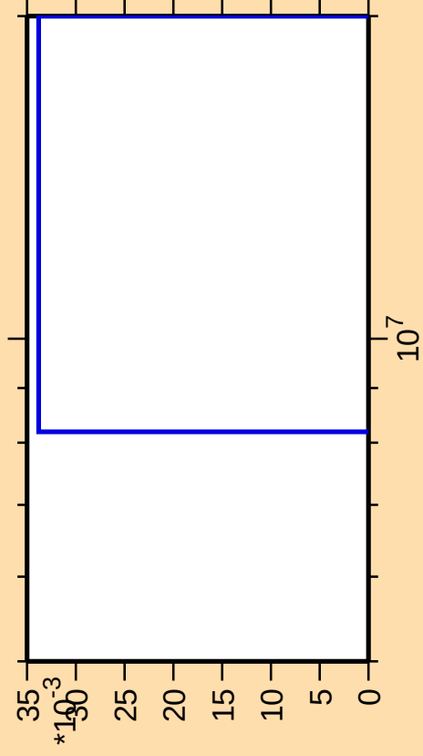
\Delta\sigma/\sigma vs. E for ^{206}\text{Pb}(n,p\alpha)
