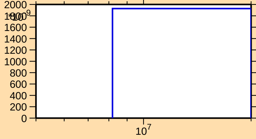
\sigma vs. E for ^{206}\text{Pb}(n,t)
