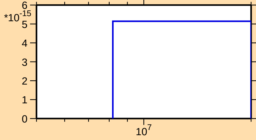
\sigma vs. E for ^{206}\text{Pb}(n,p\alpha)
