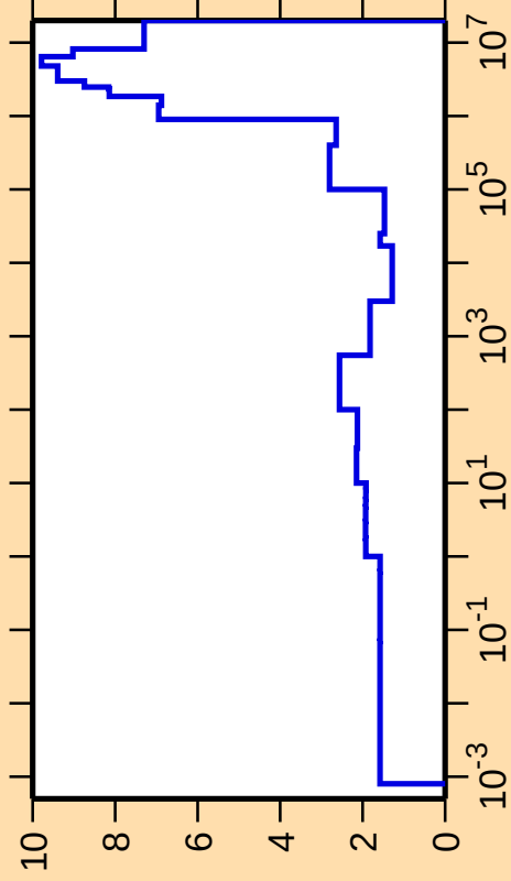
\Delta\sigma/\sigma vs. E for ^{206}\text{Pb}(n,\text{el.})
