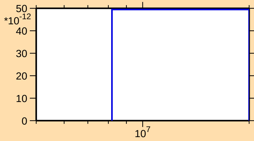
\sigma vs. E for ^{206}\text{Pb}(n,\text{nd})
