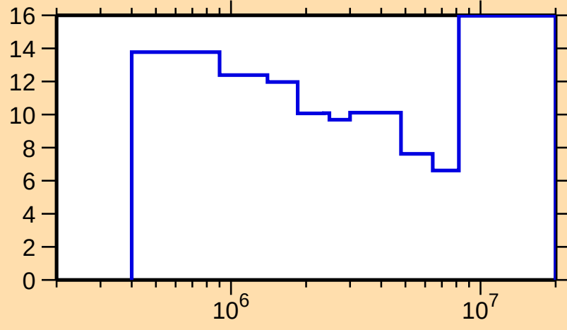
\Delta\sigma/\sigma vs. E for ^{206}\text{Pb}(n,\text{inel.})
