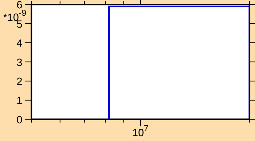
\sigma vs. E for ^{206}\text{Pb}(n,2n\alpha)
