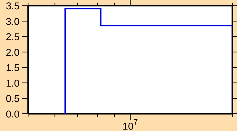
\Delta\sigma/\sigma vs. E for ^{206}\text{Pb}(n,\text{tot.})
