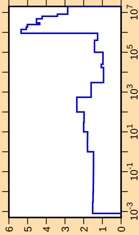
\Delta\sigma/\sigma vs. E for ^{206}\text{Pb}(n,\text{tot.})
