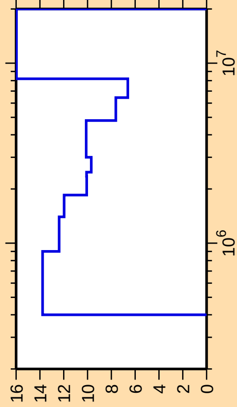
\Delta\sigma/\sigma vs. E for ^{206}\text{Pb}(n,\text{inel.})
