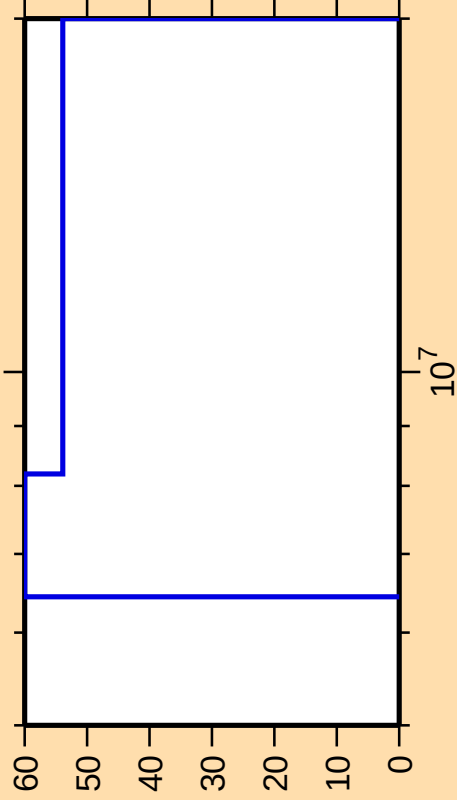
\Delta\sigma/\sigma vs. E for ^{206}\text{Pb}(n,\alpha)
