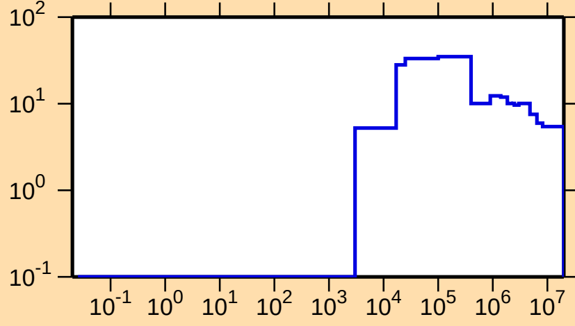
\Delta\sigma/\sigma vs. E for ^{206}\text{Pb}(n,\text{nonel.})
