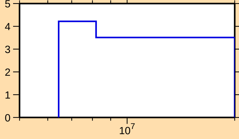
\Delta\sigma/\sigma vs. E for ^{208}\text{Pb}(n,\text{tot.})
