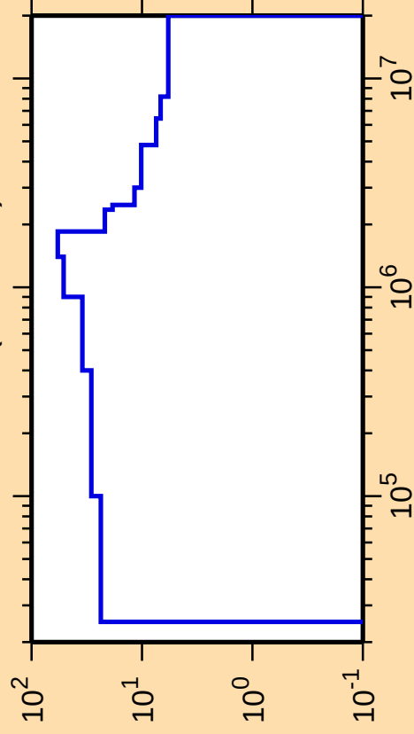
\Delta\sigma/\sigma vs. E for ^{208}\text{Pb}(n,\text{nonel.})
