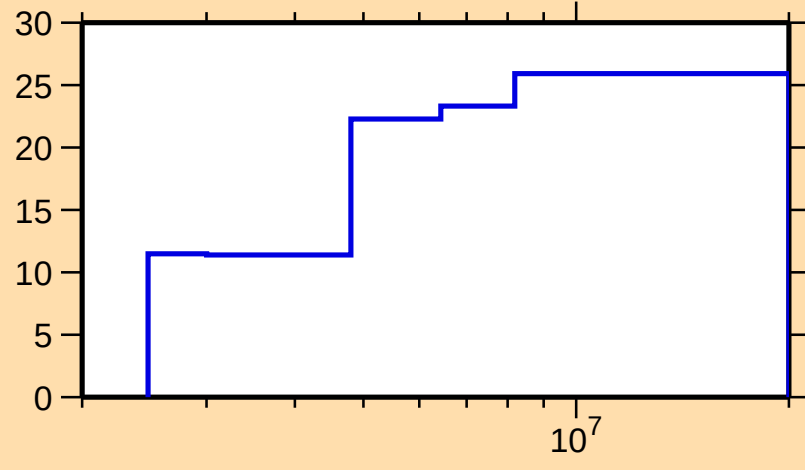
\Delta\sigma/\sigma vs. E for ^{208}\text{Pb}(n,n_1)
