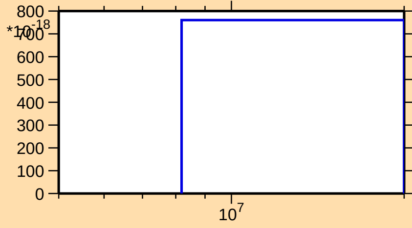
\sigma vs. E for ^{208}\text{Pb}(n,\text{He}3)
