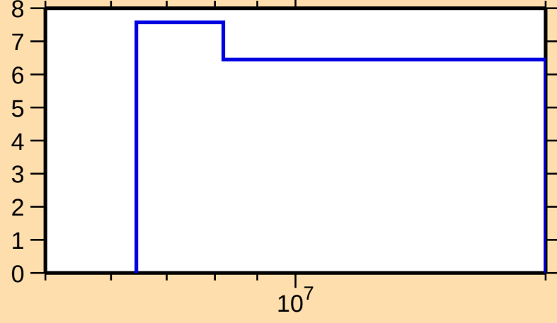
\Delta\sigma/\sigma vs. E for ^{208}\text{Pb}(n,\text{el.})
