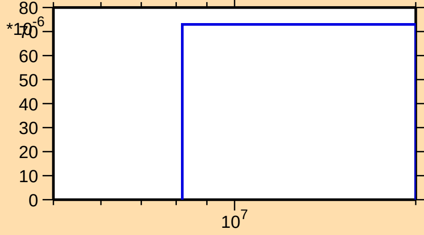
\sigma vs. E for ^{208}\text{Pb}(n,d)
