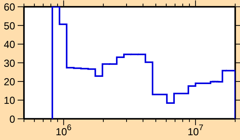
\Delta\sigma/\sigma vs. E for ^{214}\text{Pb}(n,\text{tot.})
