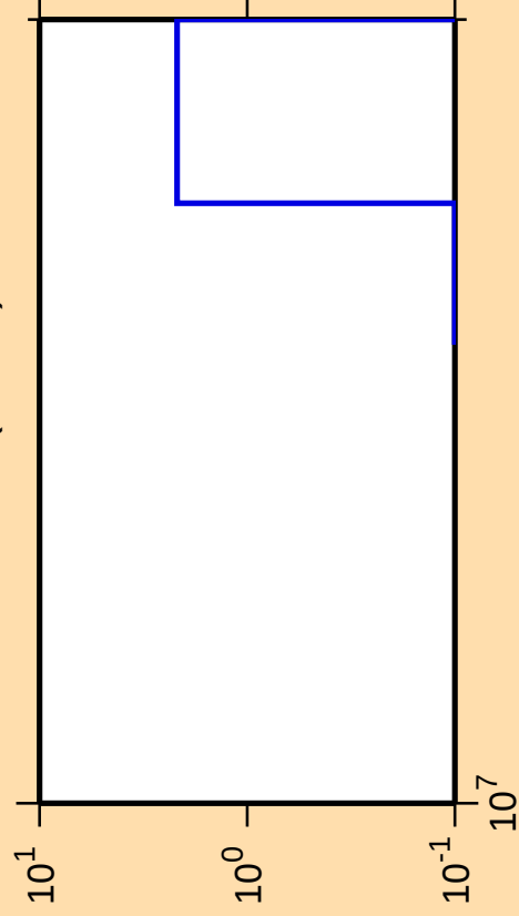
\Delta\sigma/\sigma vs. E for ^{214}\text{Pb}(\text{mt 11})
