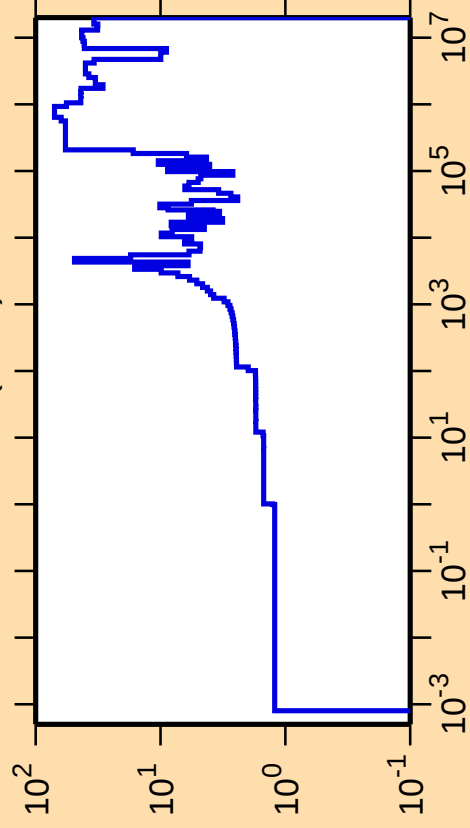
\Delta\sigma/\sigma vs. E for ^{214}\text{Pb}(n,\text{el.})
