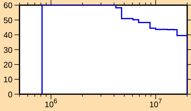
\Delta\sigma/\sigma vs. E for ^{214}\text{Pb}(n,n_1)
