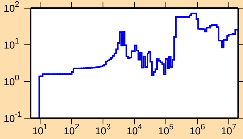
\Delta\sigma/\sigma vs. E for ^{214}\text{Pb}(n,\text{tot.})
