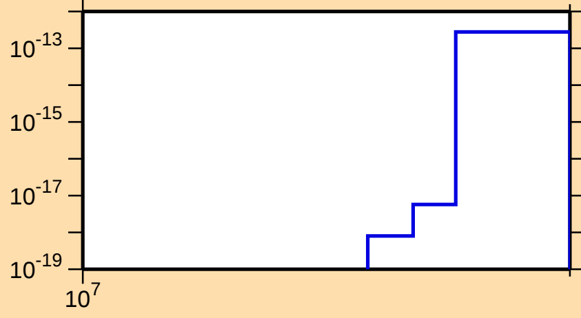
\sigma vs. E for ^{214}\text{Pb}(\text{mt 11})
