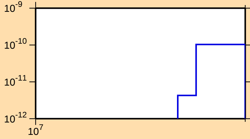
\sigma vs. E for ^{214}\text{Pb}(n,3n\alpha)
