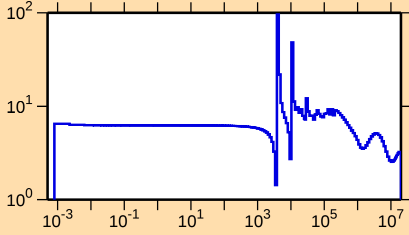
\sigma vs. E for ^{214}\text{Pb}(n,\text{el.})
