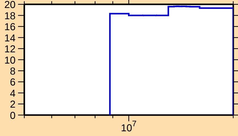
\Delta\sigma/\sigma vs. E for ^{214}\text{Pb}(n,\text{nonel.})
