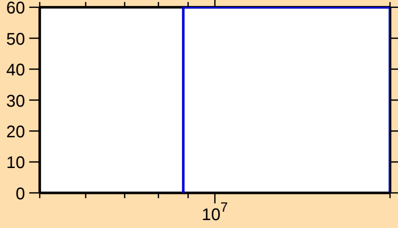
\Delta\sigma/\sigma vs. E for ^{214}\text{Pb}(n,n\text{cont.})
