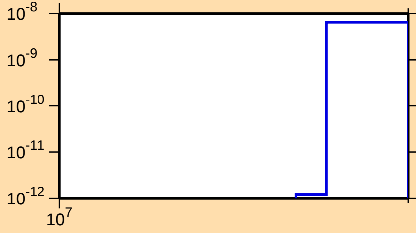
\sigma vs. E for ^{214}\text{Pb}(n,2np)
