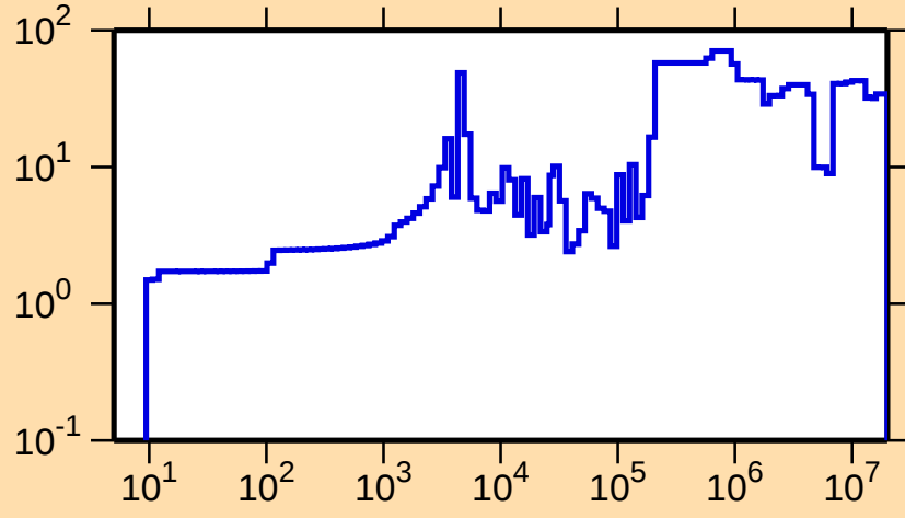
\Delta\sigma/\sigma vs. E for ^{214}\text{Pb}(n,\text{el.})
