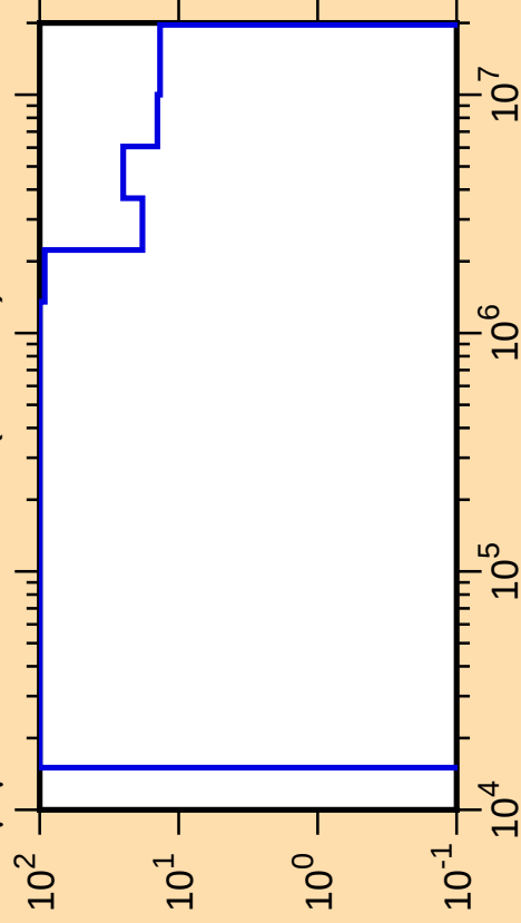
\Delta\mu/\mu vs. E for ^{214}\text{Pb}(\text{mt251})
