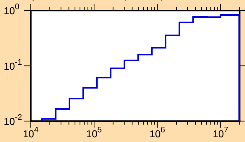
\mu vs. E for ^{214}\text{Pb}(\text{mt251})
