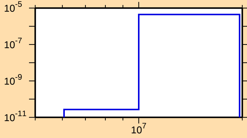
\sigma vs. E for ^{214}\text{Pb}(n,n\alpha)
