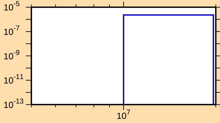
\sigma vs. E for ^{214}\text{Pb}(n,np)
