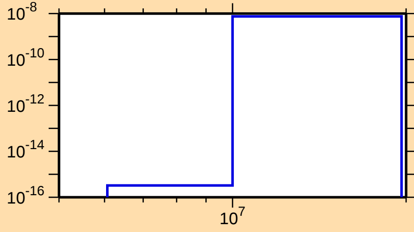
\sigma vs. E for ^{214}\text{Pb}(n,2n\alpha)
