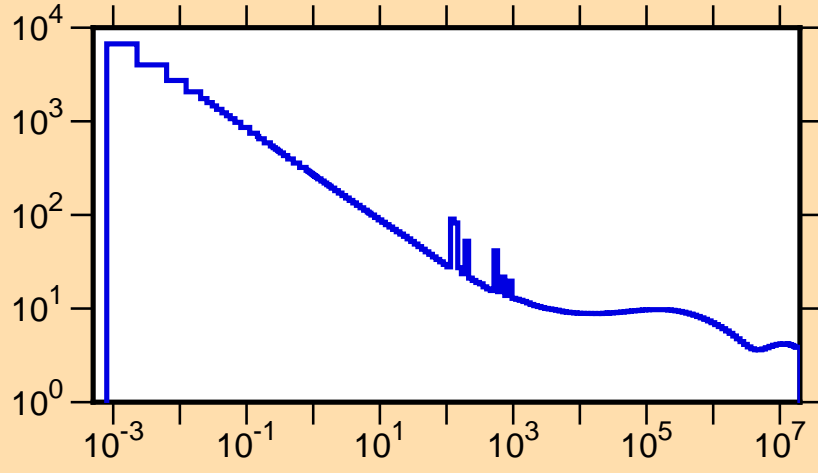
\sigma vs. E for ^{97}\text{Pd}(n,\text{tot.})
