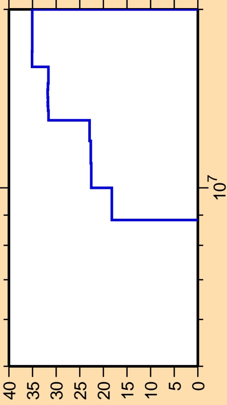
\Delta\sigma/\sigma vs. E for ^{97}\text{Pd}(n,p)
