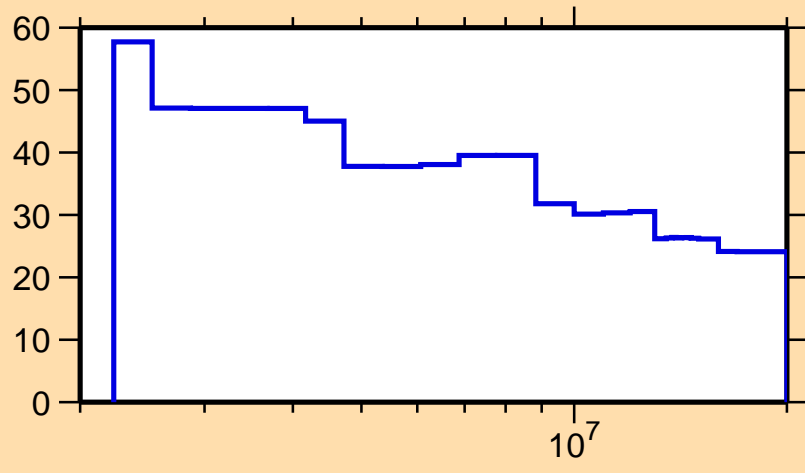
\Delta\sigma/\sigma vs. E for ^{97}\text{Pd}(n,n\text{cont.})
