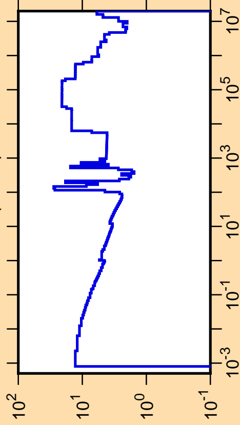
\Delta\sigma/\sigma vs. E for ^{97}\text{Pd}(n,\text{tot.})
