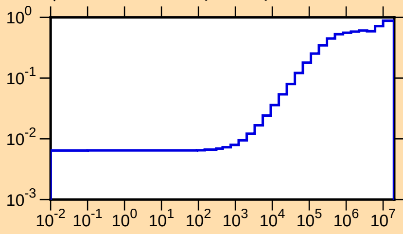
\mu vs. E for ^{113}\text{Pd}(\text{mt251})
