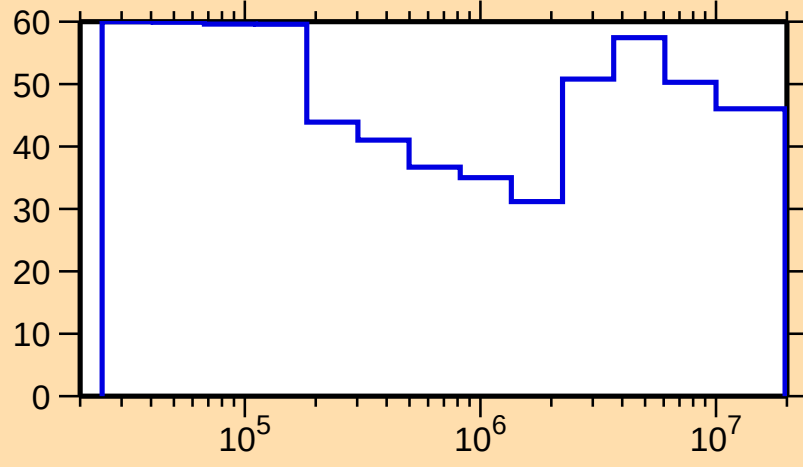
\Delta\sigma/\sigma vs. E for ^{113}\text{Pd}(n,n_1)
