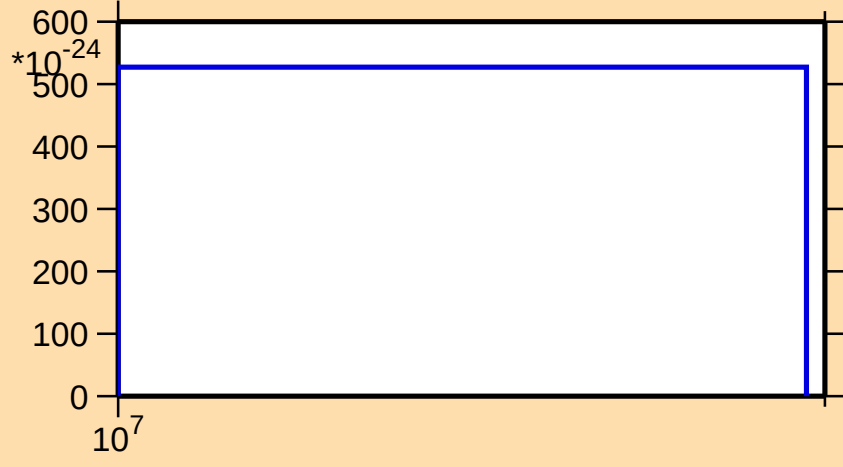
\sigma vs. E for ^{113}\text{Pd}(n,3n\alpha)
