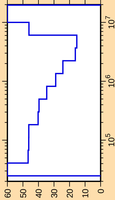
\Delta\sigma/\sigma vs. E for ^{113}\text{Pd}(n,\text{inel.})
