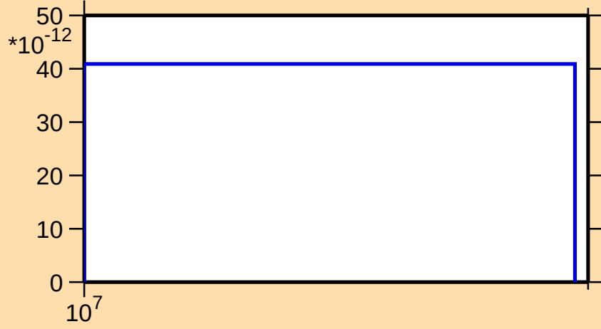
\sigma vs. E for ^{113}\text{Pd}(n,2n\alpha)
