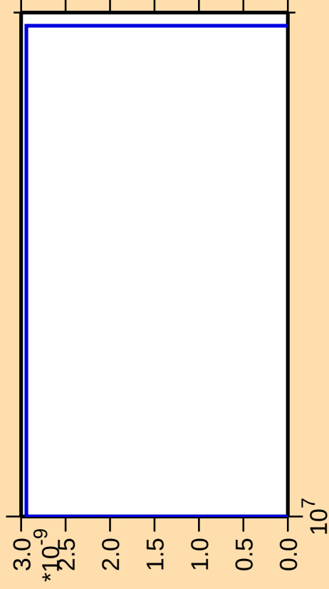
\Delta\sigma/\sigma vs. E for ^{113}\text{Pd}(n,3n\alpha)
