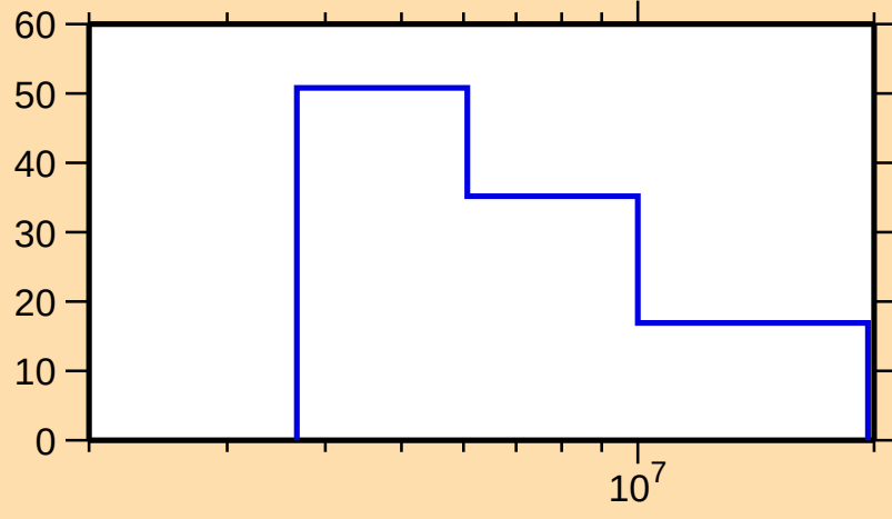
\Delta\sigma/\sigma vs. E for ^{113}\text{Pd}(n,2n)
