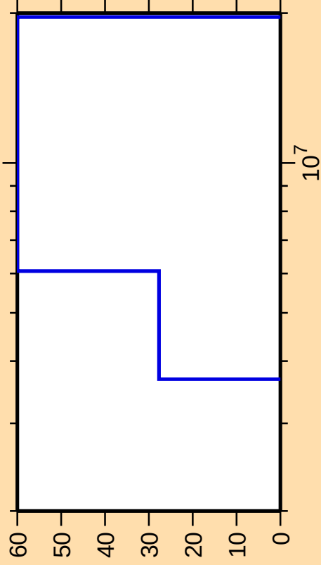
\Delta\sigma/\sigma vs. E for ^{113}\text{Pd}(n,n\text{cont.})
