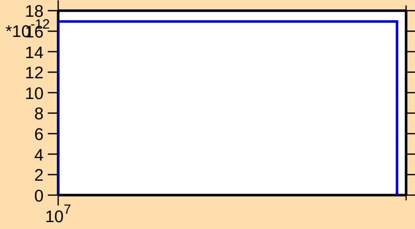
\sigma vs. E for ^{113}\text{Pd}(n,2np)
