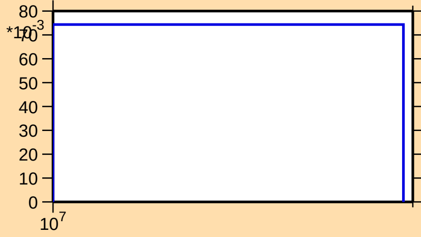
\sigma vs. E for ^{113}\text{Pd}(n,3n)
