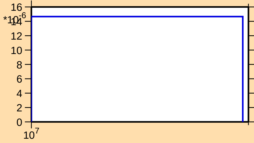
\sigma vs. E for ^{113}\text{Pd}(n,np)
