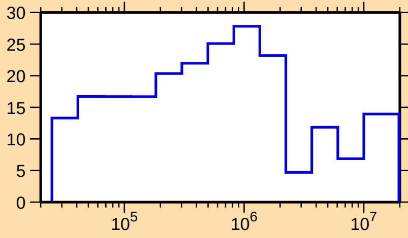
\Delta\sigma/\sigma vs. E for ^{113}\text{Pd}(n,\text{tot.})
