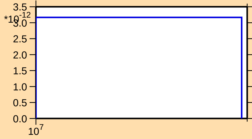
\sigma vs. E for ^{113}\text{Pd}(n,\text{nt})
