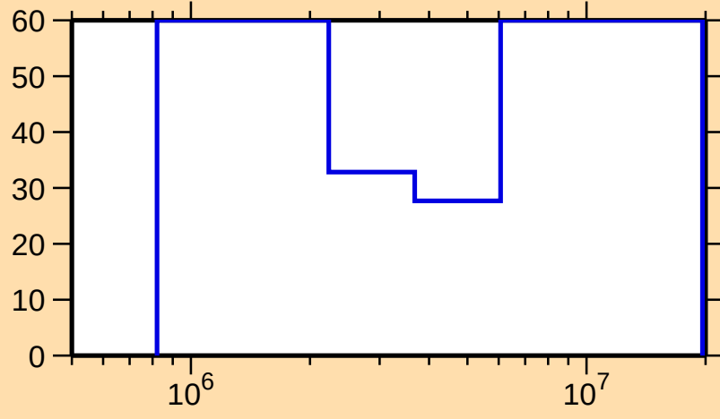
\Delta\sigma/\sigma vs. E for ^{113}\text{Pd}(n,n\text{cont.})
