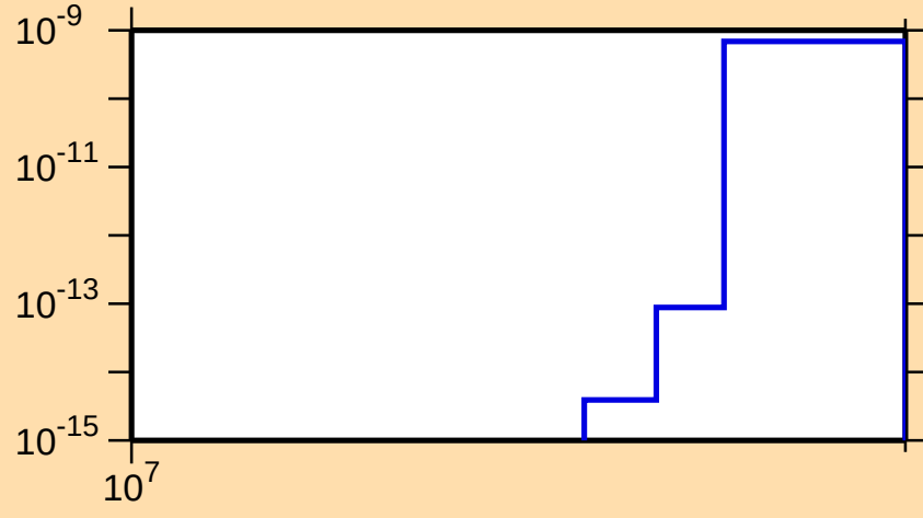
\sigma vs. E for ^{115}\text{Pd}(n,nt)
