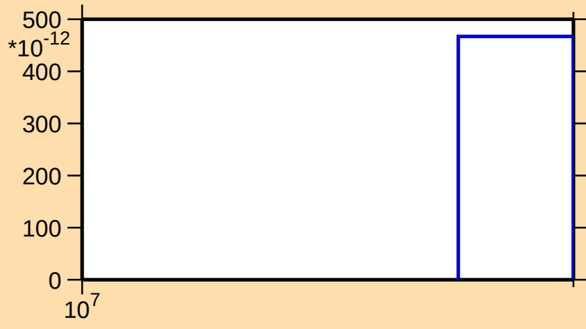
\sigma vs. E for ^{115}\text{Pd}(n,2np)
