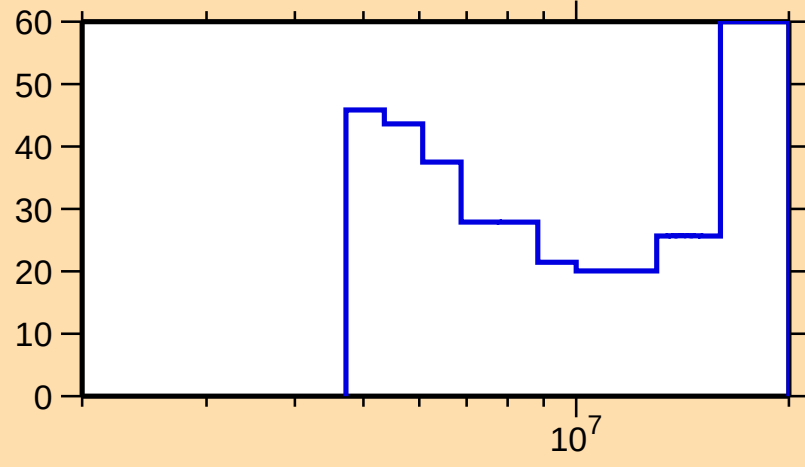
\Delta\sigma/\sigma vs. E for ^{115}\text{Pd}(n,2n)
