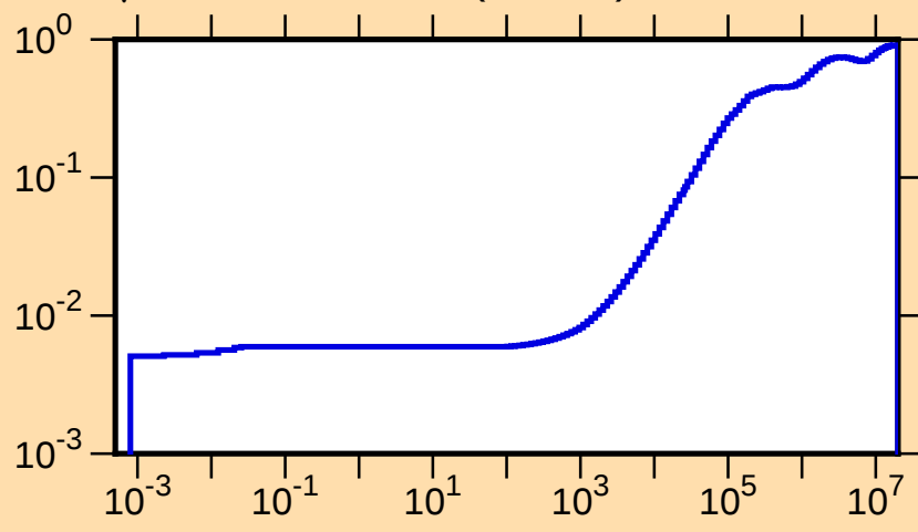
\mu vs. E for ^{134}\text{Pm}(\text{mt251})
