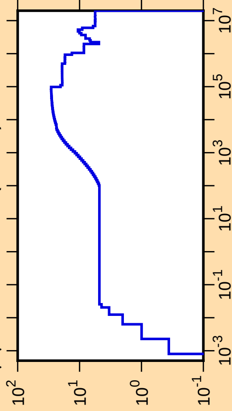
\Delta\mu/\mu vs. E for ^{134}\text{Pm}(\text{mt251})
