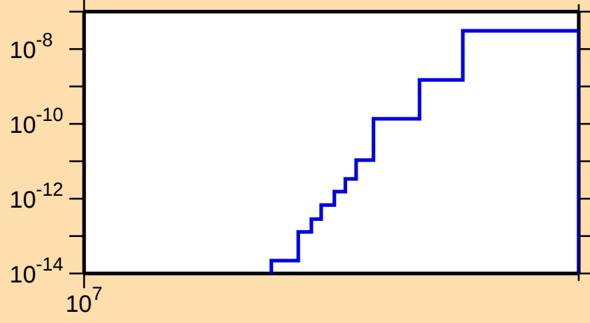
\sigma vs. E for ^{134}\text{Pm}(\text{mt } 34)
