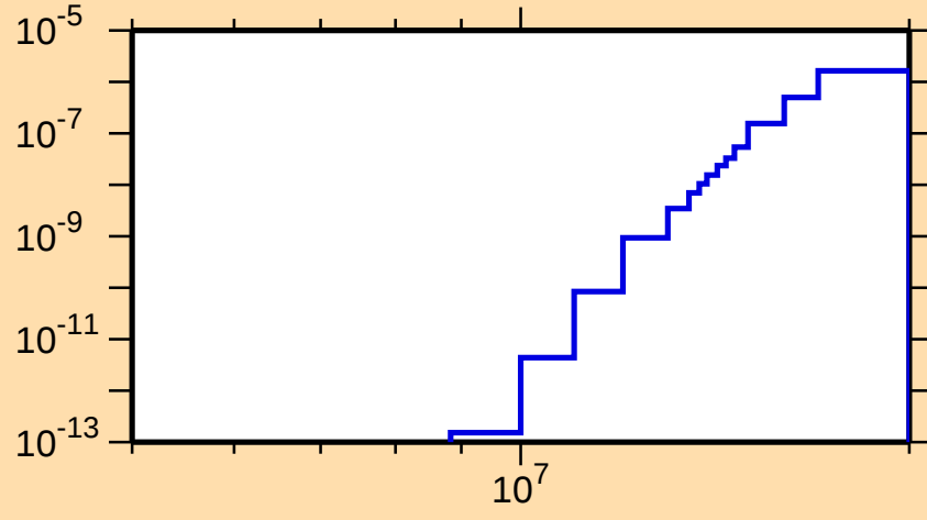
\sigma vs. E for ^{134}\text{Pm}(\text{mt117})
