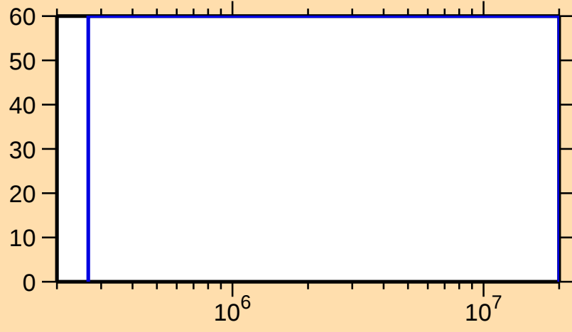
\Delta\sigma/\sigma vs. E for ^{134}\text{Pm}(n,n\text{cont.})
