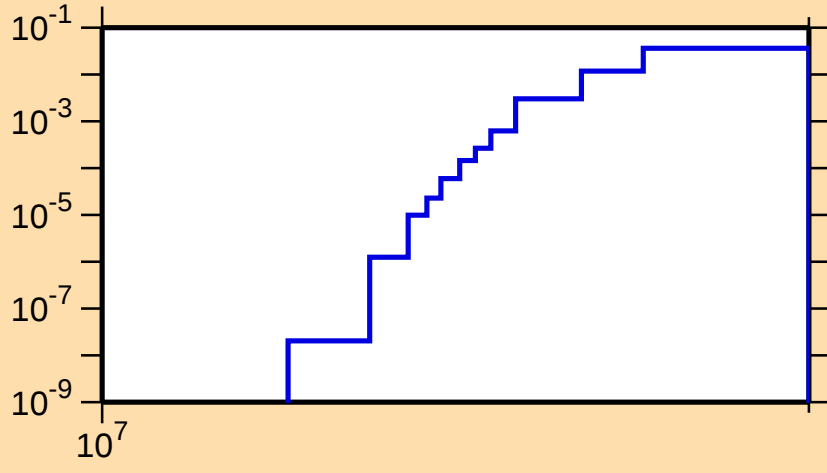
\sigma vs. E for ^{134}\text{Pm}(n,2np)
