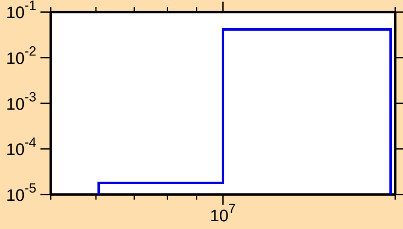
\sigma vs. E for ^{134}\text{Pm}(n,2n)
