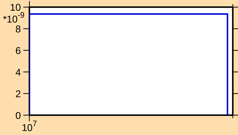
\sigma vs. E for ^{134}\text{Pm}(n,2n\alpha)
