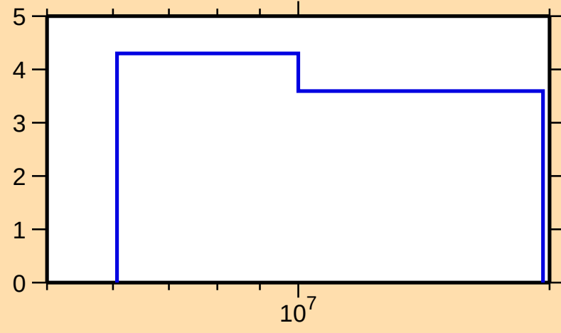
\Delta\sigma/\sigma vs. E for ^{134}\text{Pm}(n,\text{nonel.})
