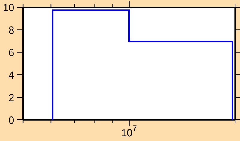
\Delta\sigma/\sigma vs. E for ^{134}\text{Pm}(n,\text{el.})
