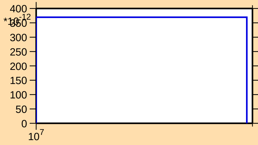
\sigma vs. E for ^{134}\text{Pm} (mt 34)
