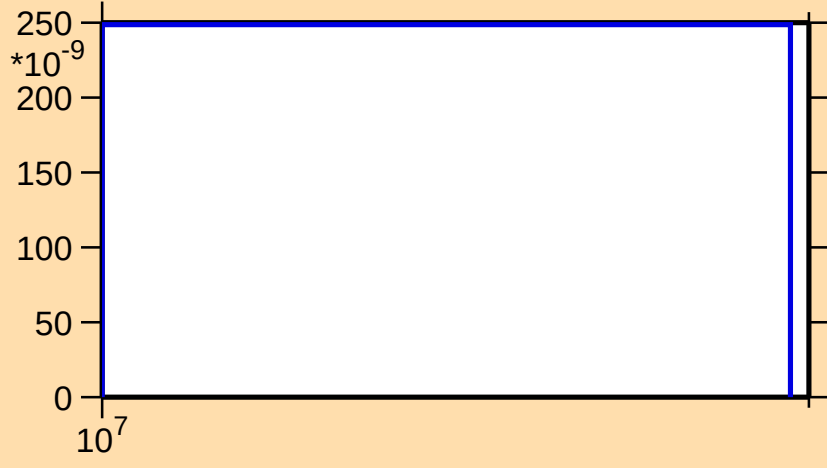
\sigma vs. E for ^{134}\text{Pm}(n,\text{pt})
