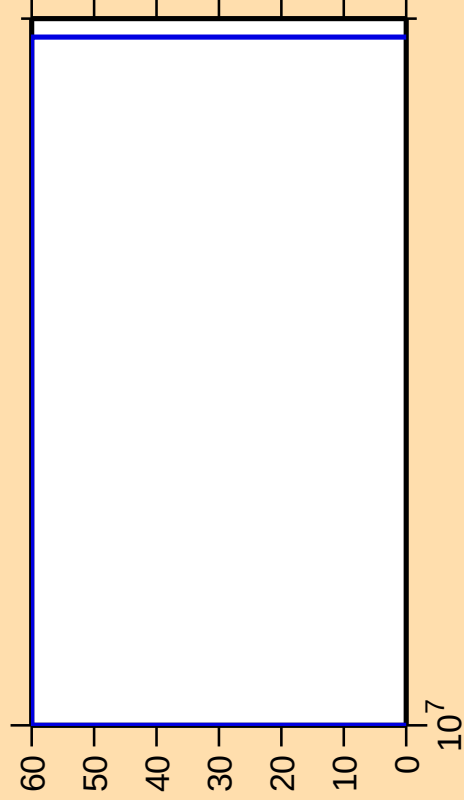
\Delta\sigma/\sigma vs. E for ^{134}\text{Pm}(n,\text{nt})
