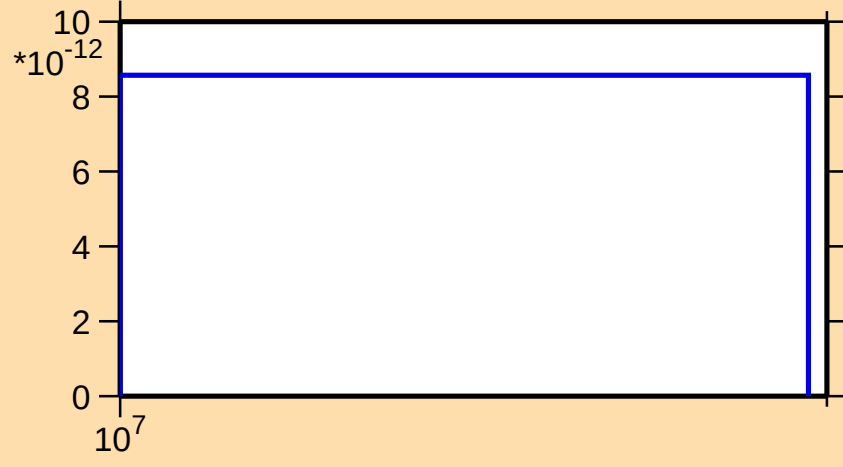
\sigma vs. E for ^{134}\text{Pm}(n,\text{nt})
