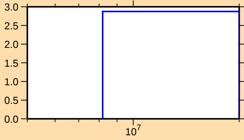
\Delta\sigma/\sigma vs. E for ^{134}\text{Pm}(n,\text{tot.})
