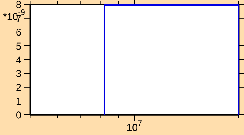
\sigma vs. E for ^{134}\text{Pm}(n,2n\alpha)
