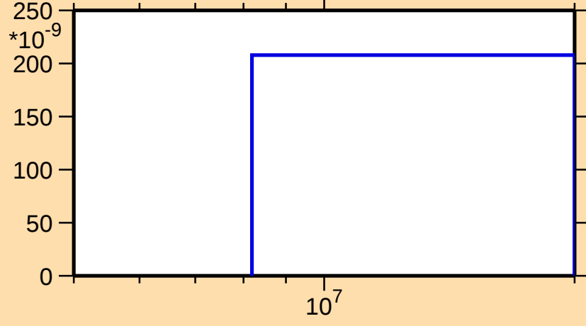
\sigma vs. E for ^{134}\text{Pm}(n,\text{pt})
