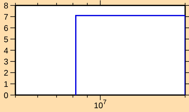
\Delta\sigma/\sigma vs. E for ^{134}\text{Pm}(n,\text{el.})
