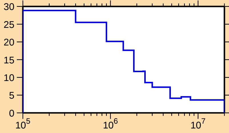
\Delta\sigma/\sigma vs. E for ^{134}\text{Pm}(n,\text{nonel.})
