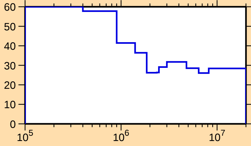
\Delta\sigma/\sigma vs. E for ^{134}\text{Pm}(n,n_1)
