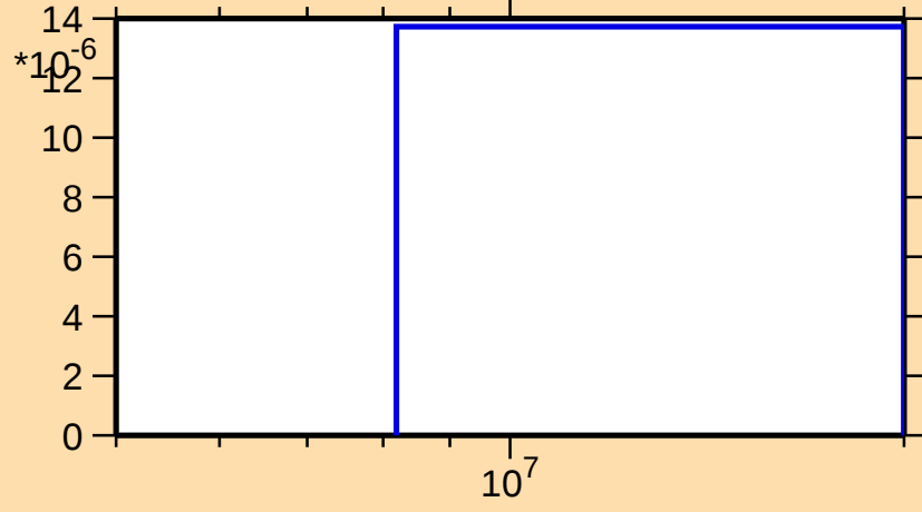
\sigma vs. E for ^{134}\text{Pm} (mt 45)
