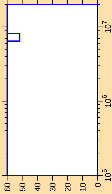
\Delta\sigma/\sigma vs. E for ^{134}\text{Pm}(n,\gamma)
