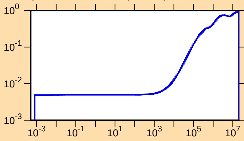
\mu vs. E for ^{139}\text{Pm}(\text{mt251})
