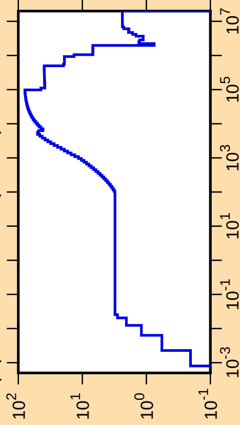
\Delta\mu/\mu vs. E for ^{139}\text{Pm}(\text{mt251})
