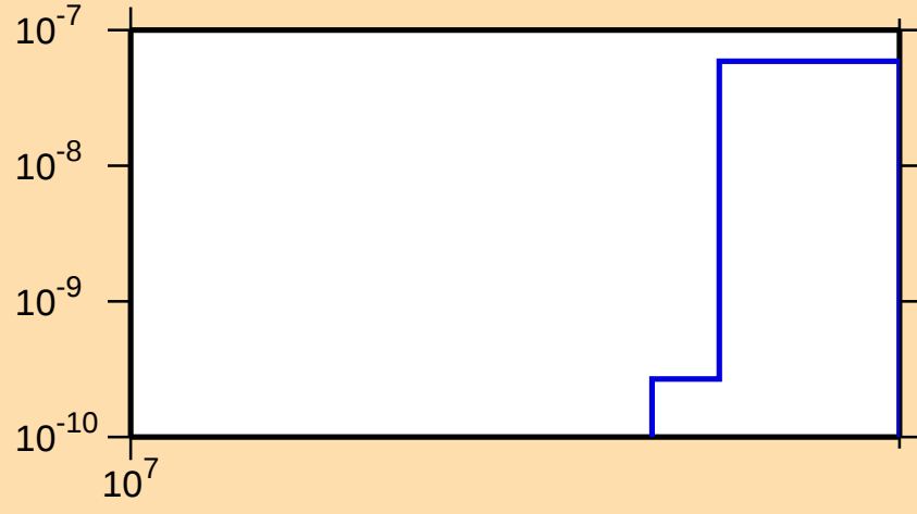
\sigma vs. E for ^{139}\text{Pm}(n,2n\alpha)
