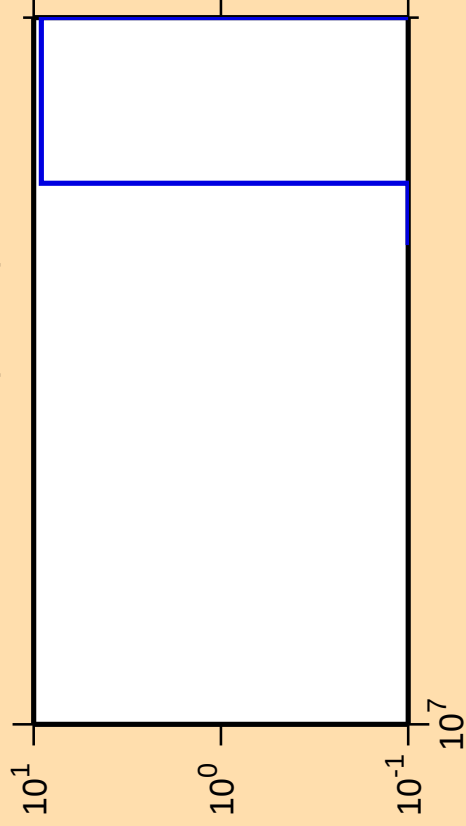
\Delta\sigma/\sigma vs. E for ^{139}\text{Pm} (mt 34)
