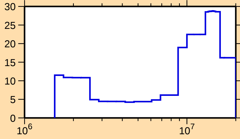
\Delta\sigma/\sigma vs. E for ^{139}\text{Pm}(n,n\text{cont.})
