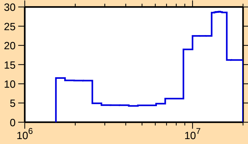
\Delta\sigma/\sigma vs. E for ^{139}\text{Pm}(n,n\text{cont.})
