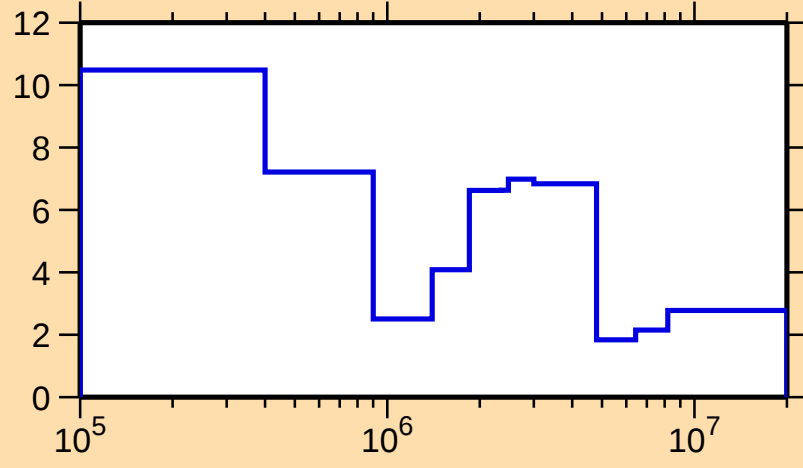
\Delta\sigma/\sigma vs. E for ^{139}\text{Pm}(n,\text{el.})
