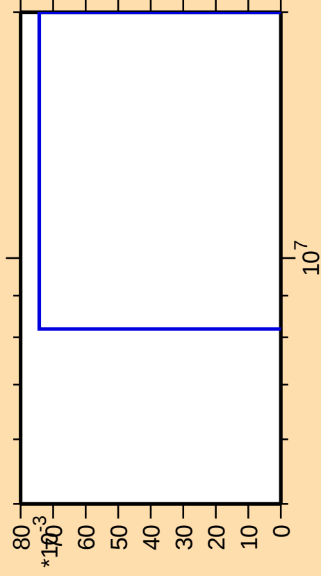
\Delta\sigma/\sigma vs. E for ^{139}\text{Pm}(\text{mt } 34)
