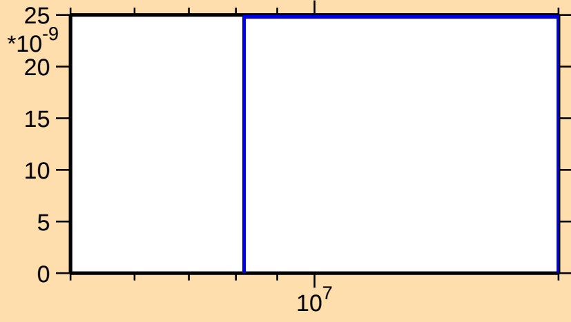
\sigma vs. E for ^{139}\text{Pm}(\text{mt } 45)
