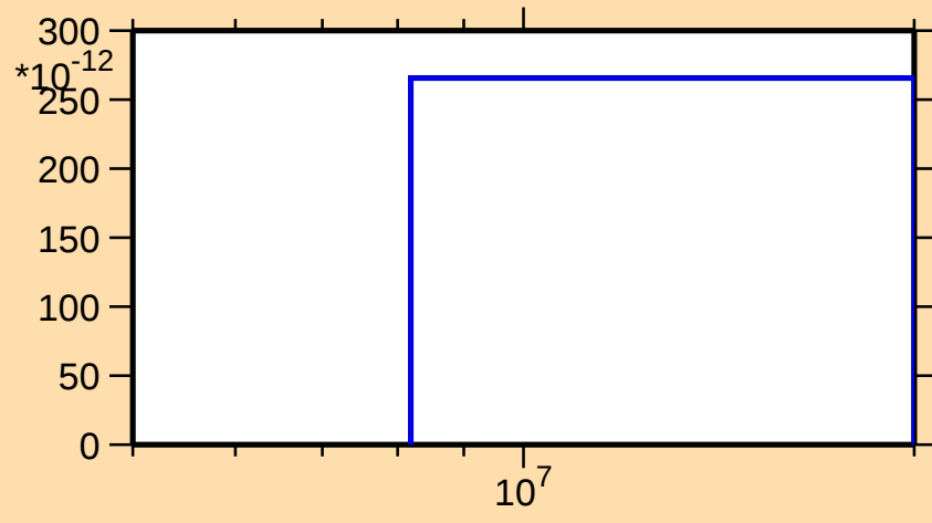
\sigma vs. E for ^{139}\text{Pm}(\text{mt117})
