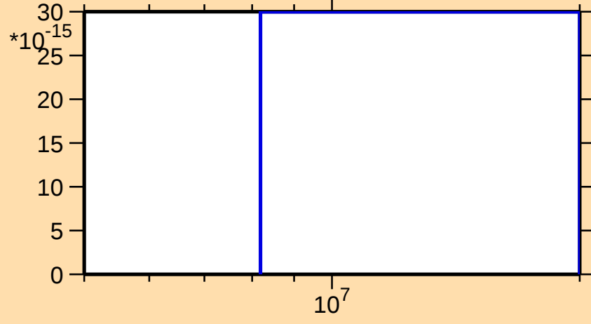
\sigma vs. E for ^{139}\text{Pm}(\text{mt } 34)
