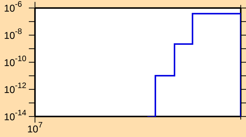
\sigma vs. E for ^{144}\text{Pm}(n,nt)
