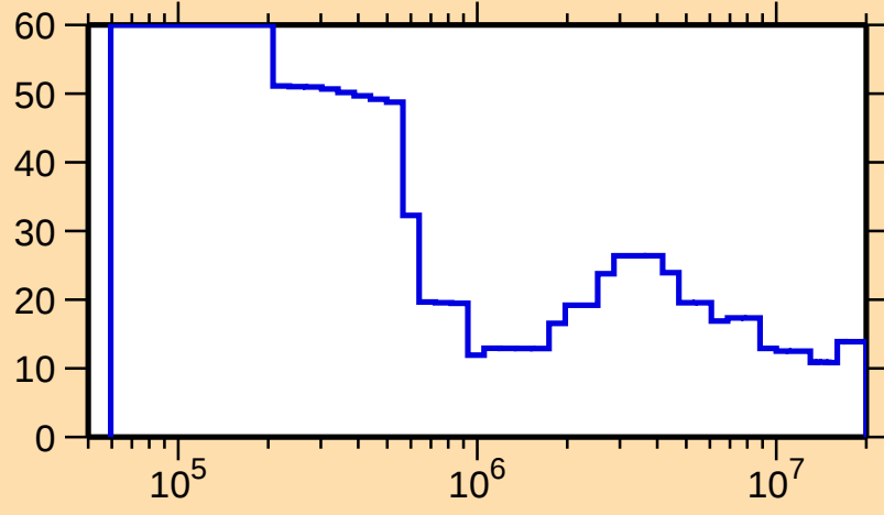
\Delta\sigma/\sigma vs. E for ^{144}\text{Pm}(n,\text{el.})
