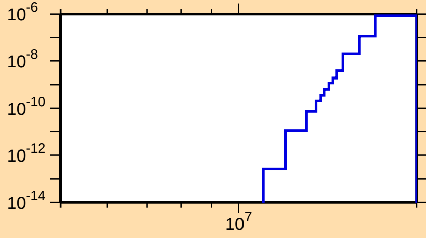
\sigma vs. E for ^{144}\text{Pm}(n,\text{He}3)
