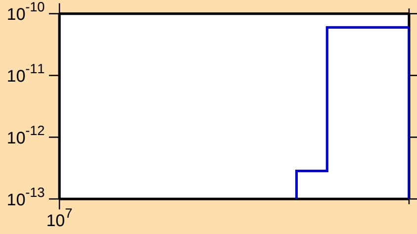
\sigma vs. E for ^{144}\text{Pm}(n,\text{pt})
