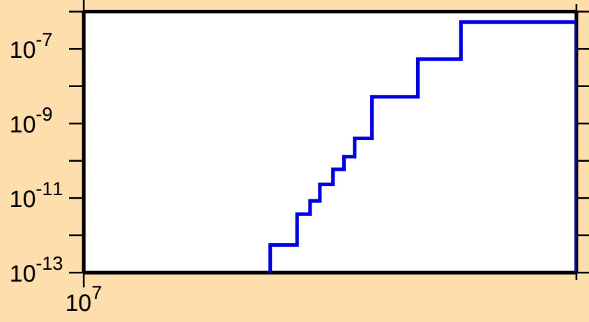
\sigma vs. E for ^{144}\text{Pm}(n,2n\alpha)
