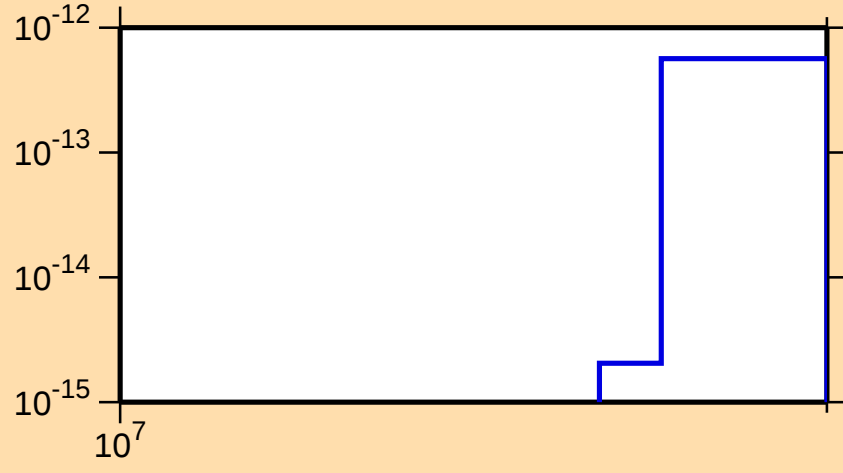
\sigma vs. E for ^{144}\text{Pm}(n,\text{pd})
