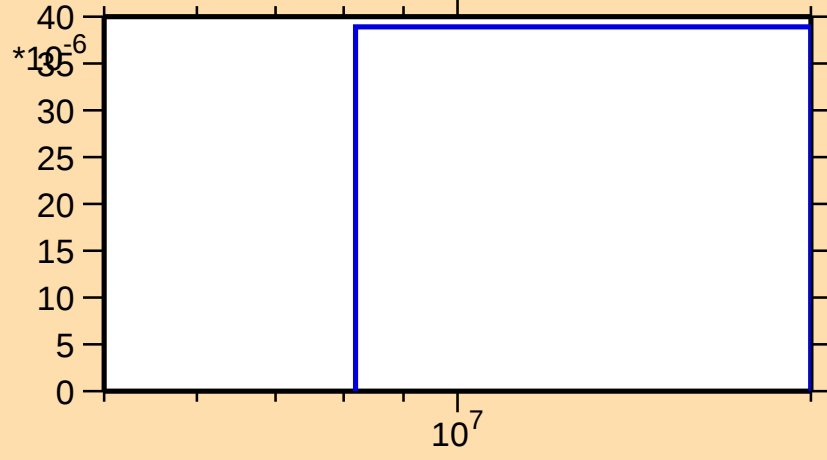
\sigma vs. E for ^{144}\text{Pm}(n,2np)
