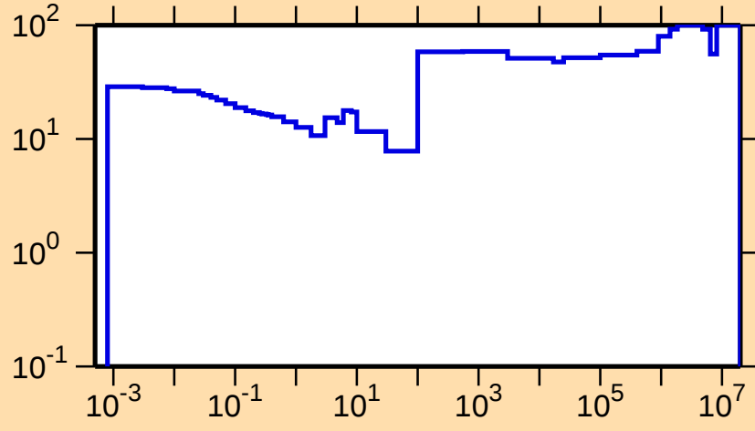
\Delta\sigma/\sigma vs. E for ^{144}\text{Pm}(n,\gamma)
