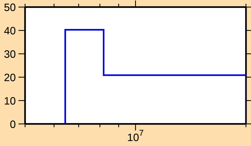
\Delta\sigma/\sigma vs. E for ^{144}\text{Pm}(n,2n)
