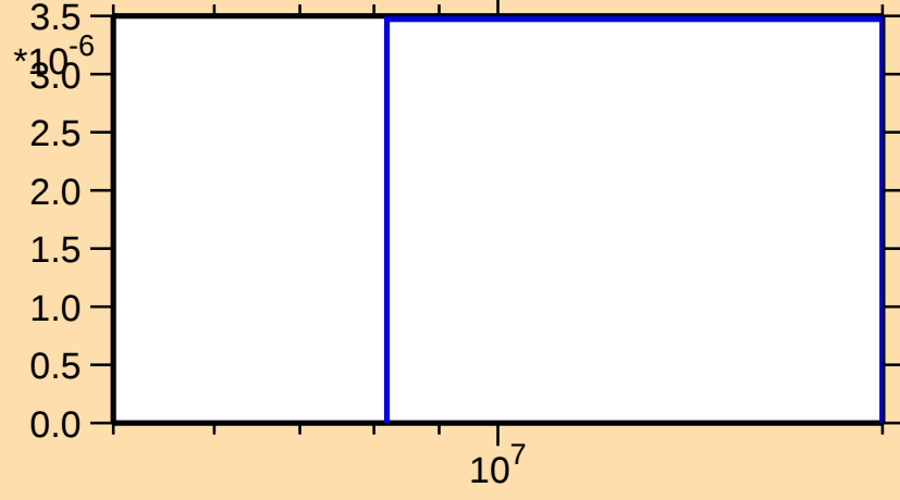
\sigma vs. E for ^{144}\text{Pm}(n,\text{nd})
