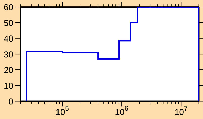
\Delta\sigma/\sigma vs. E for ^{144}\text{Pm}(n,n_1)
