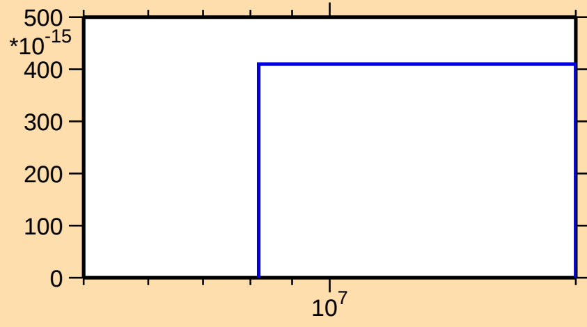
\sigma vs. E for ^{144}\text{Pm}(\text{mt } 45)
