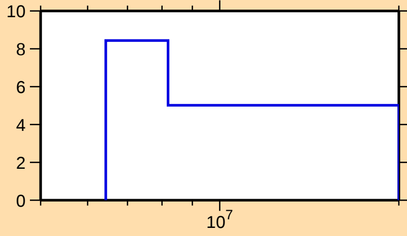
\Delta\sigma/\sigma vs. E for ^{144}\text{Pm}(n,\text{tot.})
