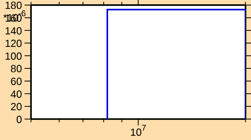
\sigma vs. E for ^{144}\text{Pm}(n,3n)
