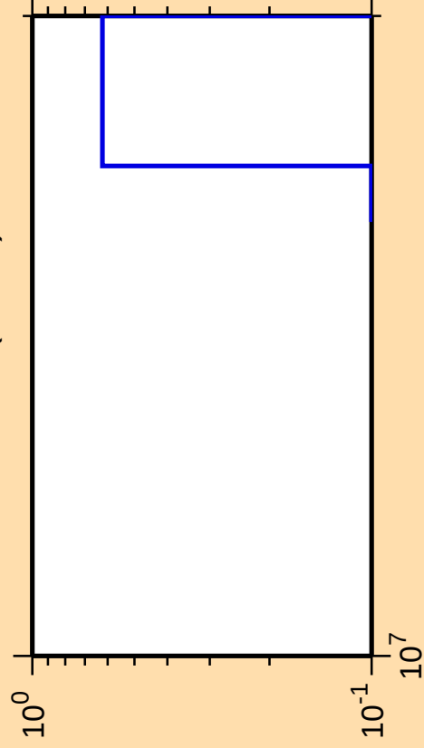
\Delta\sigma/\sigma vs. E for ^{145}\text{Pm} (mt 34)
