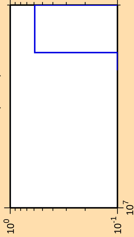
\Delta\sigma/\sigma vs. E for ^{145}\text{Pm} (mt 11)
