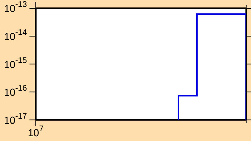
\sigma vs. E for ^{145}\text{Pm}(n,\text{pd})
