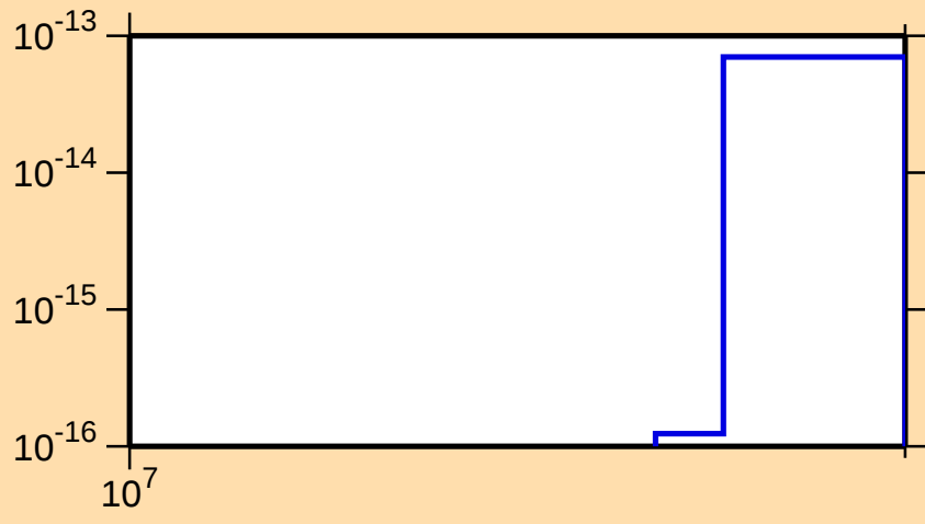
\sigma vs. E for ^{145}\text{Pm} (mt 11)
