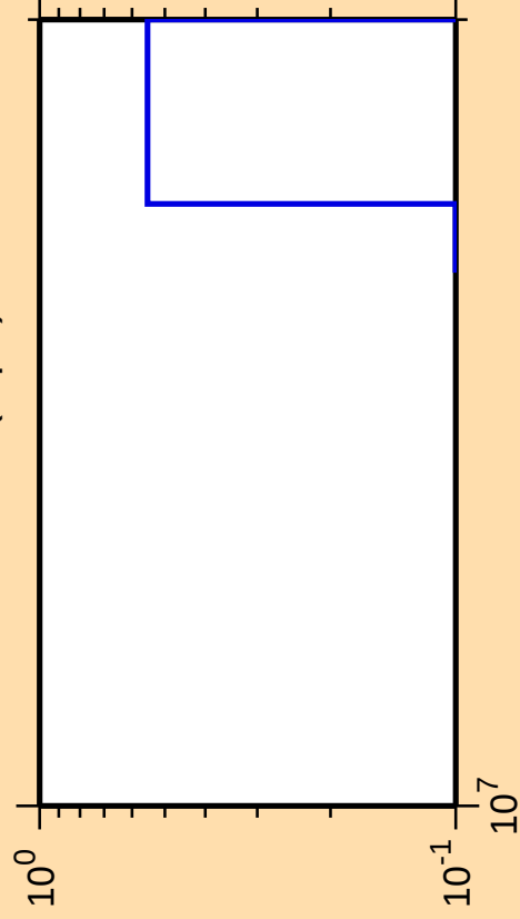
\Delta\sigma/\sigma vs. E for ^{145}\text{Pm}(n,\text{pd})
