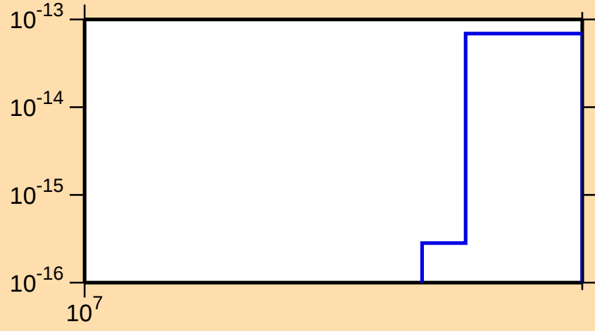
\sigma vs. E for ^{145}\text{Pm} (mt 34)
