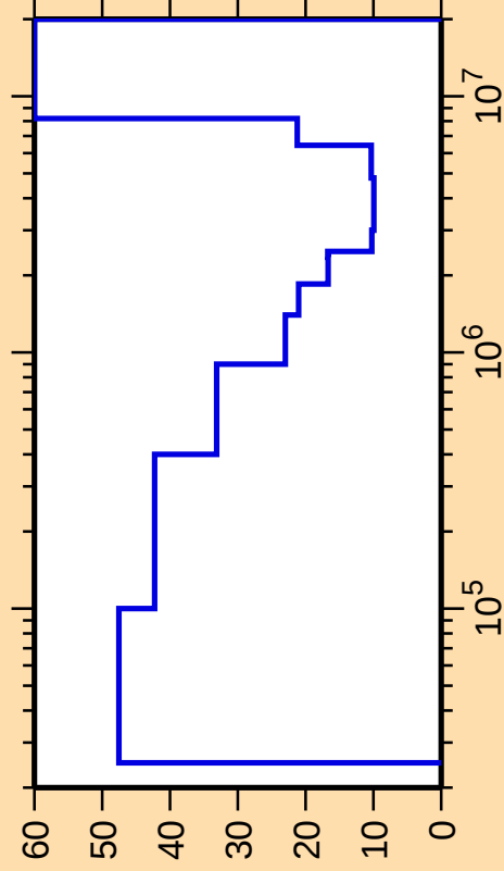
\Delta\sigma/\sigma vs. E for ^{145}\text{Pm}(n,\text{inel.})
