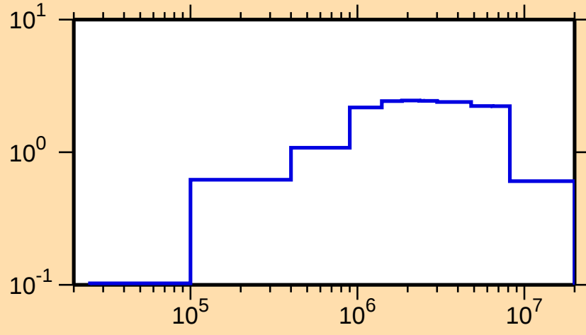
\sigma vs. E for ^{145}\text{Pm}(n,\text{inel.})
