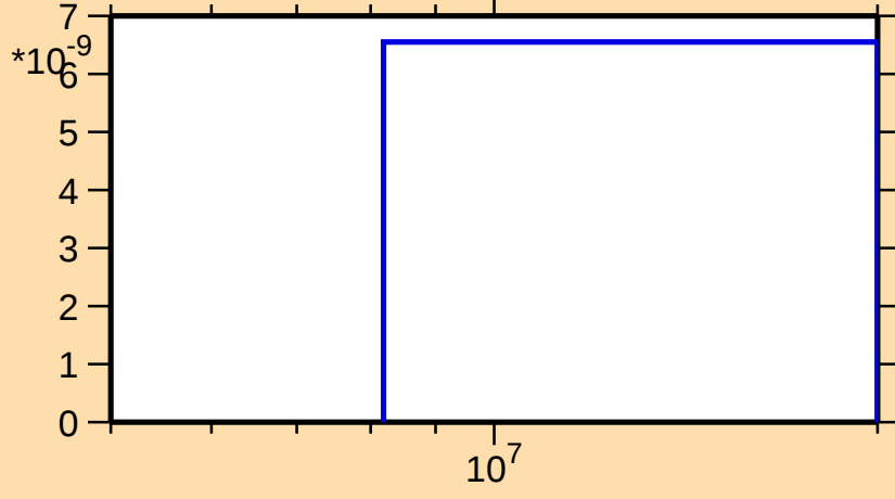
\sigma vs. E for ^{145}\text{Pm}(n,2n\alpha)
