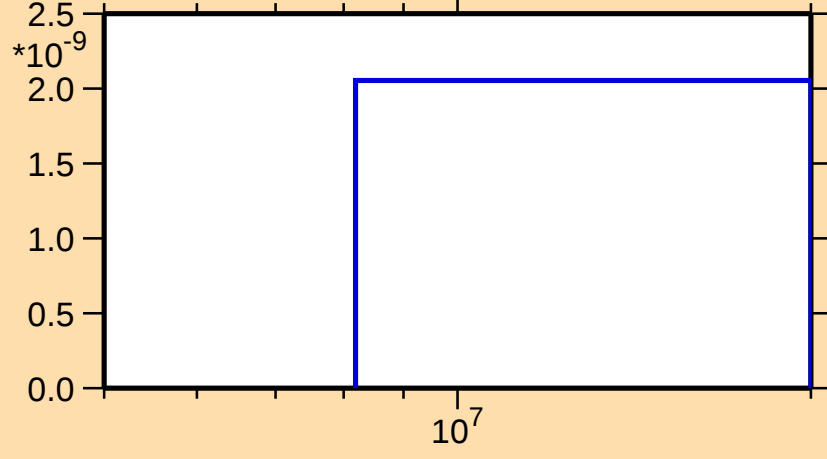
\sigma vs. E for ^{145}\text{Pm}(n,p\alpha)
