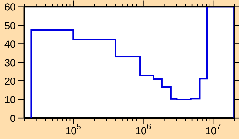
\Delta\sigma/\sigma vs. E for ^{145}\text{Pm}(n,\text{inel.})
