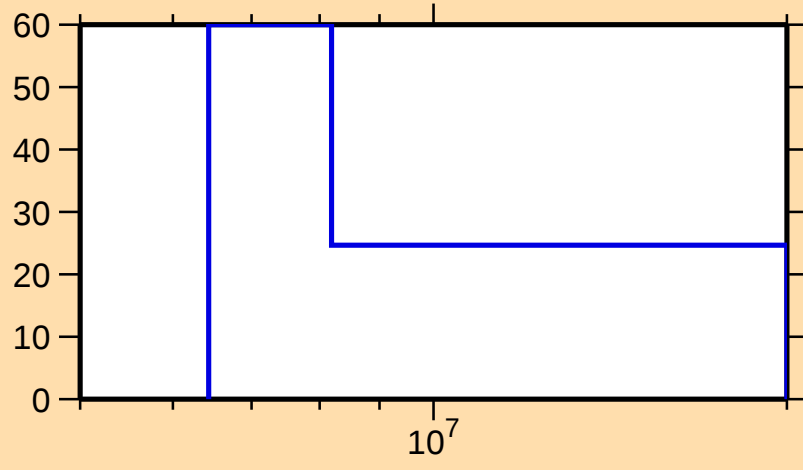
\Delta\sigma/\sigma vs. E for ^{145}\text{Pm}(n,2n)
