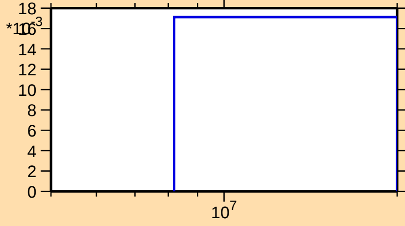
\sigma vs. E for ^{145}\text{Pm}(n,3n)
