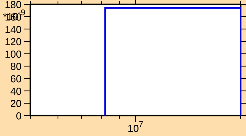
\sigma vs. E for ^{145}\text{Pm}(n,nt)
