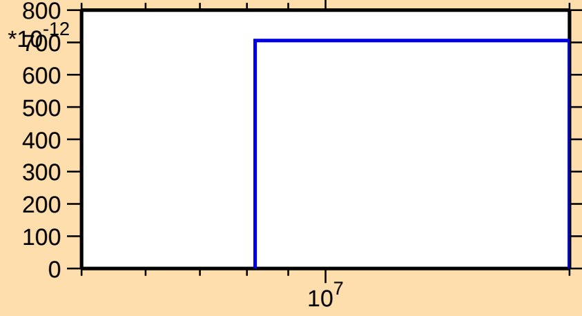
\sigma vs. E for ^{145}\text{Pm}(n,\text{He}3)
