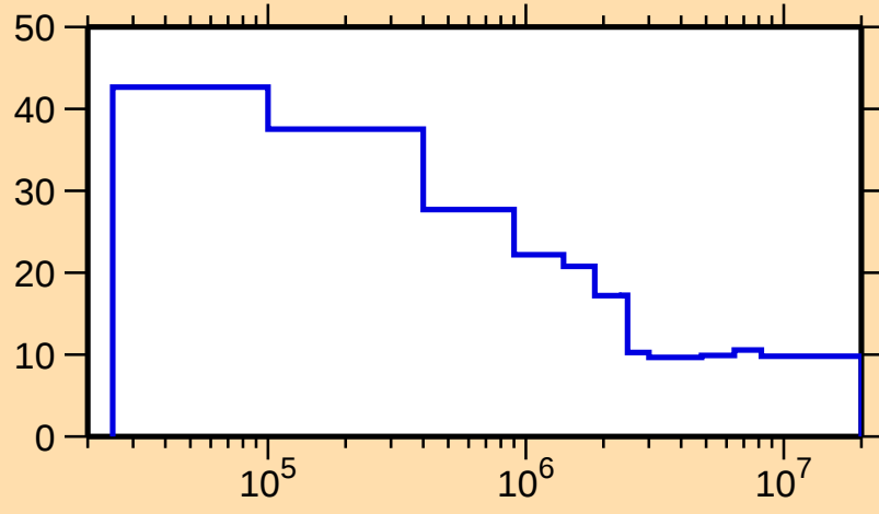
\Delta\sigma/\sigma vs. E for ^{145}\text{Pm}(n,\text{nonel.})
