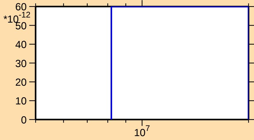
\sigma vs. E for ^{145}\text{Pm}(\text{mt } 45)
