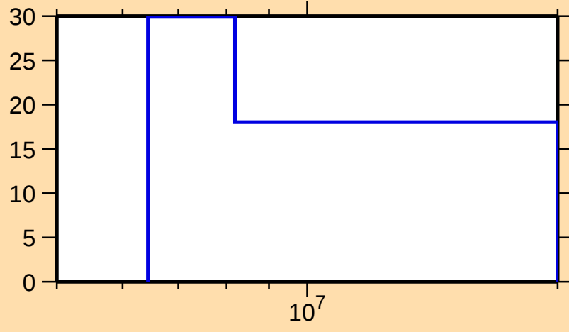
\Delta\sigma/\sigma vs. E for ^{145}\text{Pm}(n,\text{el.})
