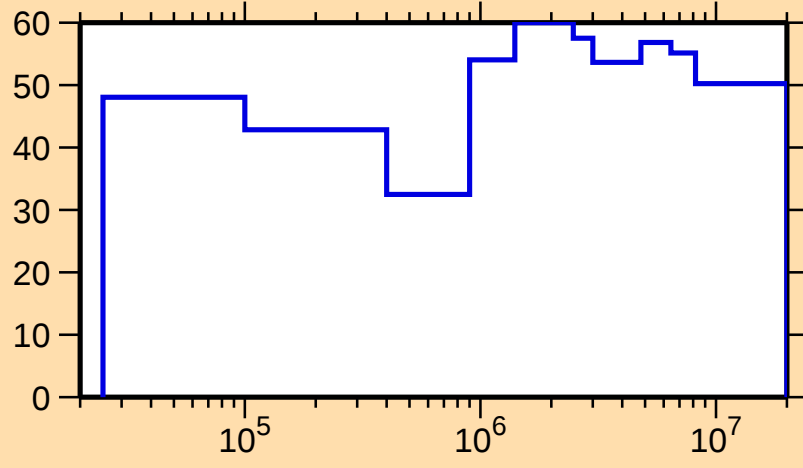
\Delta\sigma/\sigma vs. E for ^{145}\text{Pm}(n,n_1)
