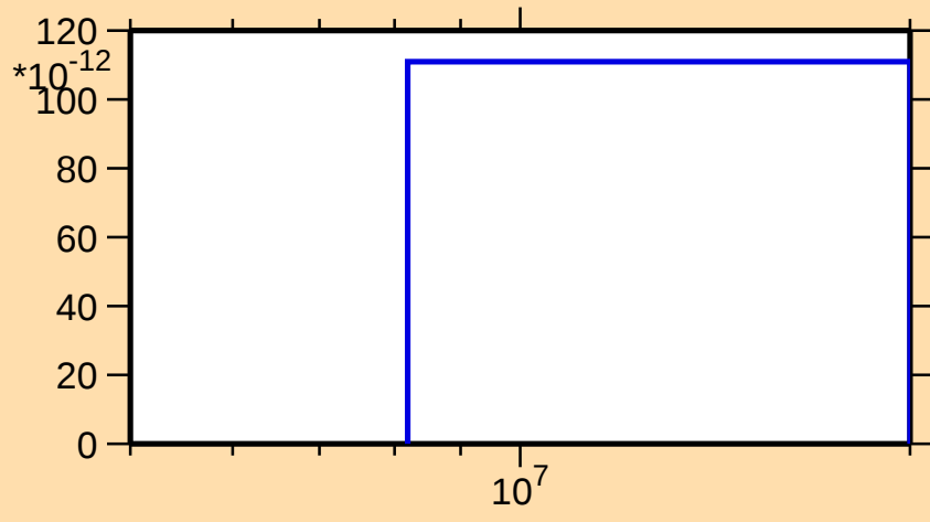
\sigma vs. E for ^{145}\text{Pm}(\text{mt117})
