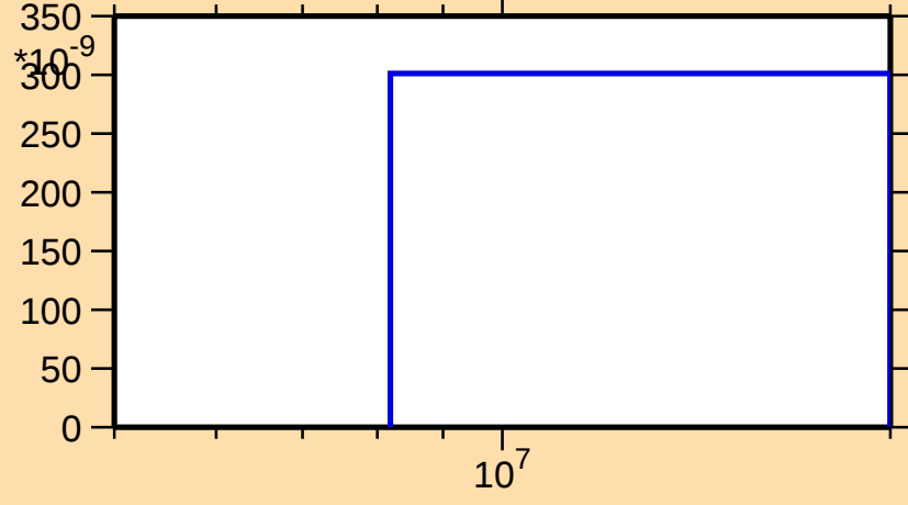
\sigma vs. E for ^{145}\text{Pm}(n,2np)
