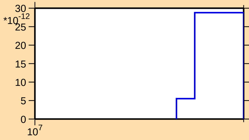
\sigma vs. E for ^{147}\text{Pm}(\text{mt117})
