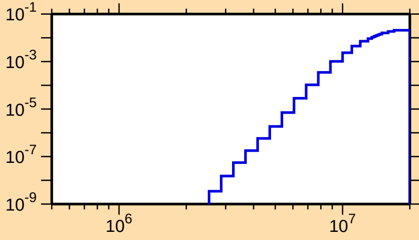
\sigma vs. E for ^{147}\text{Pm}(n,p)
