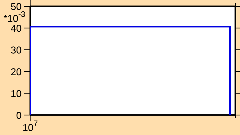
\sigma vs. E for ^{147}\text{Pm}(n,3n)
