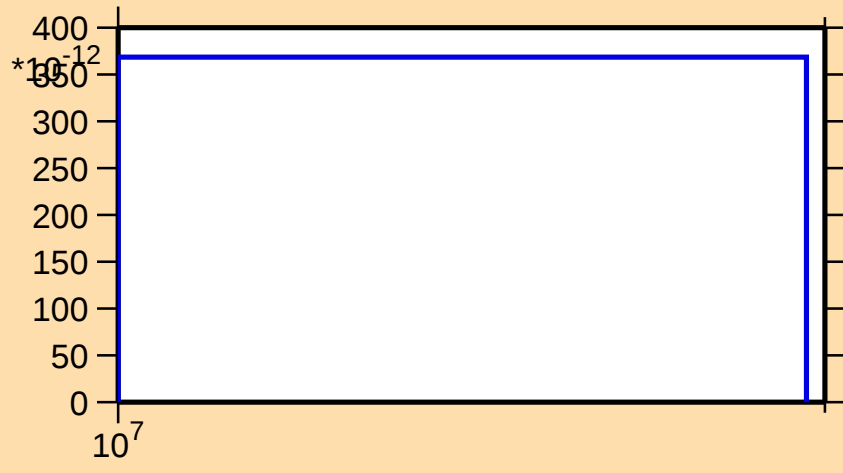
\sigma vs. E for ^{147}\text{Pm}(n,\text{He}3)
