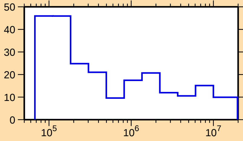
\Delta\sigma/\sigma vs. E for ^{147}\text{Pm}(n,\text{tot.})
