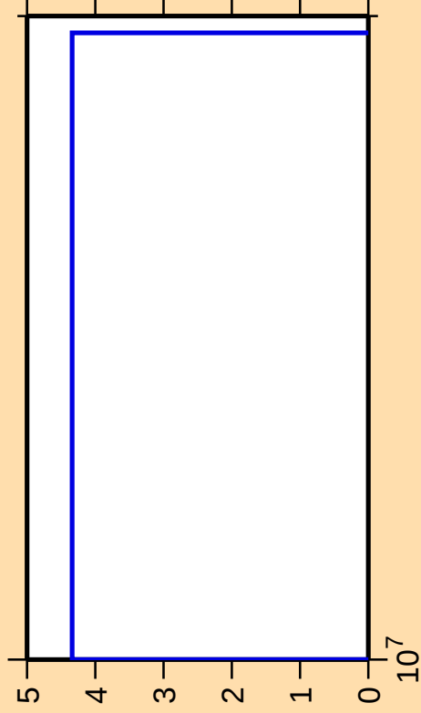
\Delta\sigma/\sigma vs. E for ^{147}\text{Pm}(\text{mt117})
