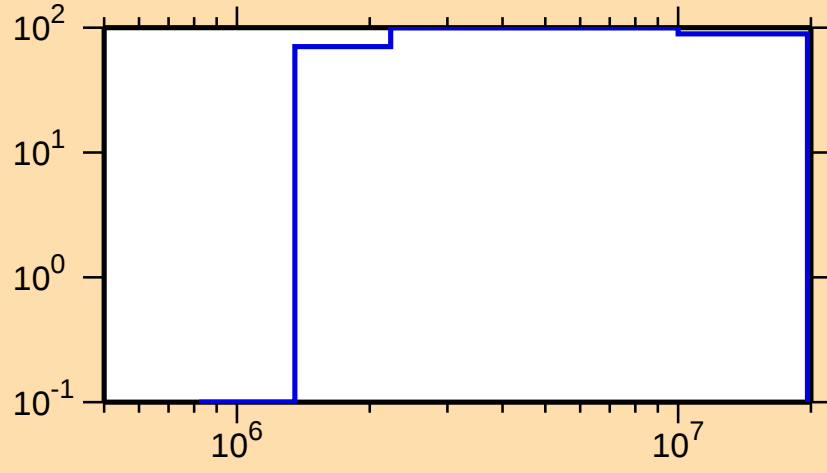
\Delta\sigma/\sigma vs. E for ^{147}\text{Pm}(n,p)
