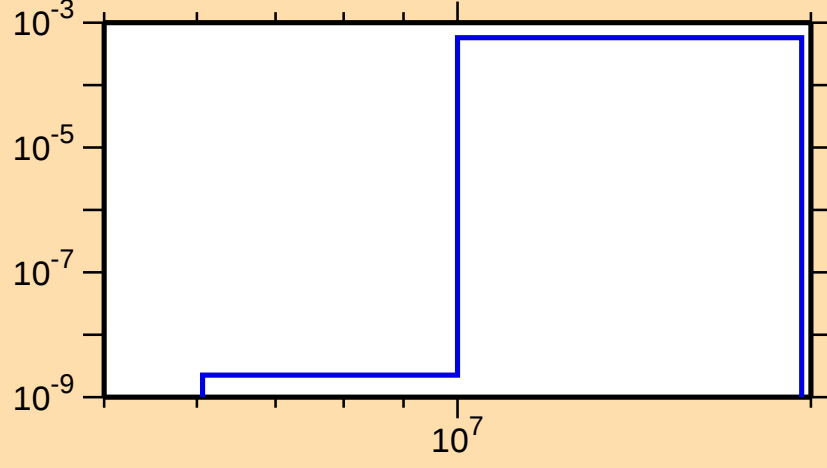
\sigma vs. E for ^{147}\text{Pm}(n,t)
