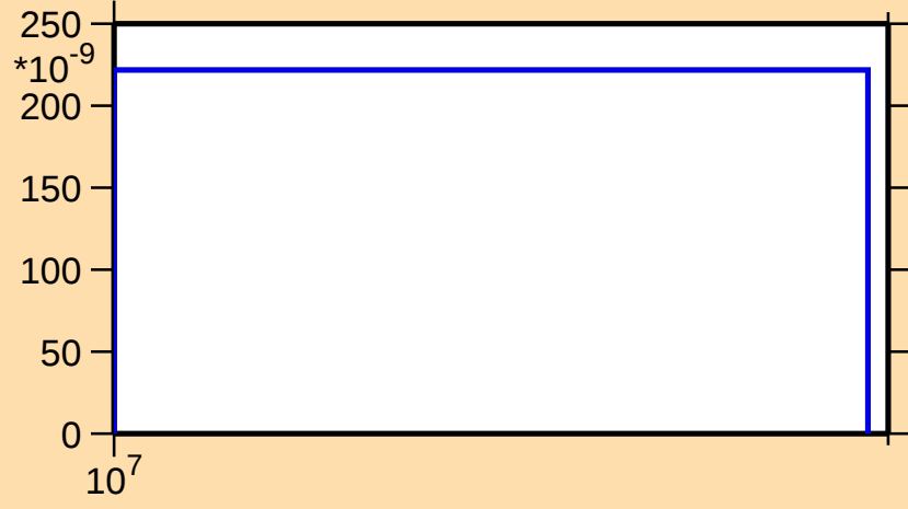
\sigma vs. E for ^{147}\text{Pm}(n,\text{nt})
