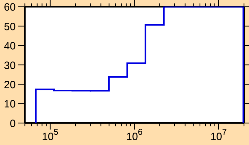
\Delta\sigma/\sigma vs. E for ^{147}\text{Pm}(n,n_1)
