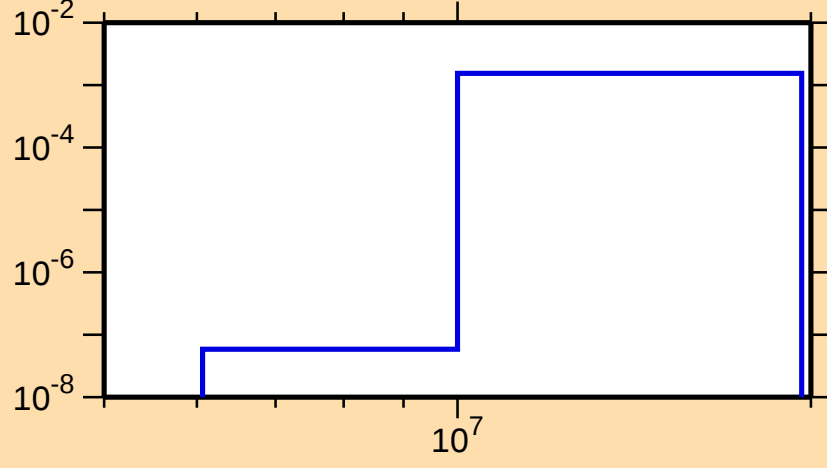
\sigma vs. E for ^{147}\text{Pm}(n,np)
