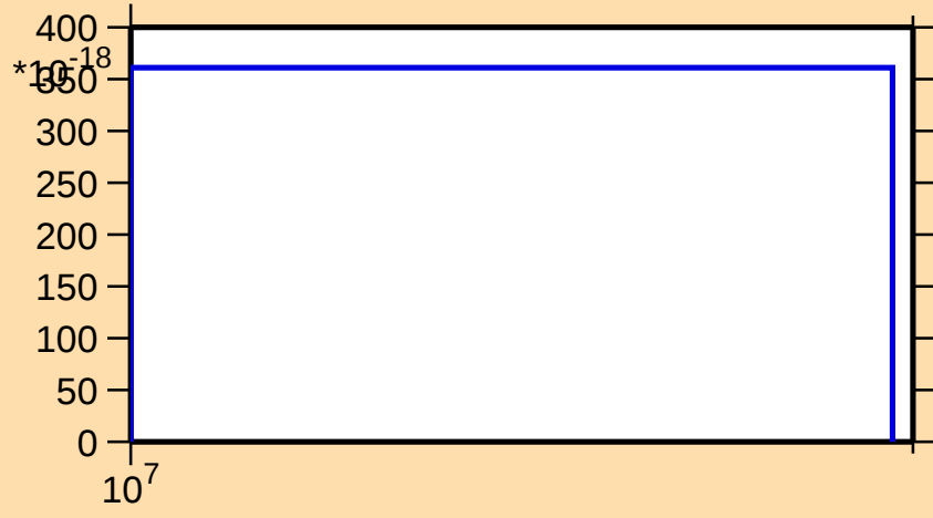
\sigma vs. E for ^{147}\text{Pm} (mt 11)
