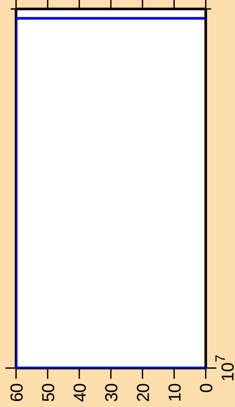
\Delta\sigma/\sigma vs. E for ^{147}\text{Pm}(n,\text{nd})
