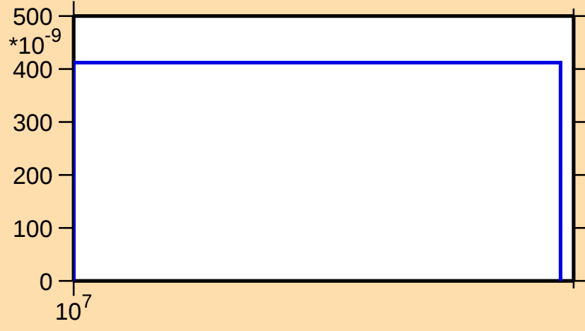
\sigma vs. E for ^{147}\text{Pm}(n,\text{nd})
