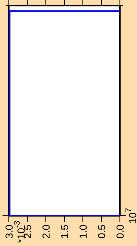
\Delta\sigma/\sigma vs. E for ^{147}\text{Pm} (mt 11)
