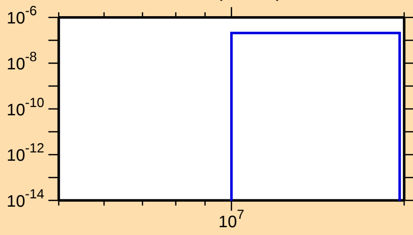
\sigma vs. E for ^{147}\text{Pm}(n,2n\alpha)
