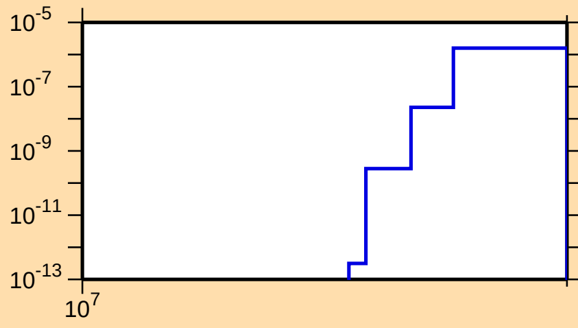
\sigma vs. E for ^{149}\text{Pm}(n,2np)
