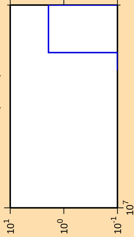
\Delta\sigma/\sigma vs. E for ^{149}\text{Pm}(\text{mt } 11)
