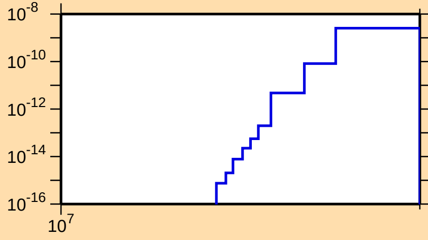
\sigma vs. E for ^{149}\text{Pm}(n,\text{He}3)
