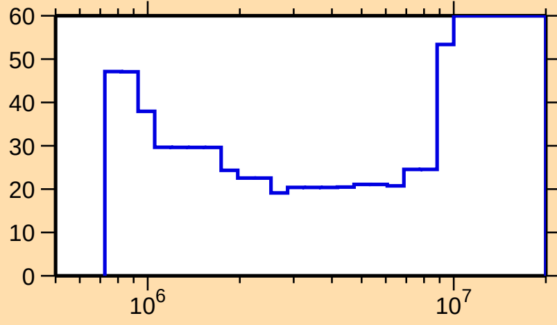
\Delta\sigma/\sigma vs. E for ^{149}\text{Pm}(n,n\text{cont.})
