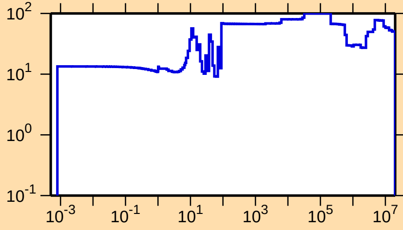
\Delta\sigma/\sigma vs. E for ^{149}\text{Pm}(n,\text{el.})
