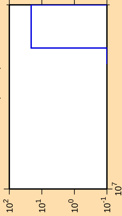
\Delta\sigma/\sigma vs. E for ^{149}\text{Pm}(n,3n\alpha)
