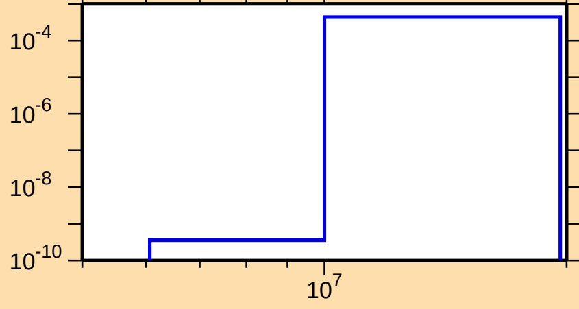
\sigma vs. E for ^{149}\text{Pm}(n,t)
