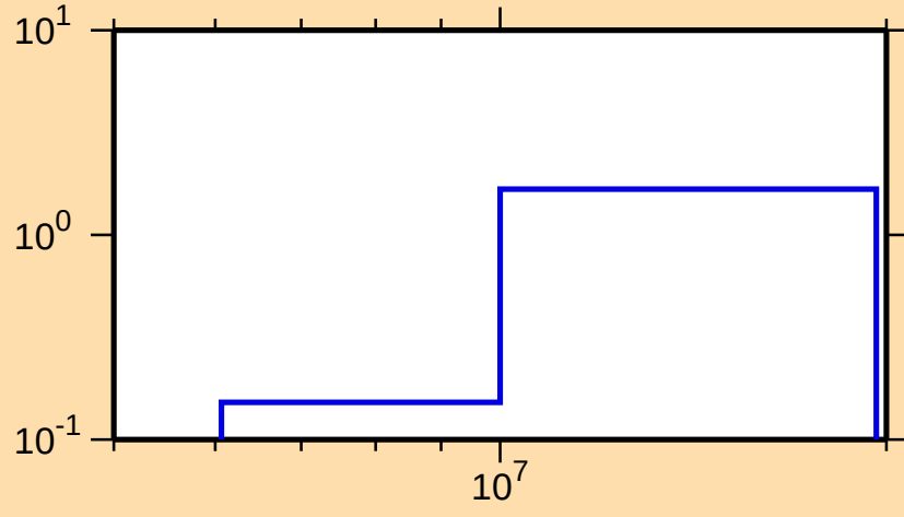
\sigma vs. E for ^{149}\text{Pm}(n,2n)
