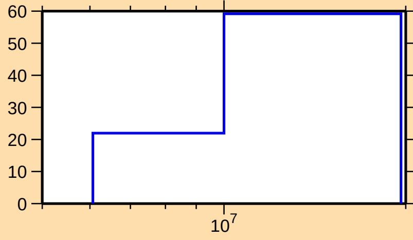
\Delta\sigma/\sigma vs. E for ^{149}\text{Pm}(n,\text{inel.})
