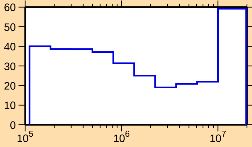
\Delta\sigma/\sigma vs. E for ^{149}\text{Pm}(n,\text{inel.})
