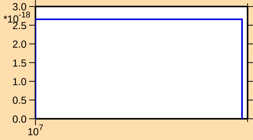
\sigma vs. E for ^{149}\text{Pm}(\text{mt } 42)
