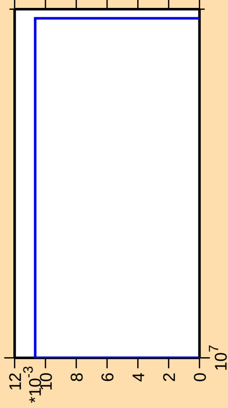
\Delta\sigma/\sigma vs. E for ^{149}\text{Pm}(\text{mt } 11)
