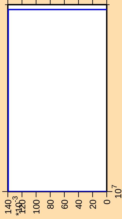
\Delta\sigma/\sigma vs. E for ^{149}\text{Pm}(n,3n\alpha)
