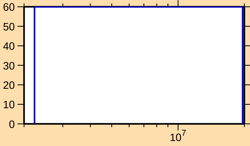
\Delta\sigma/\sigma vs. E for ^{149}\text{Pm}(n,n_1)
