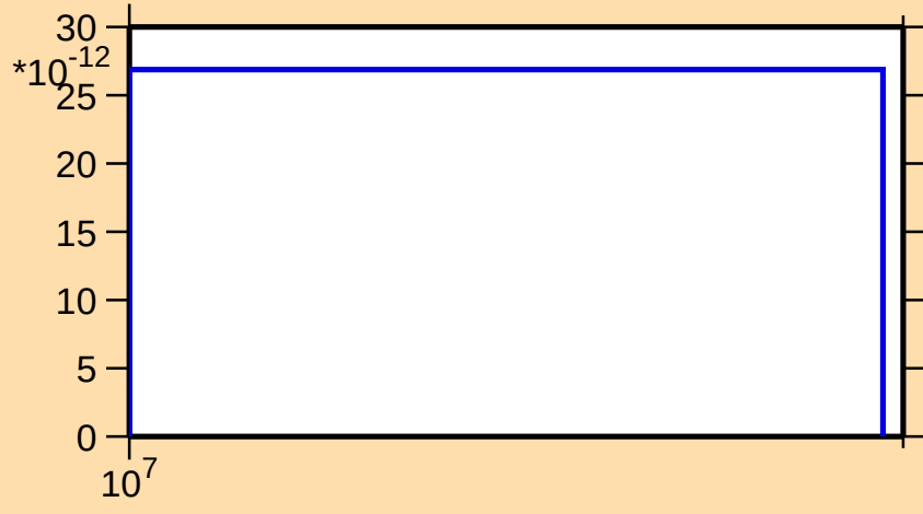
\sigma vs. E for ^{149}\text{Pm}(n,\text{He}3)
