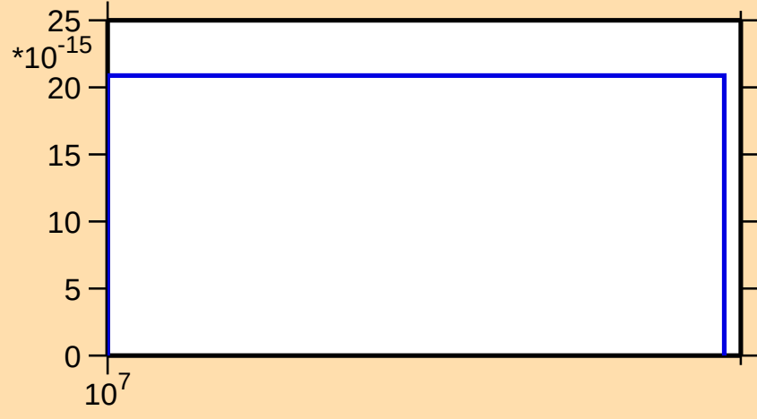
\sigma vs. E for ^{149}\text{Pm}(n,3n\alpha)
