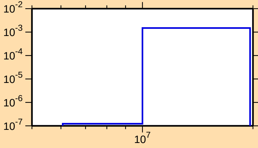
\sigma vs. E for ^{149}\text{Pm}(n,d)
