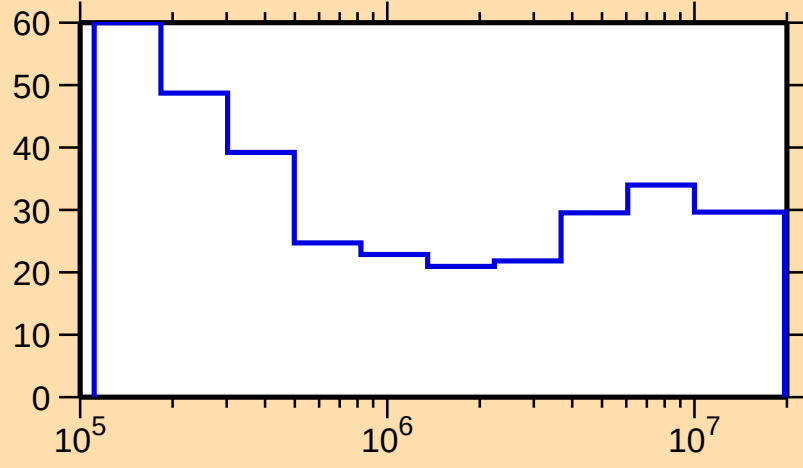
\Delta\sigma/\sigma vs. E for ^{149}\text{Pm}(n,\text{tot.})
