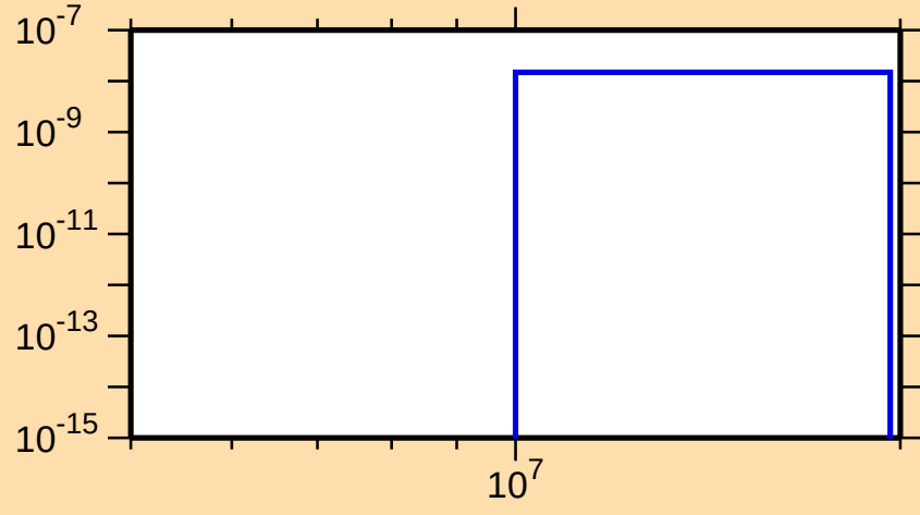
\sigma vs. E for ^{149}\text{Pm}(n,2n\alpha)
