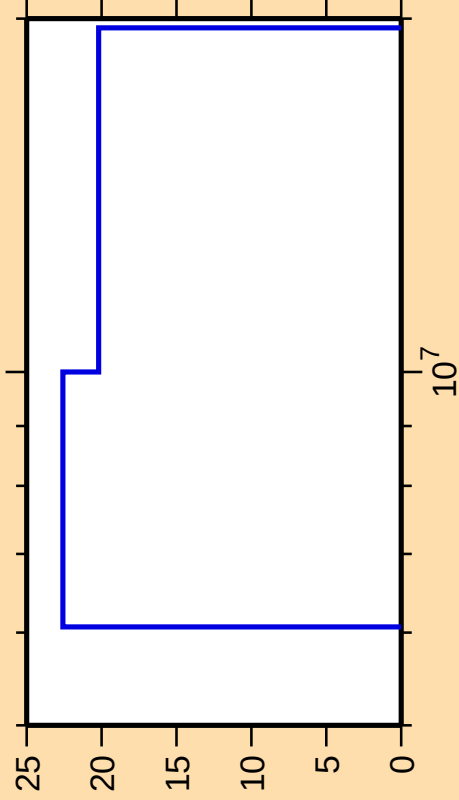
\Delta\sigma/\sigma vs. E for ^{149}\text{Pm}(n,2n)
