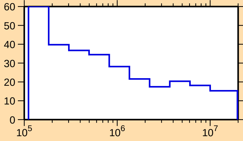
\Delta\sigma/\sigma vs. E for ^{149}\text{Pm}(n,\text{nonel.})
