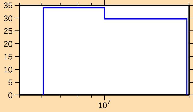
\Delta\sigma/\sigma vs. E for ^{149}\text{Pm}(n,\text{tot.})
