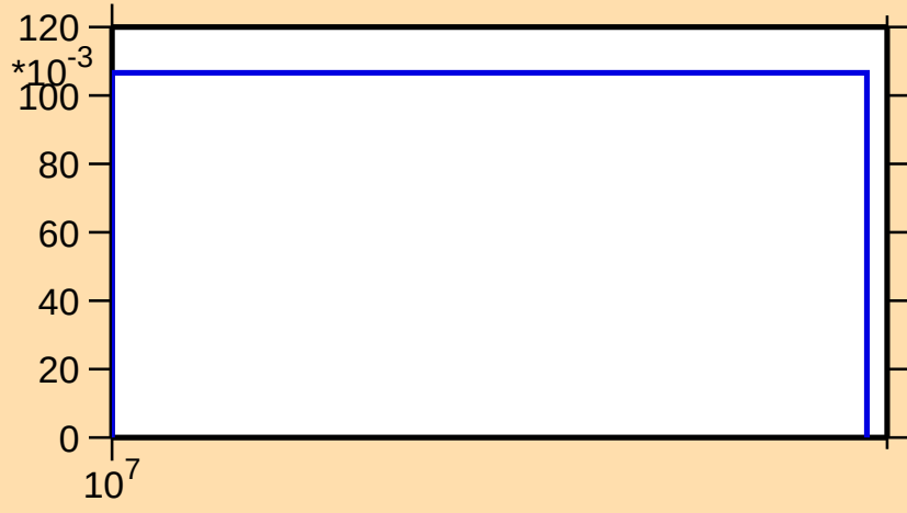
\sigma vs. E for ^{149}\text{Pm}(n,3n)
