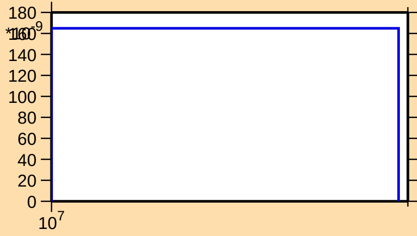
\sigma vs. E for ^{149}\text{Pm}(n,\text{nd})
