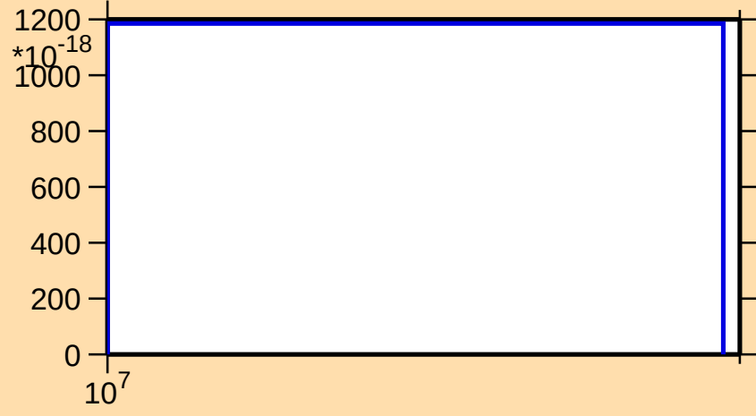
\sigma vs. E for ^{149}\text{Pm}(\text{mt } 11)
