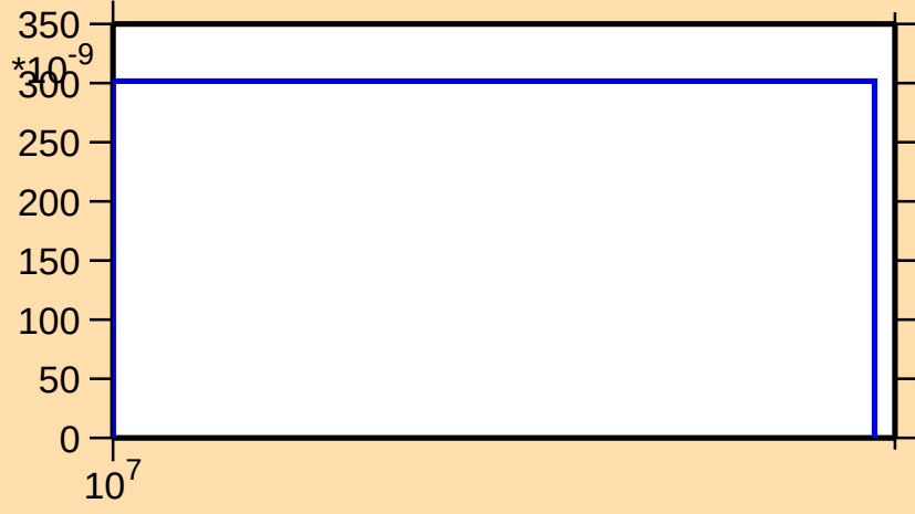
\sigma vs. E for ^{149}\text{Pm}(n,nt)
