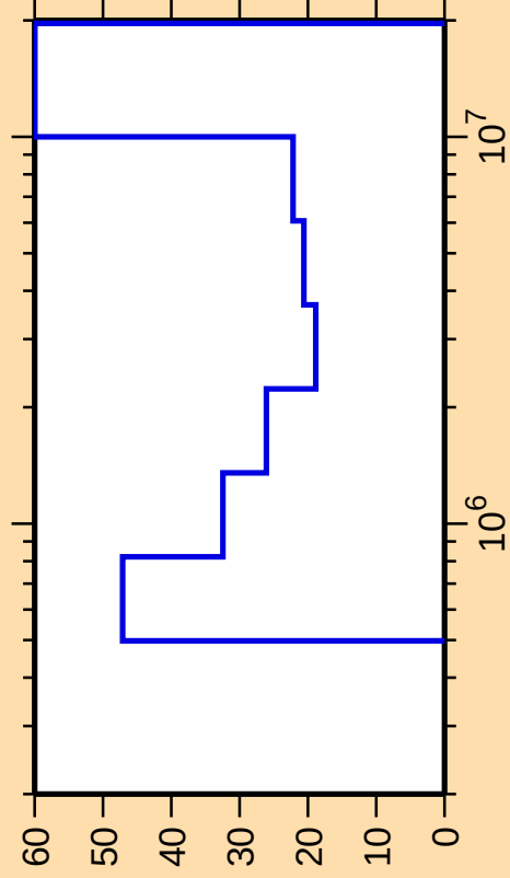
\Delta\sigma/\sigma vs. E for ^{149}\text{Pm}(n,n\text{cont.})
