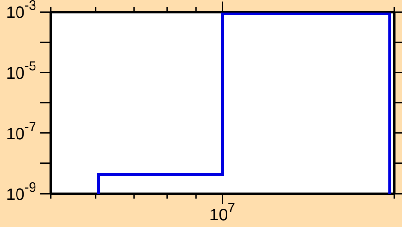
\sigma vs. E for ^{149}\text{Pm}(n,np)
