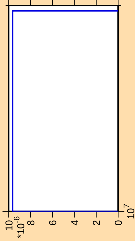
\Delta\sigma/\sigma vs. E for ^{149}\text{Pm}(\text{mt } 42)
