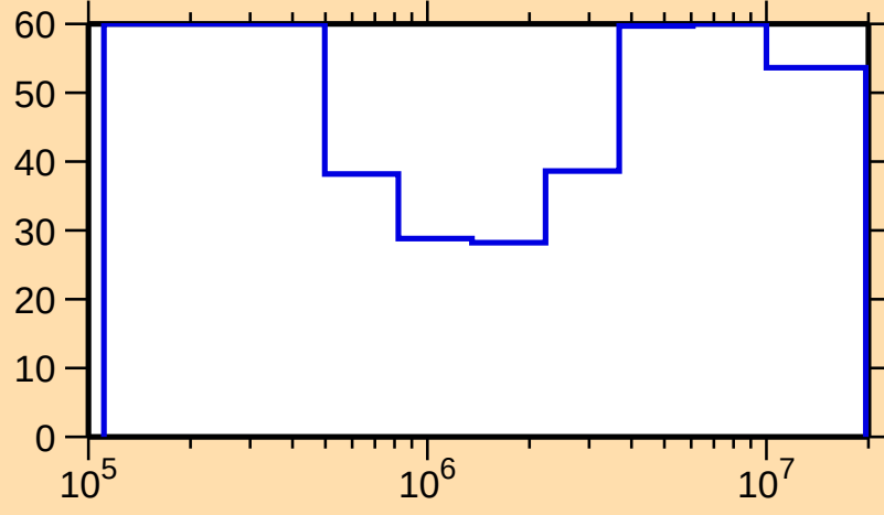
\Delta\sigma/\sigma vs. E for ^{149}\text{Pm}(n,\text{el.})
