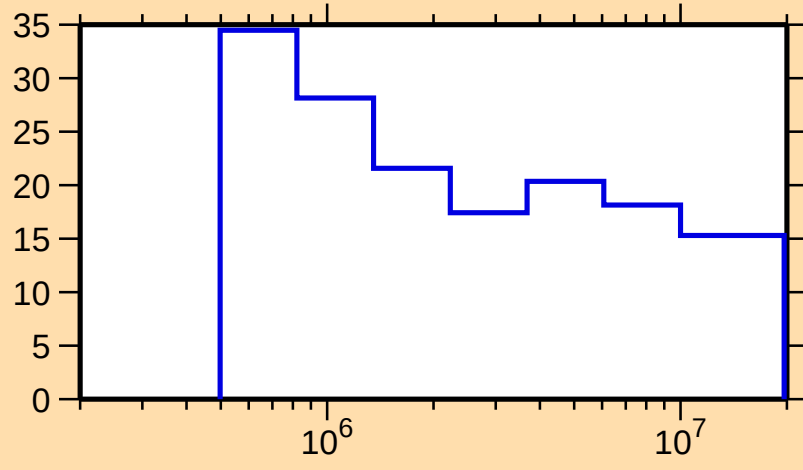
\Delta\sigma/\sigma vs. E for ^{149}\text{Pm}(n,\text{nonel.})
