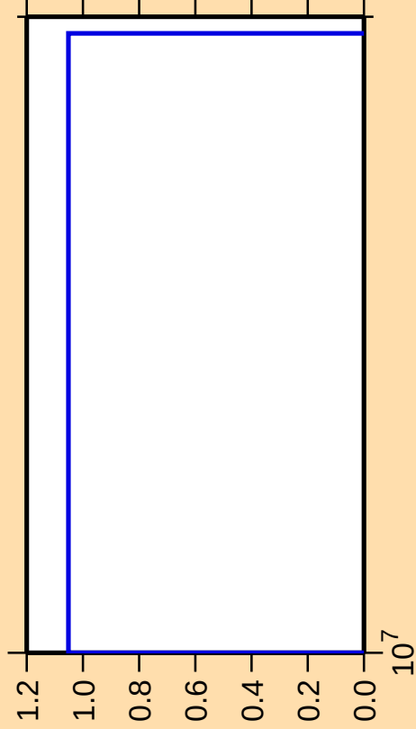
\Delta\sigma/\sigma vs. E for ^{149}\text{Pm}(n,p\alpha)
