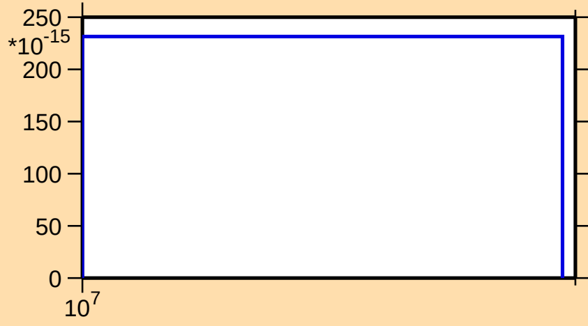
\sigma vs. E for ^{149}\text{Pm}(n,p\alpha)
