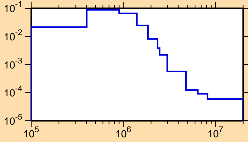
\sigma vs. E for ^{149}\text{Pm}(n,n_2)
