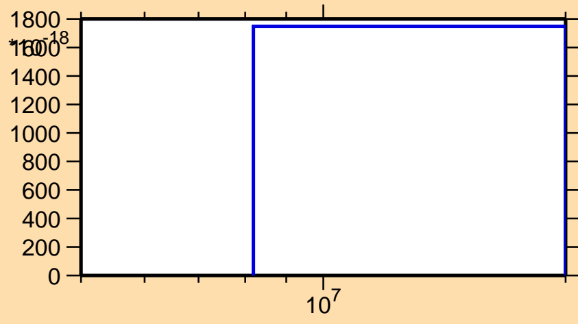
\sigma vs. E for ^{149}\text{Pm} (mt 11)
