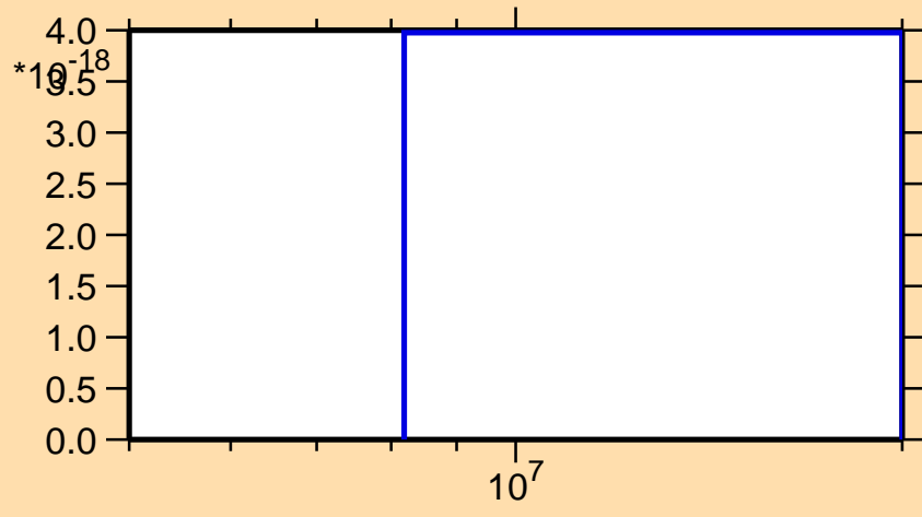
\sigma vs. E for ^{149}\text{Pm} (mt 42)
