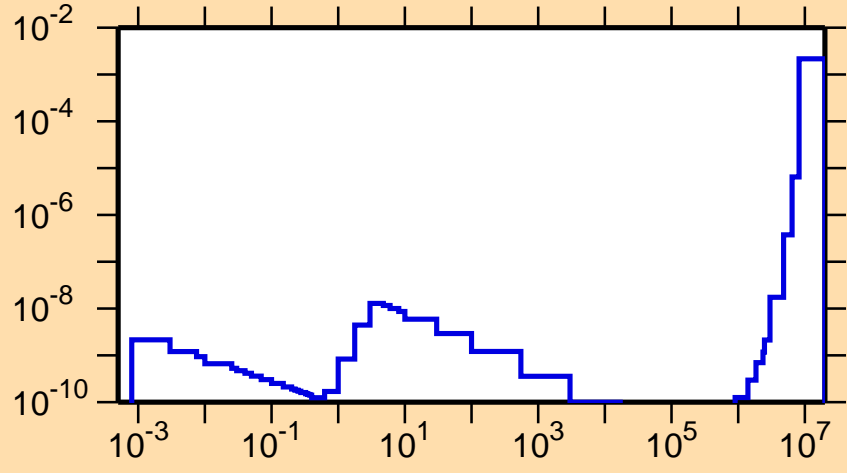
\sigma vs. E for ^{149}\text{Pm}(n,\alpha)
