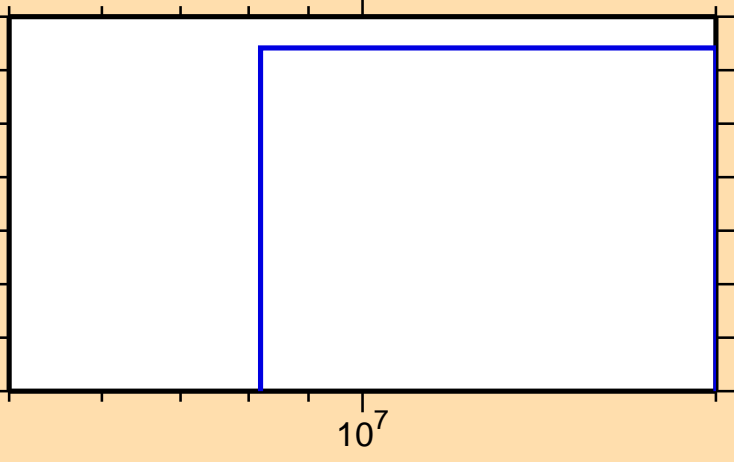
\sigma vs. E for ^{149}\text{Pm}(n,2n\alpha)
