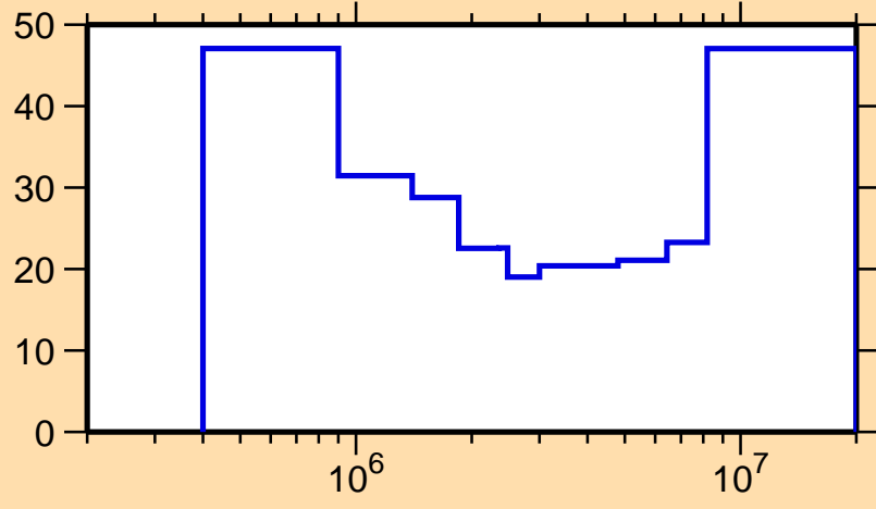
\Delta\sigma/\sigma vs. E for ^{149}\text{Pm}(n,n\text{cont.})
