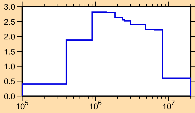
\sigma vs. E for ^{149}\text{Pm}(n,\text{inel.})
