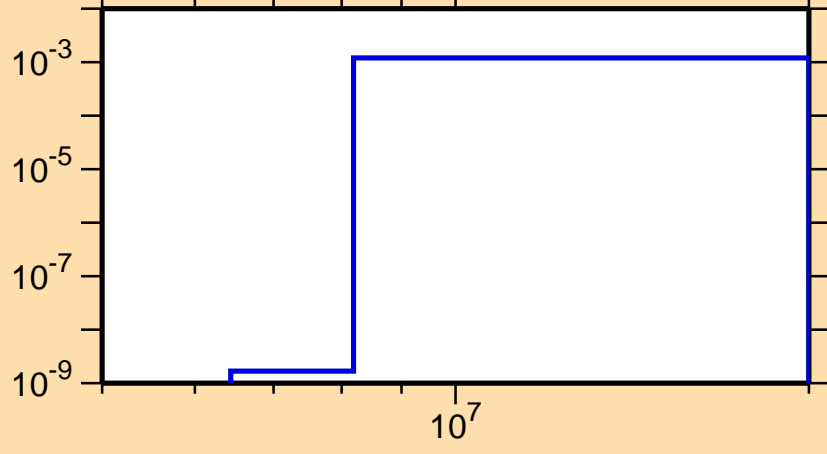
\sigma vs. E for ^{149}\text{Pm}(n,d)
