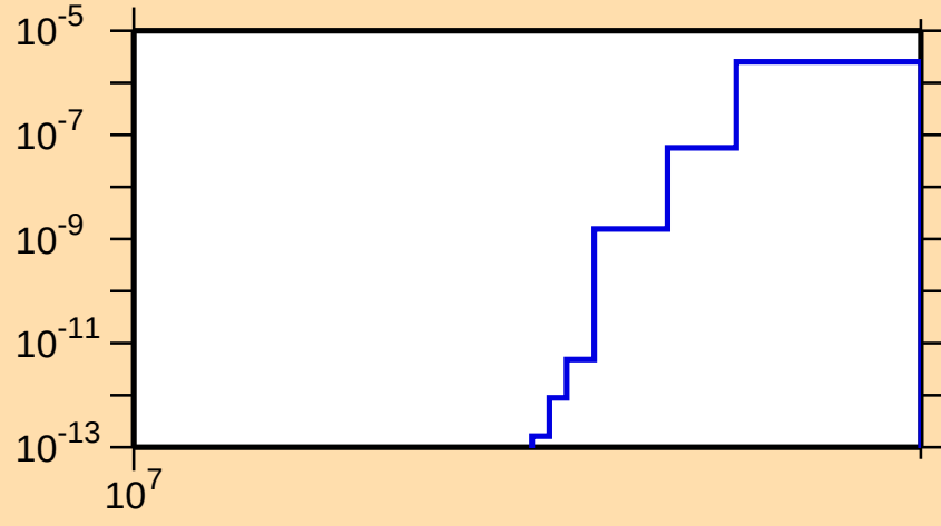
\sigma vs. E for ^{152}\text{Pm}(n,2np)
