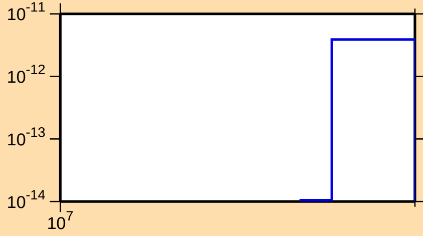
\sigma vs. E for ^{152}\text{Pm}(n,\text{He}3)
