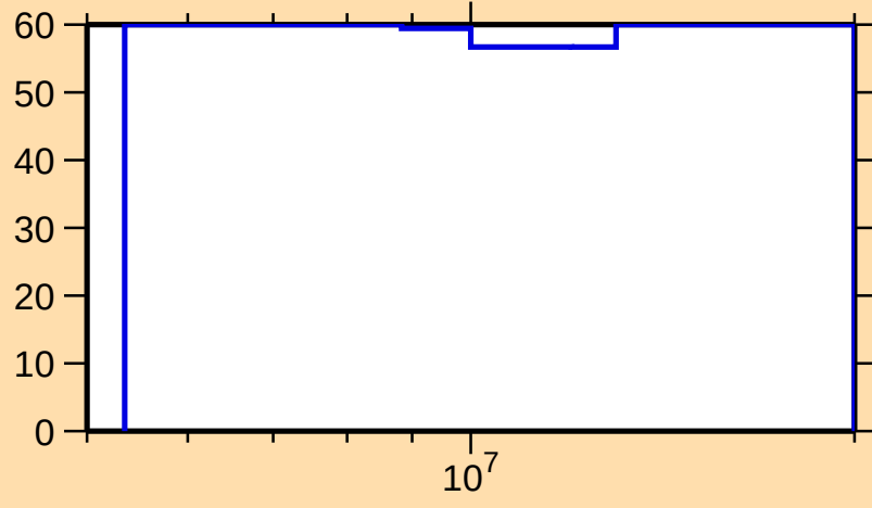
\Delta\sigma/\sigma vs. E for ^{152}\text{Pm}(n,2n)
