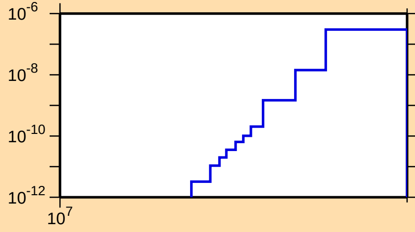
\sigma vs. E for ^{152}\text{Pm}(n,2n\alpha)
