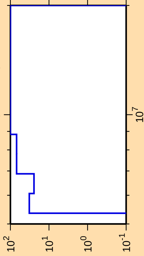
\Delta\sigma/\sigma vs. E for ^{152}\text{Pm}(n,n\text{cont.})
