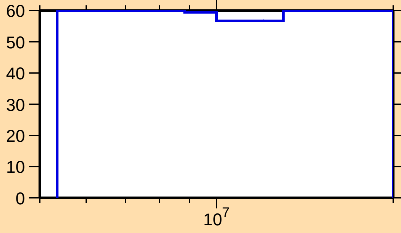
\Delta\sigma/\sigma vs. E for ^{152}\text{Pm}(n,2n)
