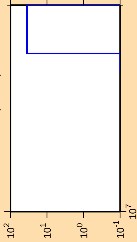
\Delta\sigma/\sigma vs. E for ^{152}\text{Pm}(n,\text{He}3)
