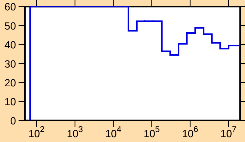
\Delta\sigma/\sigma vs. E for ^{152}\text{Pm}(n,\text{nonel.})
