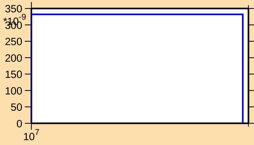
\sigma vs. E for ^{152}\text{Pm}(n,\text{nd})
