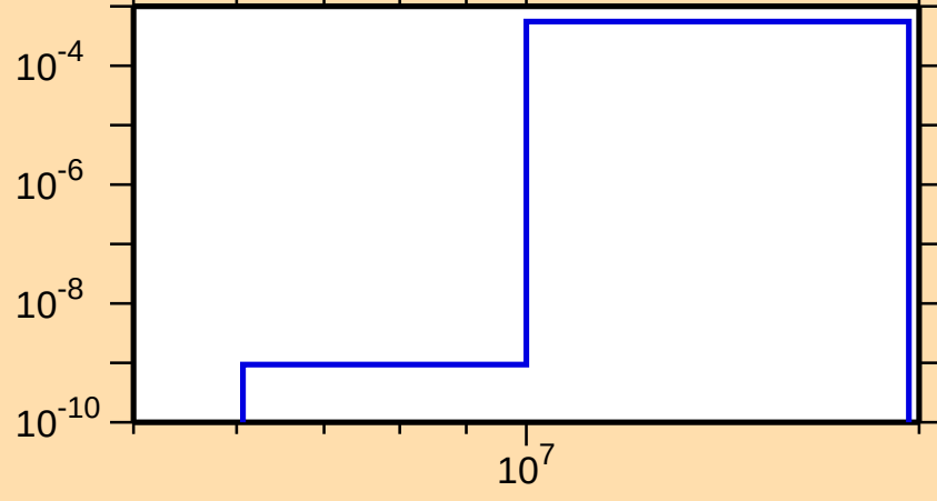
\sigma vs. E for ^{152}\text{Pm}(n,d)
