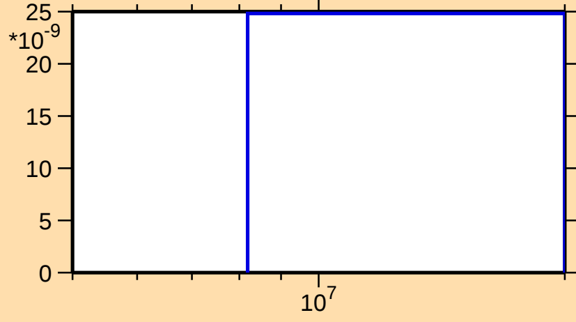
\sigma vs. E for ^{152}\text{Pm}(n,nt)
