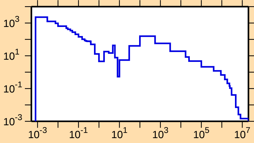
\sigma vs. E for ^{152}\text{Pm}(n,\gamma)
