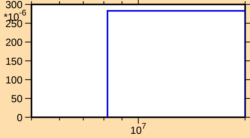
\sigma vs. E for ^{152}\text{Pm}(n,np)
