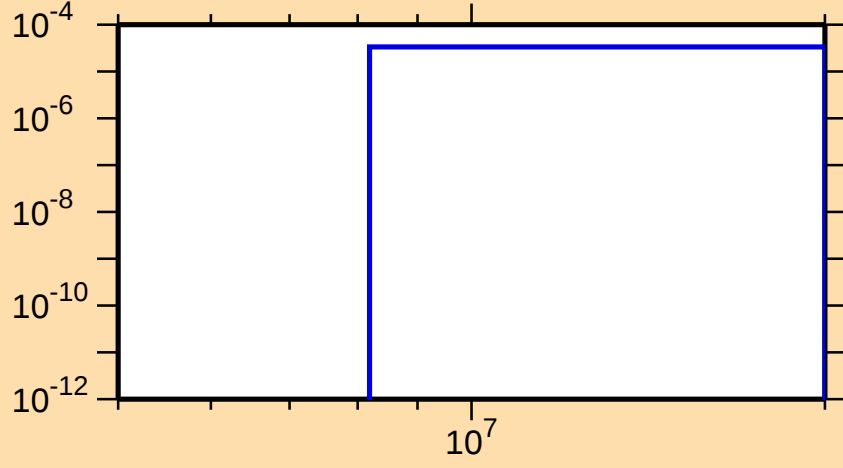
\sigma vs. E for ^{152}\text{Pm}(n,n\alpha)
