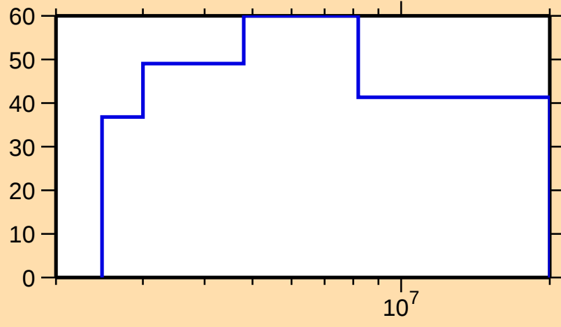
\Delta\sigma/\sigma vs. E for ^{152}\text{Pm}(n,\text{el.})
