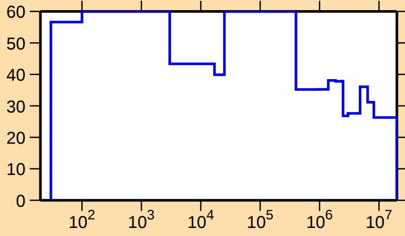
\Delta\sigma/\sigma vs. E for ^{152}\text{Pm}(n,\text{tot.})
