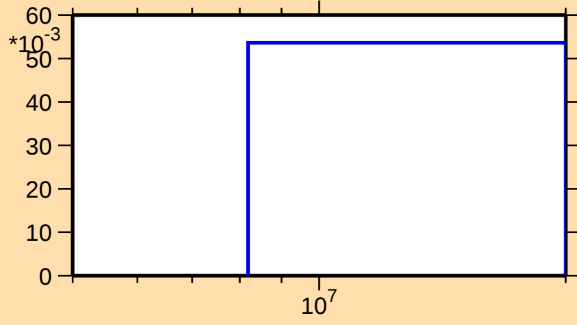
\sigma vs. E for ^{152}\text{Pm}(n,3n)
